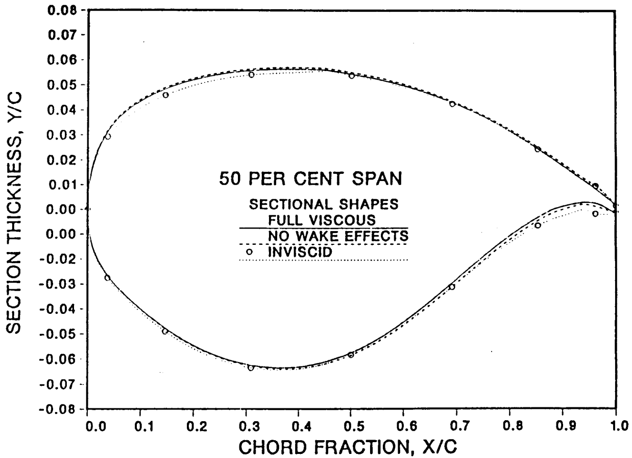
Figure 22. Comparison of sections designed at 50 percent span using different viscous interaction assumptions for Lockheed Wing 'A' wing body.
