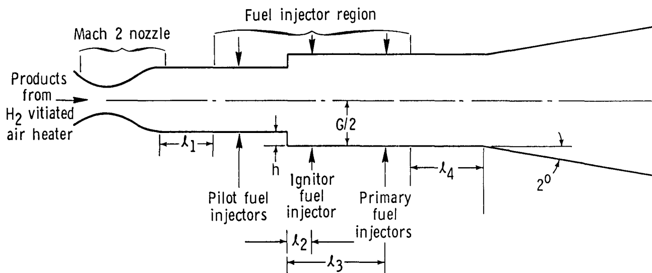
Fuel injector region (Top view)
