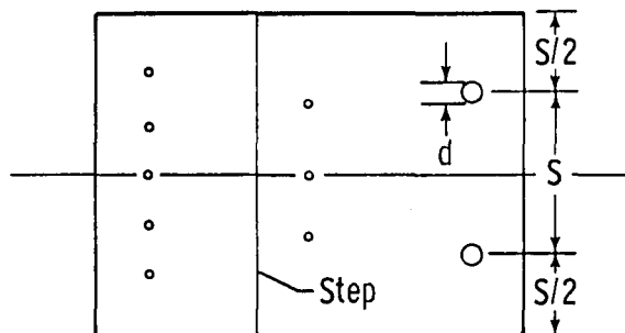
Fuel injector region (Top view)
