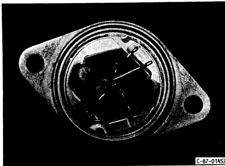
FIGURE 7. - HERMETIC, HIGH POWER SEMI-CONDUCTOR PACKAGE.
