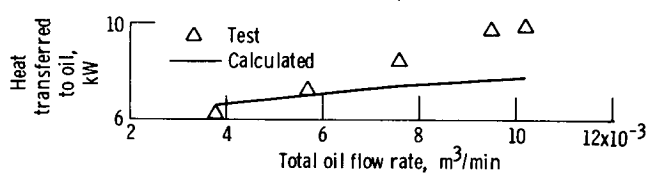
(b) Heat transferred to lubricating oil.
