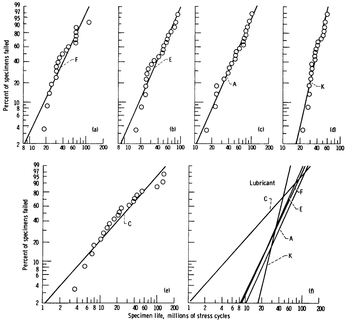
Figure 6. - Surface pitting fatigue life as affected by type of lubricant. Tests conducted on NASA Spur Gear Rig. Gear material - CVM AISI 9310, speed - 10 000 rpm, temperature - 350 K (170 °F), maximum Hertz stress - 1,7 MPa (248 000 psi). Lubricant types: A - Mobil ATF 220, C - Aeroshell 500, E - Syn Tech NS677, F - Mobil RL714, K - Aeroshell 555.
