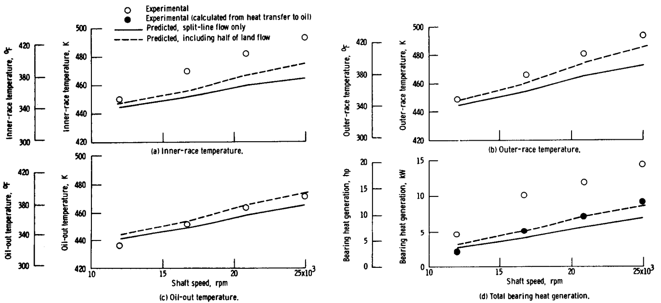
Figure 13. - Predicted and experimental thermal performance of 120 mm bore ball bearing as function of shaft speed. Thrust load, 22 240 N (5000 lb); oil-in temperature, 427 K (310 °F); total lubricant flow rate, 4740 cm 3 /min (1.253 gpm).
