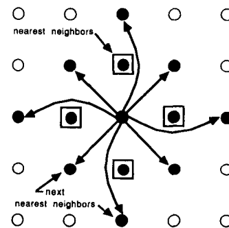
Figure 5 - Next Nearest Neighbor Connectivity
