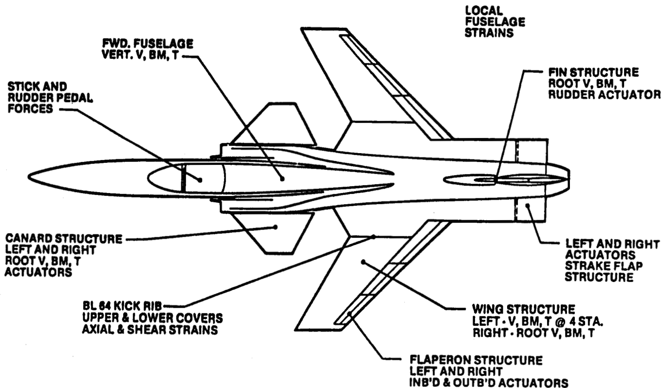
Figure 4. Structural loads instrumentation.
