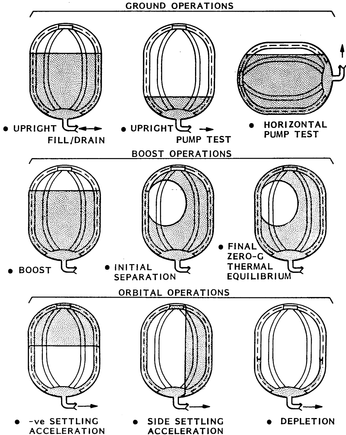
Fig. 4-2 Operational Sequence
