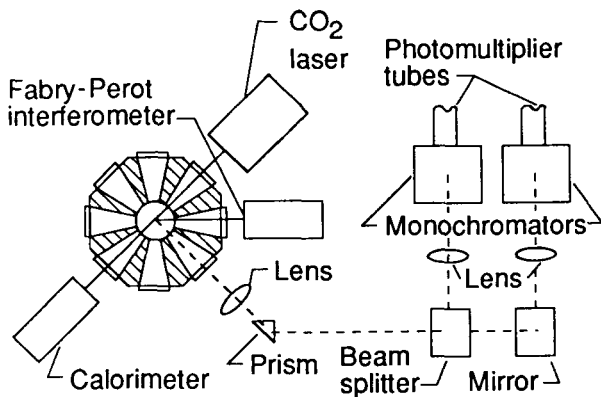
Figure 5. Laser-heated plasma.
