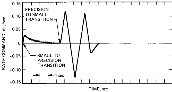
Fig. 3. Mode switching between Small Error and Precision modes (30-millidegree misalignment assumed)
