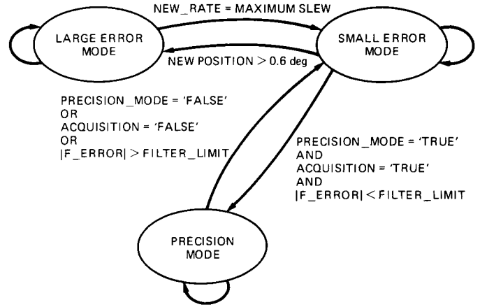
Fig. 4. New 70-m control mode switching logic
