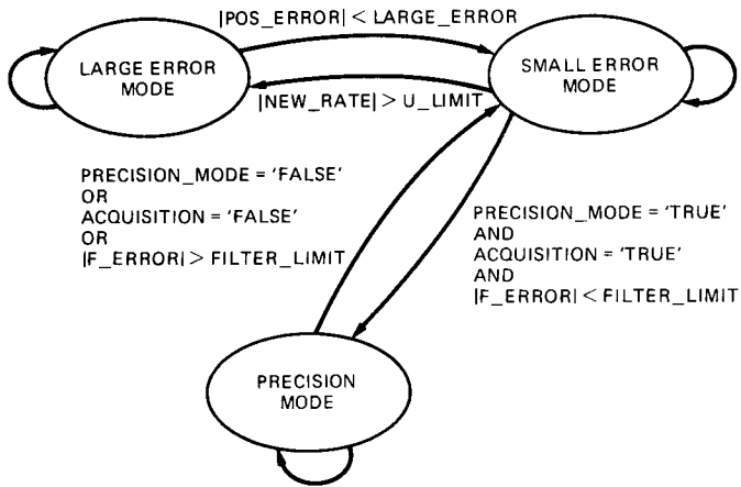
Fig. 1. Old control mode switching logic
