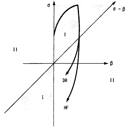
(A) STATE SPACE REPRESENTATION. LINE \sigma = \beta REPRESENTS THE ELASTIC DOMAIN GIVEN THAT Z(\Sigma_2/K) SINCE \epsilon^p = 0 THERE.
