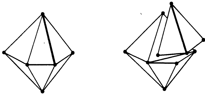
a) vertex removal
