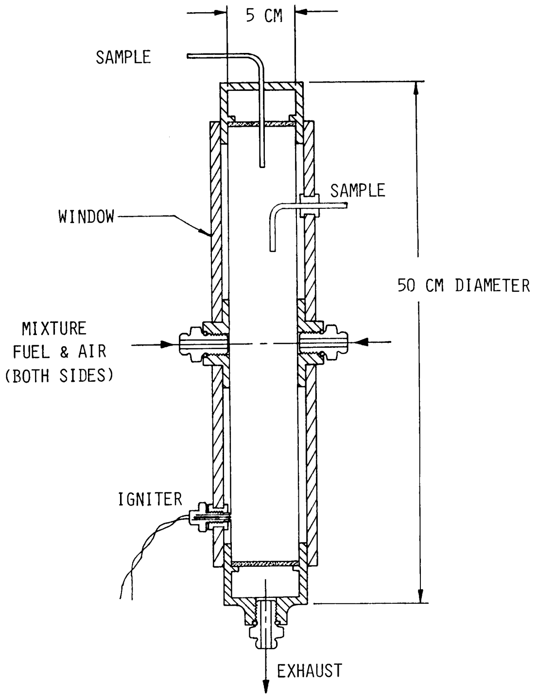
FIGURE 4b SCHEMATIC OF OPPOSED JET FUEL BURNER
