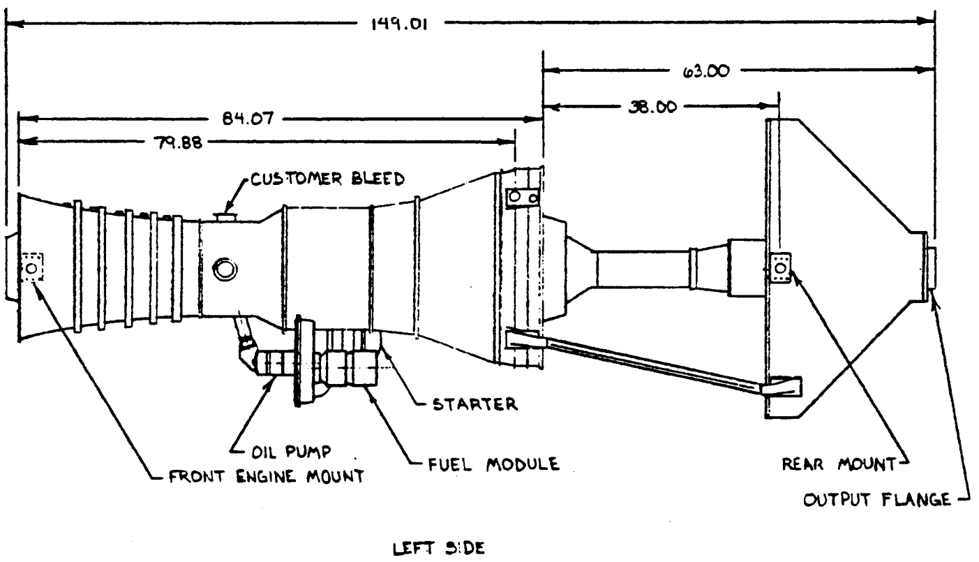
Figure 11. 11,000 shp PD436-11 Derivative Outline Drawing.
