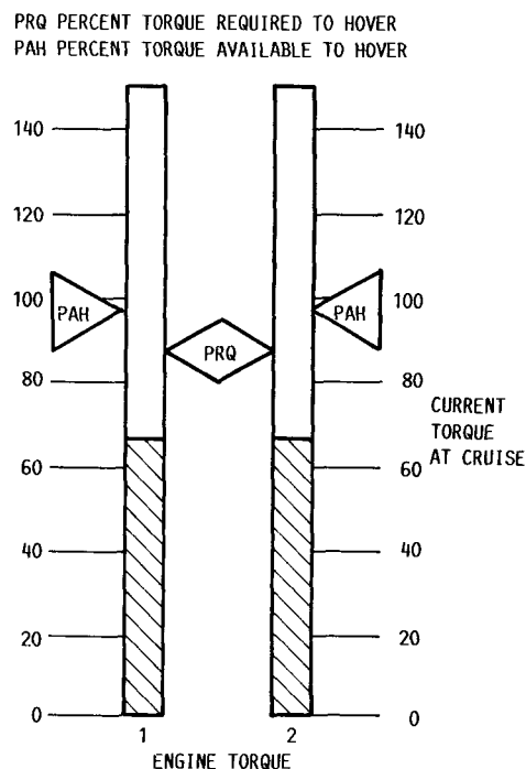
Figure 25.—Power available to hover indicator for dual-engine configuration.
