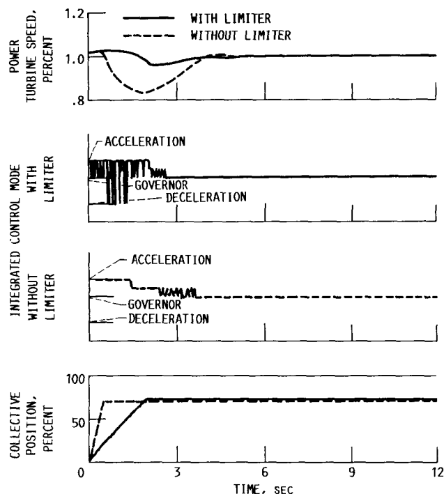
Figure 27.—Simulated autorotative recovery using collective-pitch-lever pull limiter on acceleration schedule.
