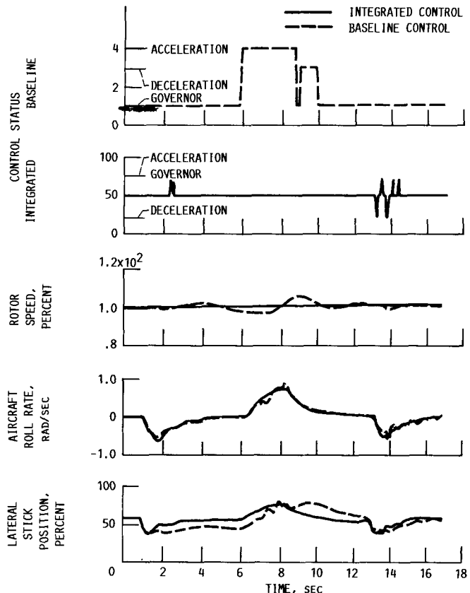
Figure 38.—Simulated roll-reversal maneuver; left-left-right.
