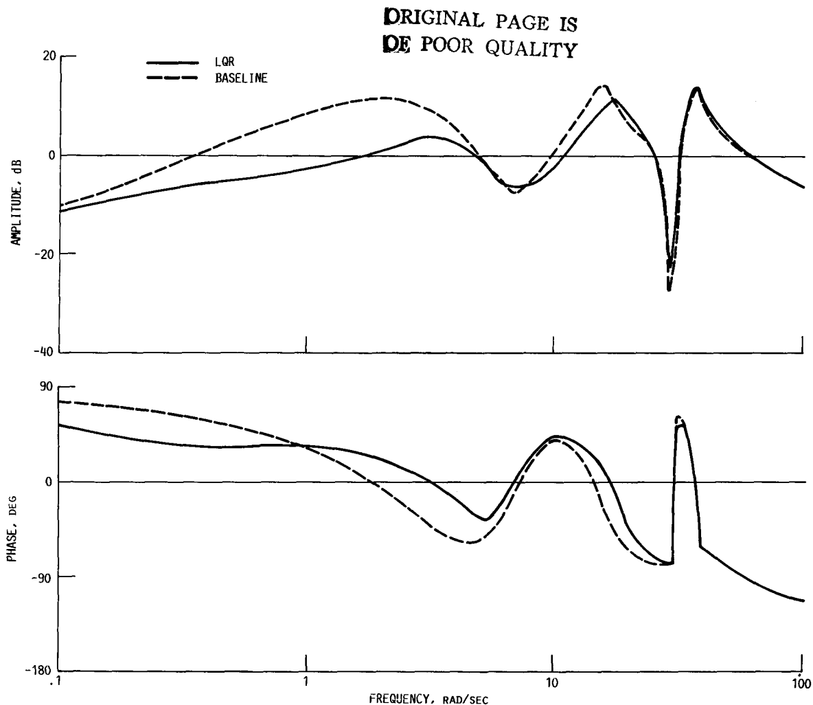
Figure 16.—Bode plot of baseline and linear-quadratic-regulator (LQR) power turbine speed response to main-rotor torque.
