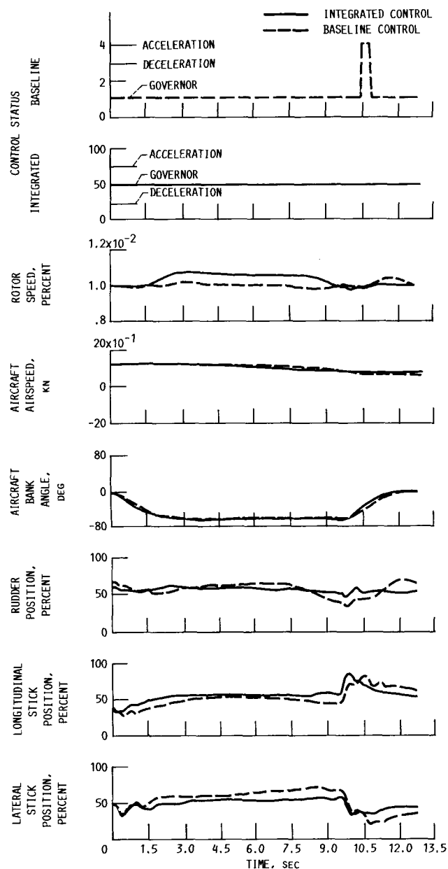
Figure 36.—High-g turn maneuver.
