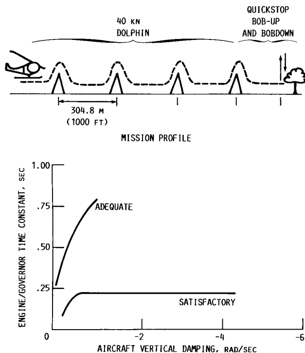
Figure 4.—Effect of engine response on handling qualities.
