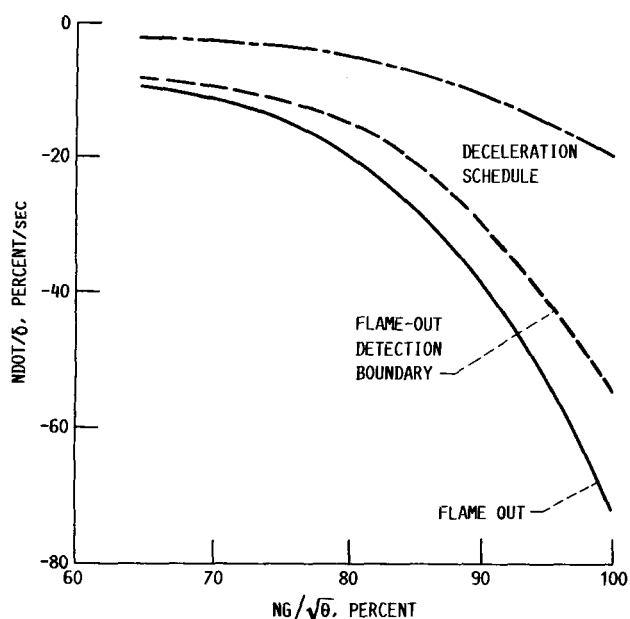
Figure 23.—Flame-out and normal engine deceleration rates.
