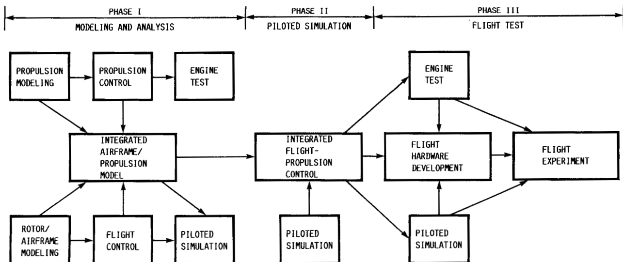
Figure 2.—Rotorcraft flight-propulsion control integration program.
