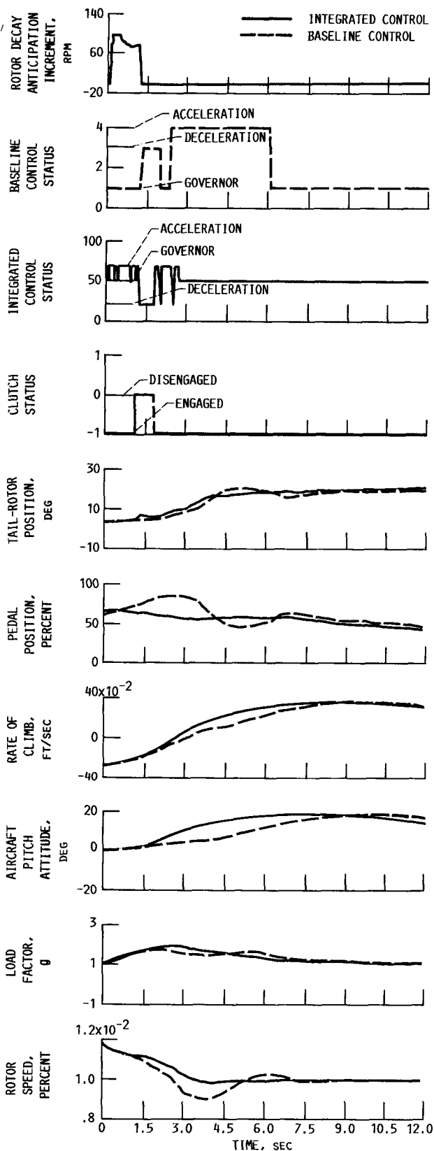
Figure 29.—Autorotational recovery from large speed split with slow collective pull.
