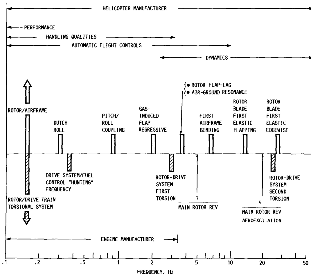
Figure 1.—Modal frequencies of interest in engine fuel control design and modeling.
