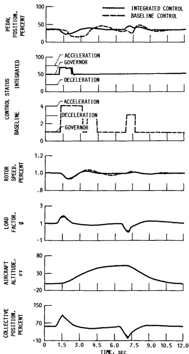
Figure 33.—Bob-up and remask maneuver.
