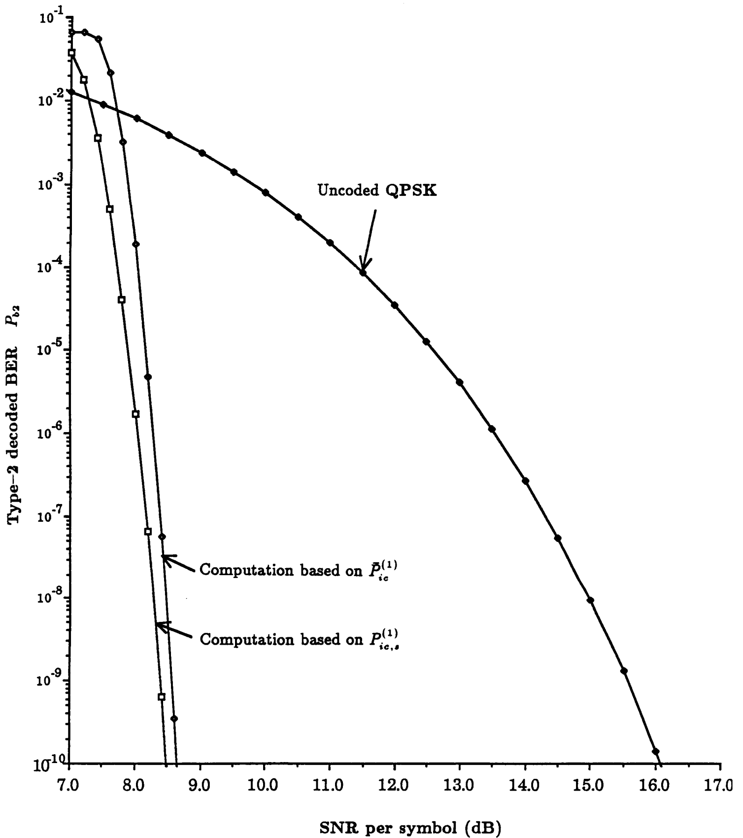
Figure 8 Type-2 bit error performance of the concatenated coded modulation scheme with the (255,223) RS outer code and the 4-state 8-PSK block inner code
