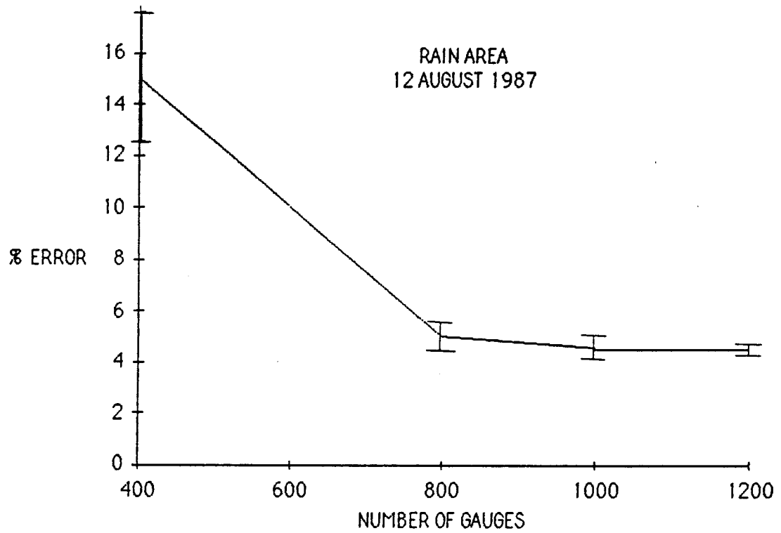
Figure 6. Mean and standard deviation of the error of the rain area estimate (12th August 1987).
