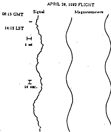
Figure 2 - Real Time Dipole Measurement.
