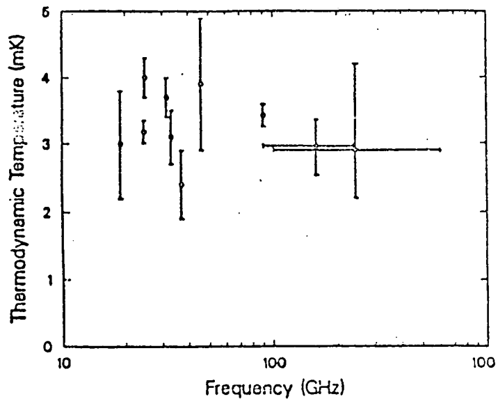
Figure 7 - Recent Dipole Anisotropy Measurements.
