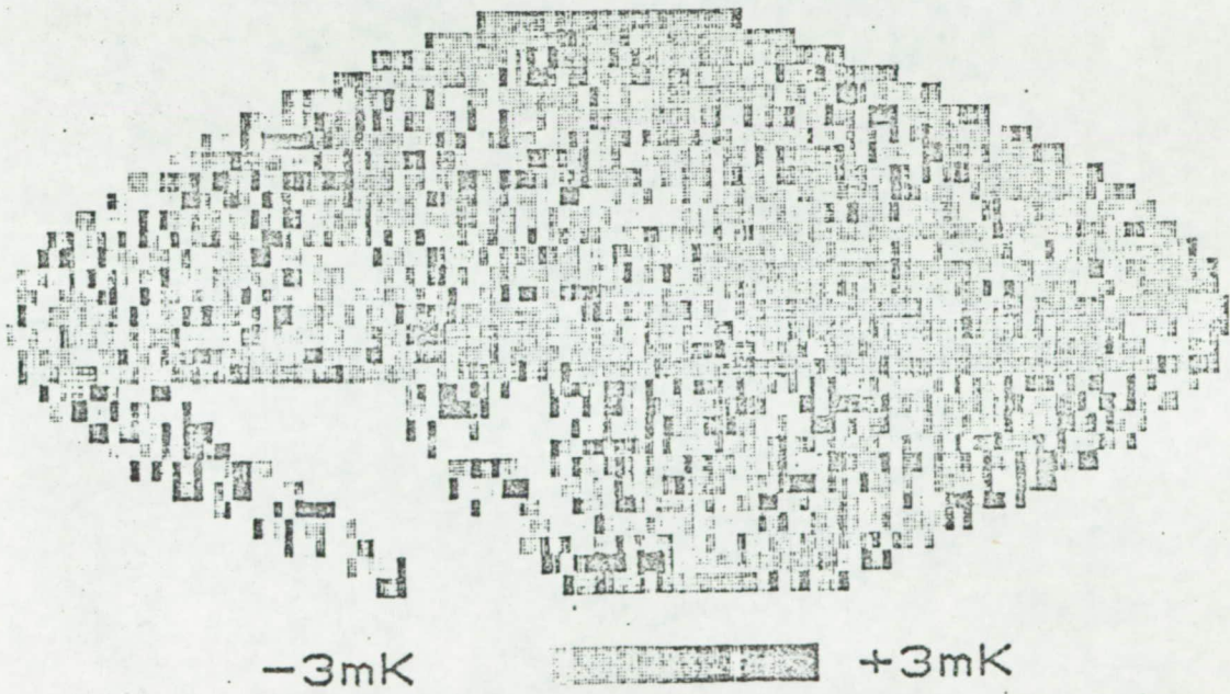
Figure 5 - Combined Residual Map.
