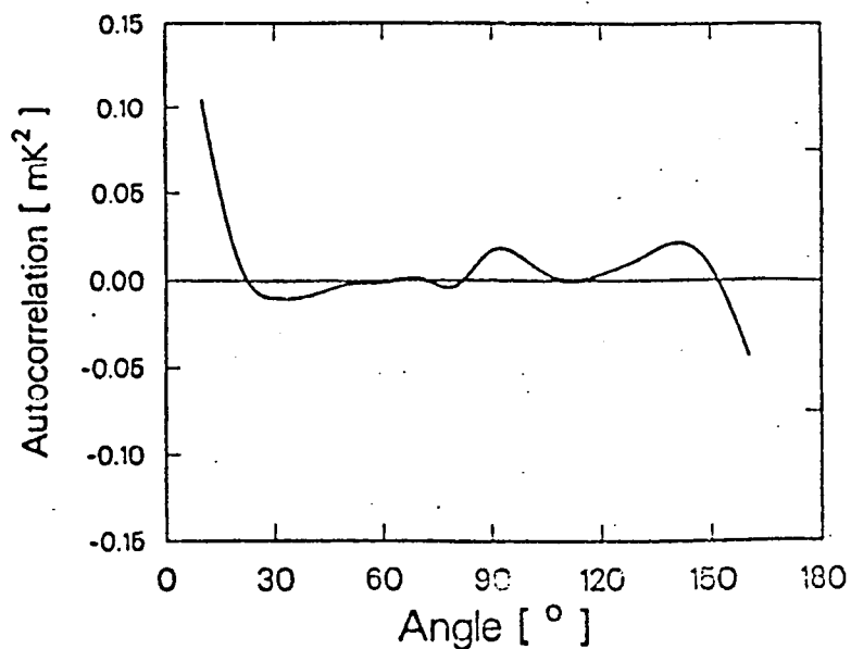
Figure 6 - Autocorrelation of the Combined Residual Map.
