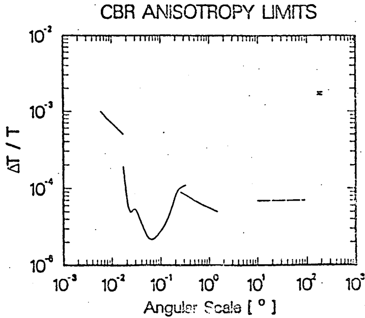
Figure 1 - Anisotropy Measurements at Various Angular Scales.
