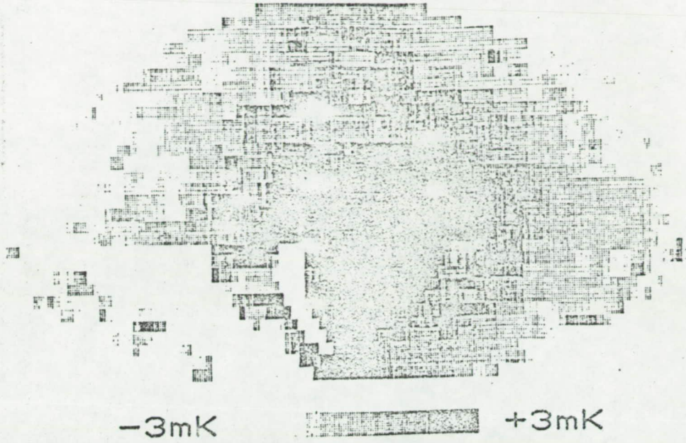
Figure 4 - Combined Dipole Map.
