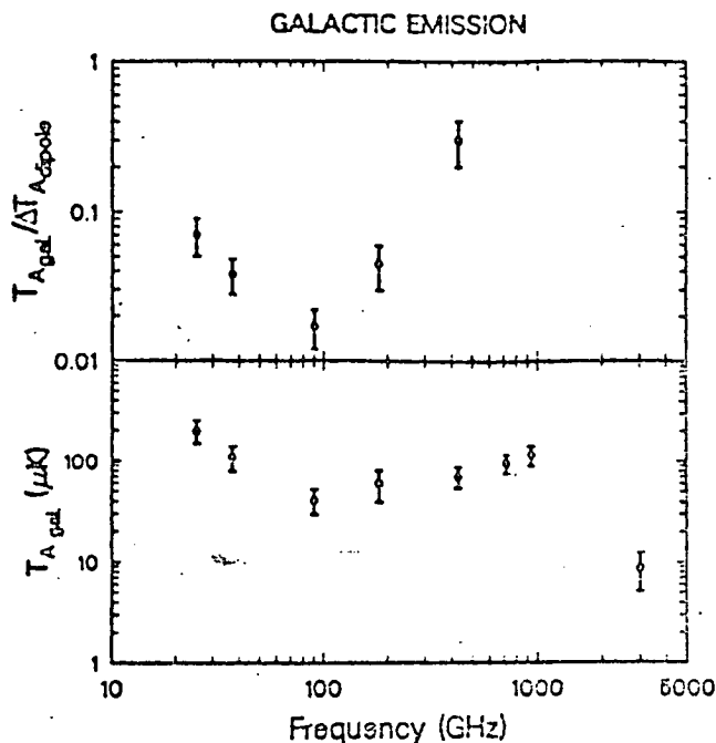
Figure 3 - Measured Galactic Emission Versus Frequency.
