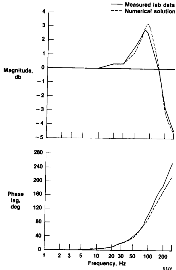
Fig. 5 Frequency response data: comparisons of lab to mathematical model for L = 24.5 in., D = 0.046 in., and altitude = 20,000 ft.
