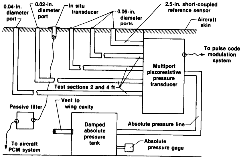
Fig. 6 Experimental configuration used for flight tests.
