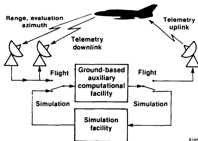
Fig. 1 Remotely augmented vehicle concept.
