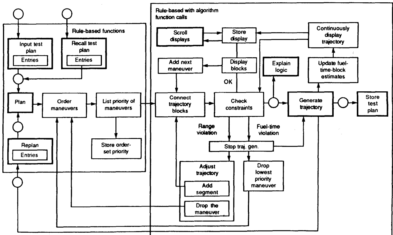
Fig. 6 Functional flow diagram of the flight test planning expert system.
