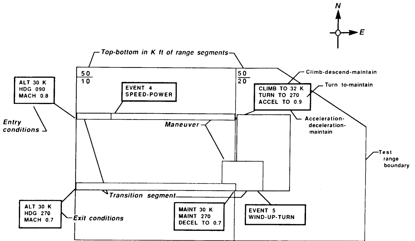
Fig. 8 Trajectory planning display.
