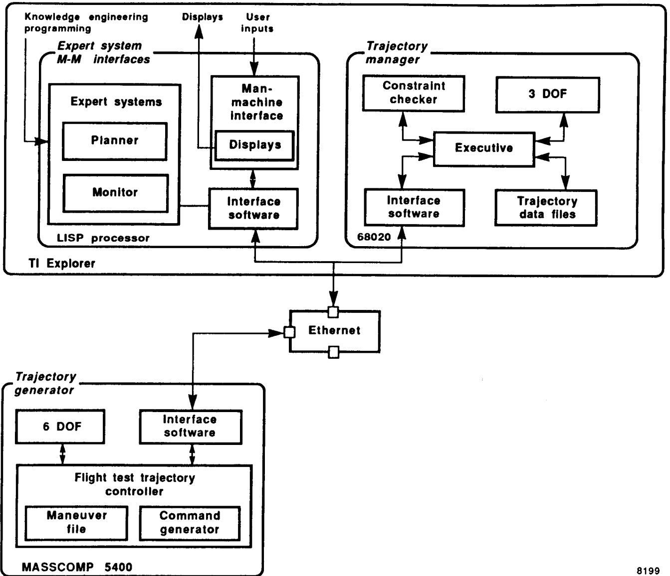
Fig. 15 System configuration for FTE workstation.
