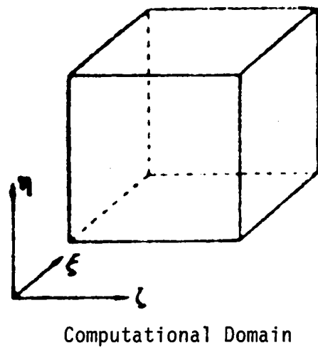
Fig. 4.1. Physical vs. Computational Domain.
