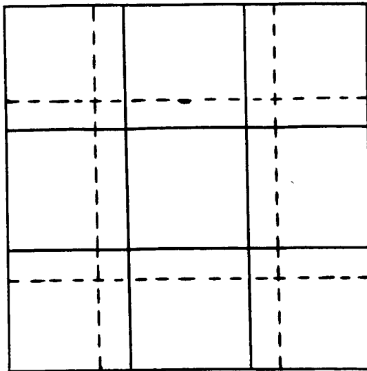
Fig. 2.1(a). Overlapped Grids
