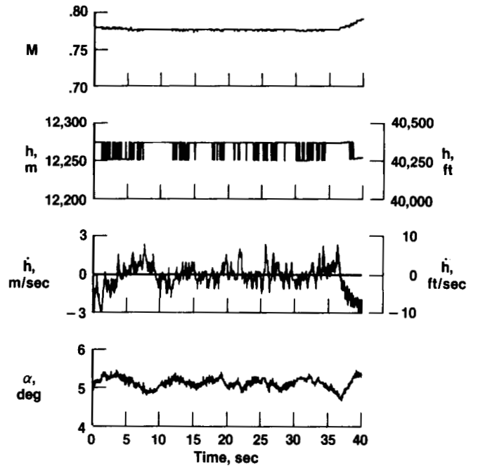
Figure 9. FTMAP constant-altitude, constant-Mach cruise at nominal conditions of Mach 0.80 and 12,200-m (40,000-ft) altitude.
