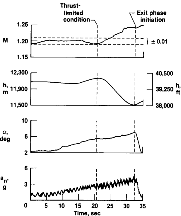
Figure 22. FTMAP supersonic thrust-limited windup turn at nominal conditions of Mach 1.20 and 12,200-m (40,000-ft) altitude.
