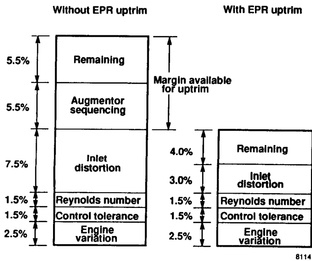
Fig. 4 Stall margin available.
