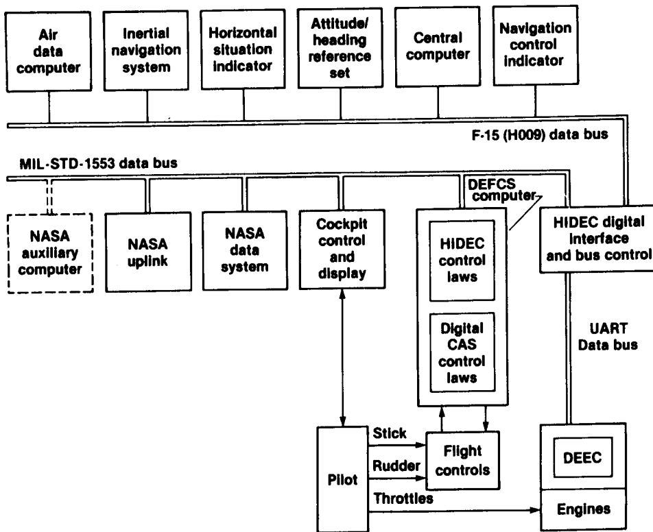
Fig. 2 Block diagram of the HIDEC system.
