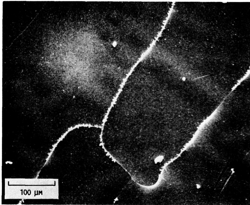
FIGURE 2. - EXAMPLE OF CRACKING OBSERVED ON SAMPLES WITH THICKER (4700 Å) \text{SiO}_2 COATINGS. PROTRUSION OF SILVER OXIDE THROUGH CRACKS IS EVIDENT. RF PLASMA EXPOSURE TIME WAS 190 HR.
