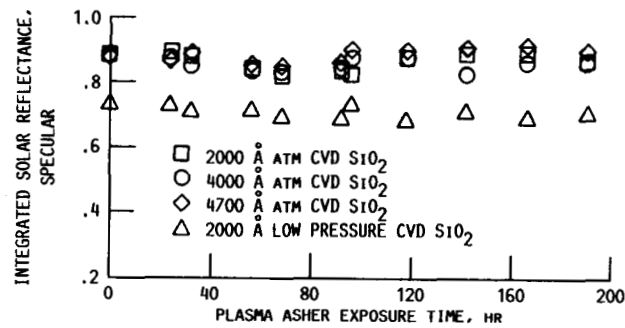
FIGURE 1. - SOLAR SPECULAR REFLECTANCE VERSUS OXYGEN PLASMA EXPOSURE TIME FOR THE REFLECTOR SAMPLES (VARIOUS THICKNESSES OF SiO 2 ON 1800 Å OF SILVER ON NICKEL SUBSTRATES) PREPARED IN THIS STUDY.
