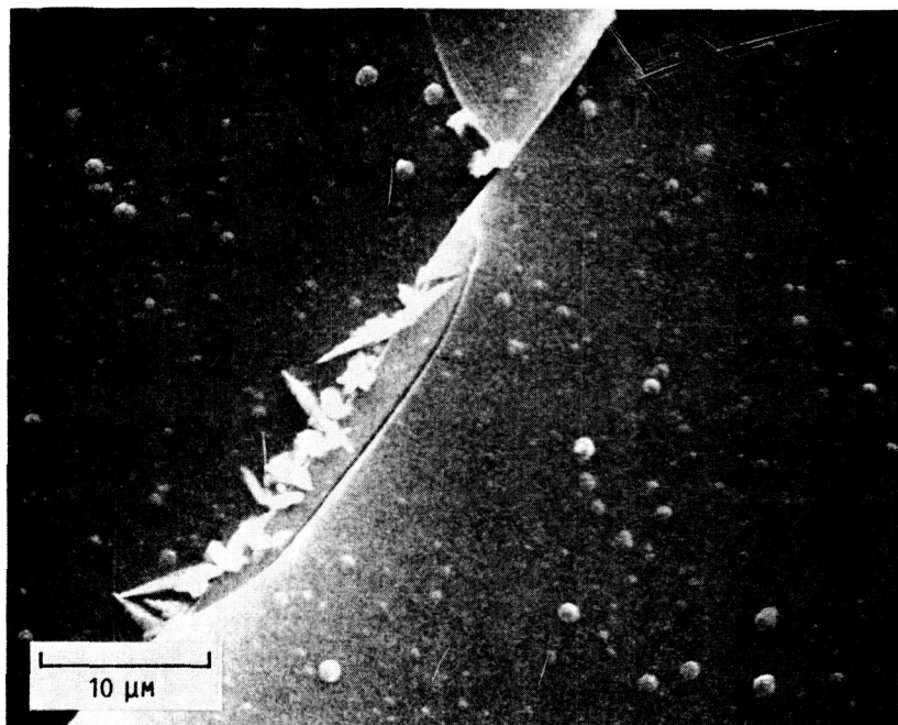
FIGURE 3. - DIFFERENT REGION OF SAME SAMPLE SHOWN IN FIG. 2, BUT AT HIGHER MAGNIFICATION. MULTIPLE FRACTURES ALONG THE CRACK INDICATE STRESS DUE TO DIFFERENT COEFFICIENTS OF THERMAL EXPANSION BETWEEN THE SUBSTRATE AND COATING.
