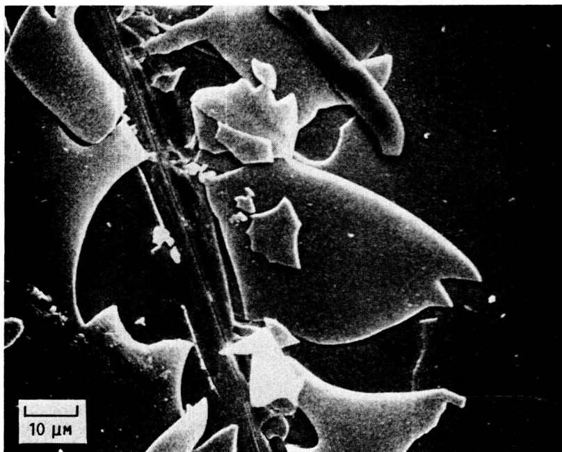
FIGURE 4. - AN EXAMPLE OF A CRACK WHICH DID NOT PENETRATE THROUGH TO THE SILVER LAYER, AS EVIDENCED BY ABSENCE OF SILVER OXIDE. \text{SiO}_2 COATING WAS 4000 Å THICK. RF PLASMA EXPOSURE TIME WAS 190 HR.
