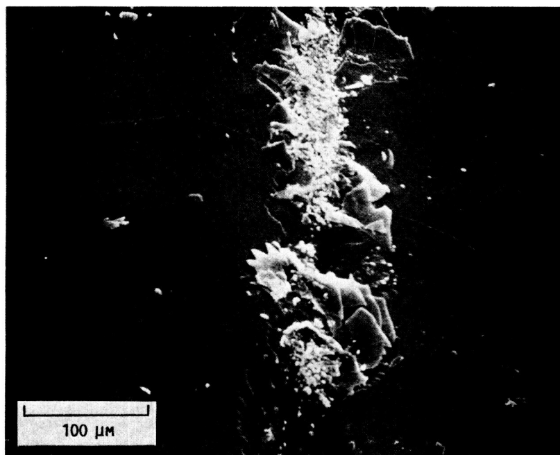
FIGURE 5. - DIFFERENT REGION OF SAME SAMPLE SHOWN IN FIG. 4 SHOWING A CRACK WHICH DID PENETRATE THROUGH TO SILVER LAYER.
