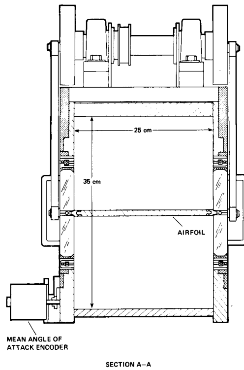
Fig. 4. Upstream view.
