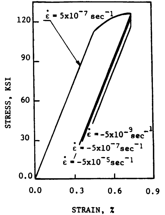
Fig. 11. Predicted load-unload response at different unloading strain rates.
