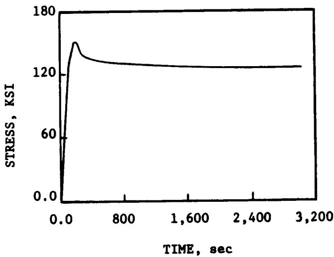
Fig. 10. Predicted relaxation response at \epsilon = 1\%
