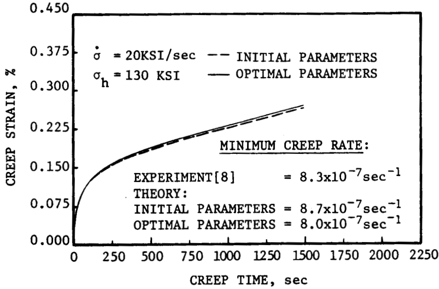
Fig. 3. Predicted creep response at \sigma_h = 130 \text{ KSI} ; only experimental steady state is available.
