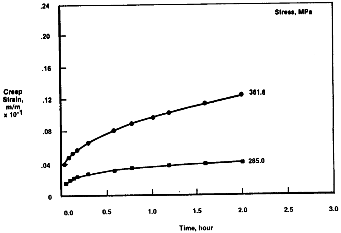
Figure 2a. - Creep Data and Curve Fits at 871 o C
