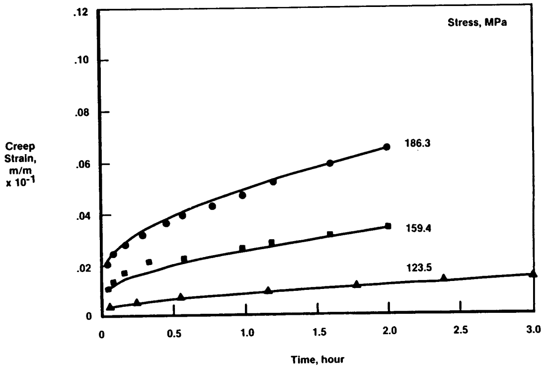
Figure 2b. - Creep Data and Curve Fits at 982 o C
