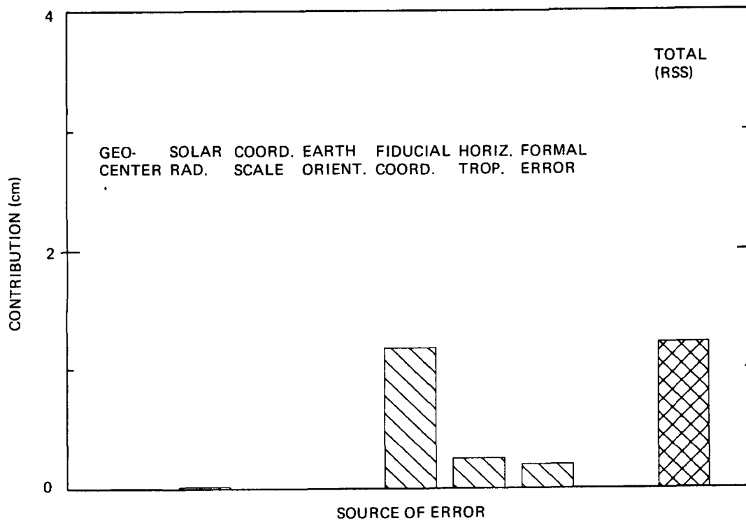
Figure 13. The total error budget for the north component of the 245 km OVRO/Mojave baseline between the SERIES-X receivers is shown. This error budget includes the contributions from all significant error sources, including consider errors, modeling errors in estimated parameters, and random, or formal, errors.
