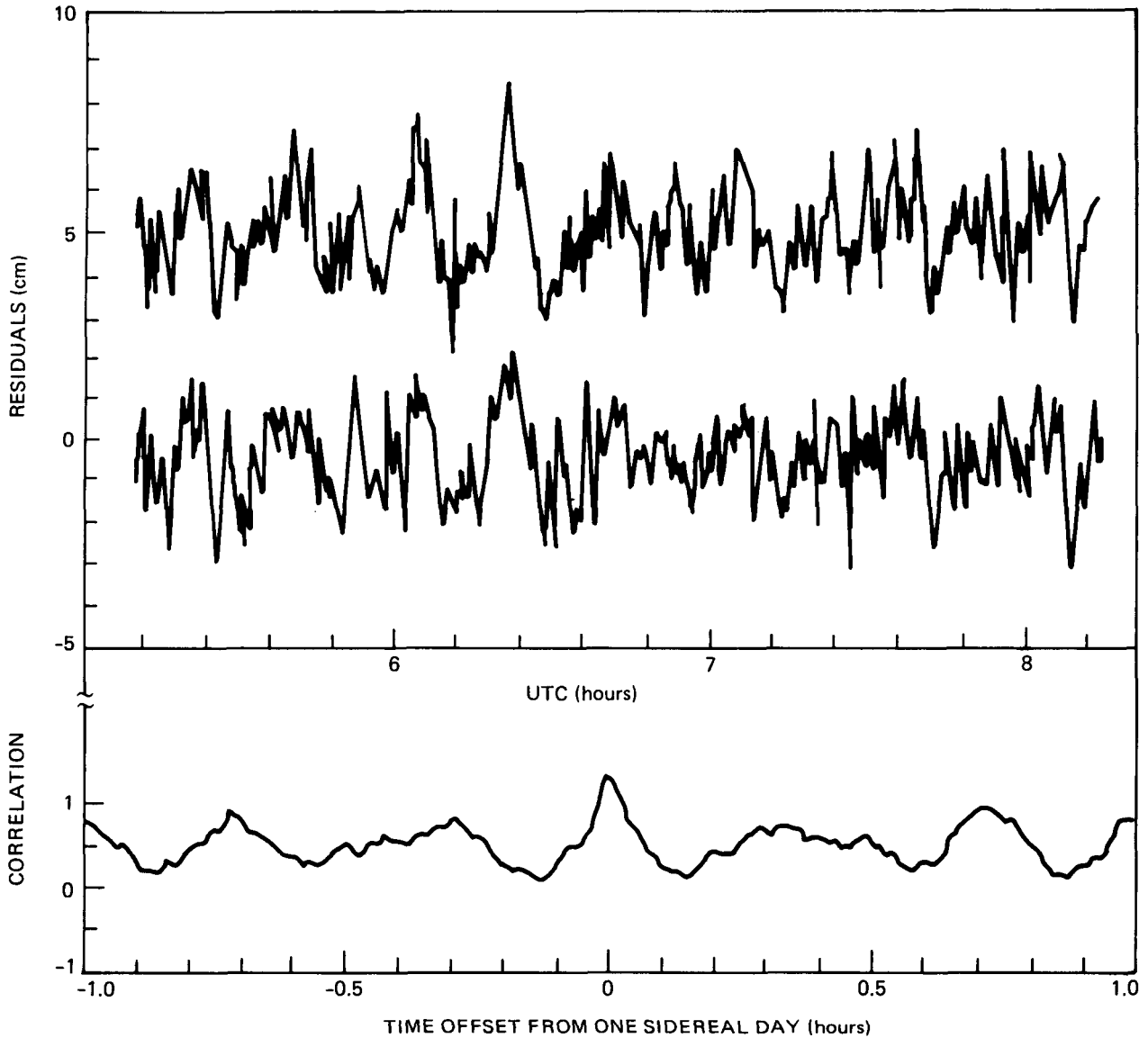
Figure 8. Post-fit residuals and cross-correlations for the TI-4100 carrier phase data of April 3 and 4, 1985, are shown. These data have been meteorologically and ionosphericly calibrated, double-differenced (GPS 6 and GPS 8 transmitters, Mojave and OVRO receivers), and fitted to a tenth-order polynomial. Multipath error will be periodic on a sidereal day, resulting in correlation between the upper and lower plots. The high correlation for an offset of exactly one sidereal day indicates substantial multipathing error for the TI-4100 antenna.
