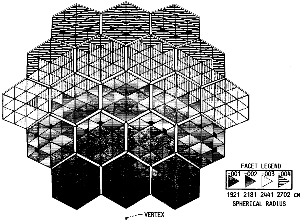
FIGURE 2. - OFFSET COLLECTOR.
