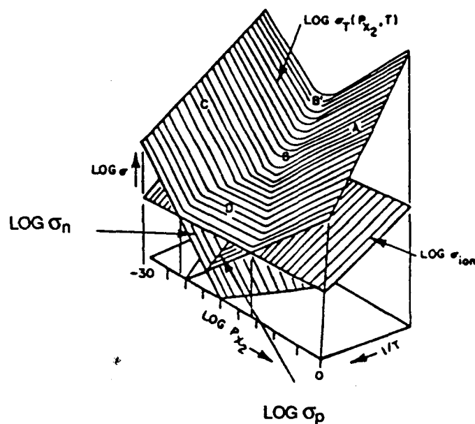
Figure 9. Schematic diagram of the P_{X_2} , T dependence of partial and total conductivities. A: \sigma_p \gg \sigma_{ion}, \sigma_n . B-B': \sigma_p = \sigma_n > \sigma_{ion} . C: \sigma_n \gg \sigma_{ion}, \sigma_p . D: \sigma_{ion} \gg \sigma_p + \sigma_n (Ref. 30).
