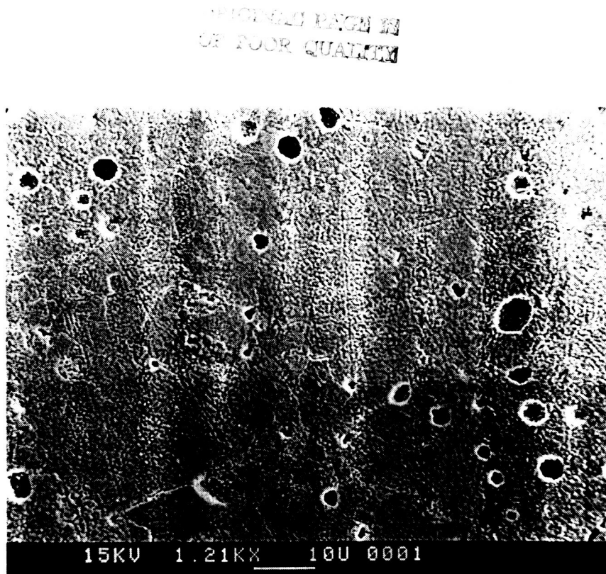
Figure 49. Scanning electron micrograph of a thermally etched, polished surface of a fired 10T_{2ox} bar.
