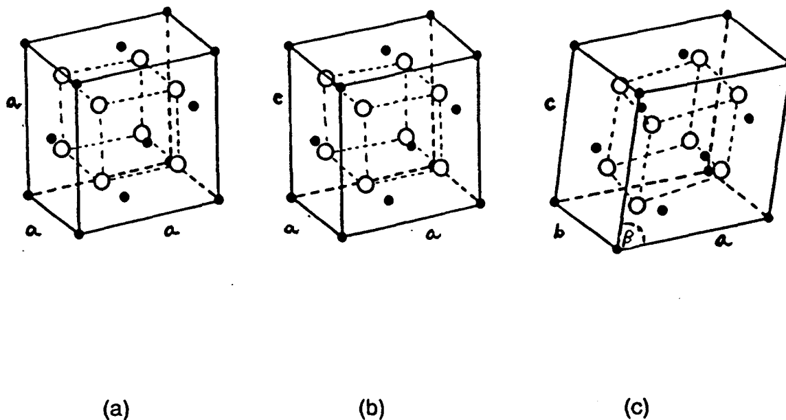
Figure 1. Polymorphic phases of the fluorite structure (a) cubic, (b) tetragonal, and (c) monoclinic. Solid circles: Zr^{4+} . Open circles: O^{2-} (Ref. 7).
