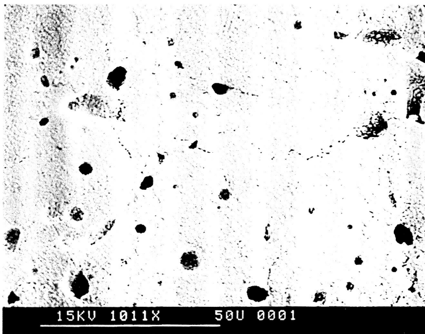
Figure 48. Scanning electron micrograph of a thermally etched, polished surface of a fired 5T_{2ox} bar.
