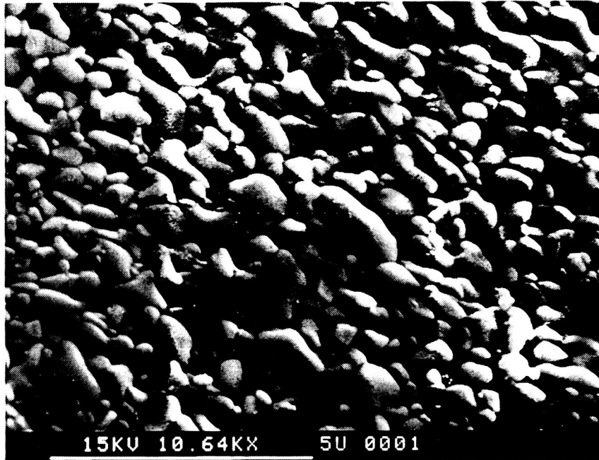
Figure 47. Scanning electron micrograph of a thermally etched, polished surface of a fired 20T_{1ox} bar.
