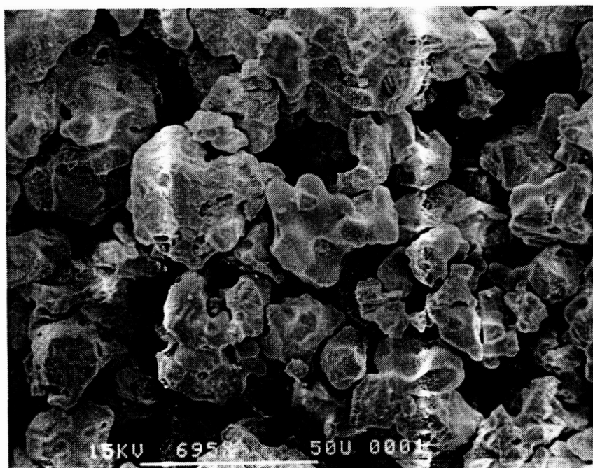
Figure 36. Scanning electron micrograph of as-received powder having 5 mol% \text{TiO}_2 ( 5T_2 ).
