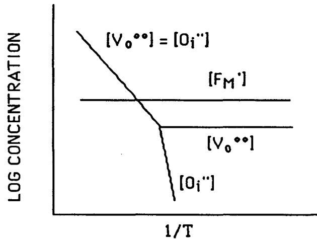
Figure 16. Schematic diagram demonstrating the effect of the temperature on defect concentration in MO_2-F_2O_3 at constant oxygen partial pressure (Ref. 28).
