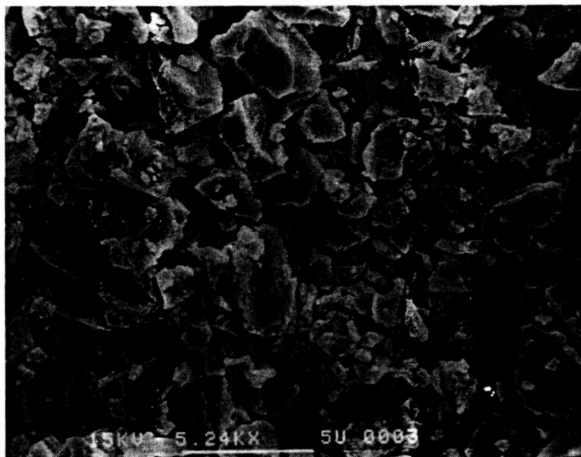
Figure 35. Scanning electron micrograph of reaction-sintered powder having 20 mol% \text{TiO}_2 ( 20T_1 ).
