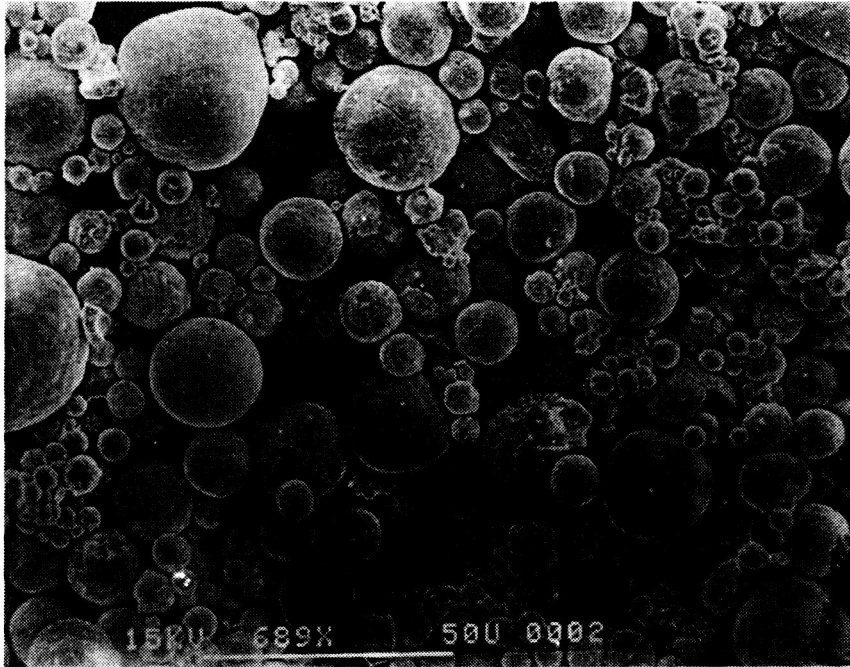
Figure 41. Scanning electron micrograph of plasma-sprayed powder having 10 mol% \text{TiO}_2 ( 10\text{T}_3 ).
