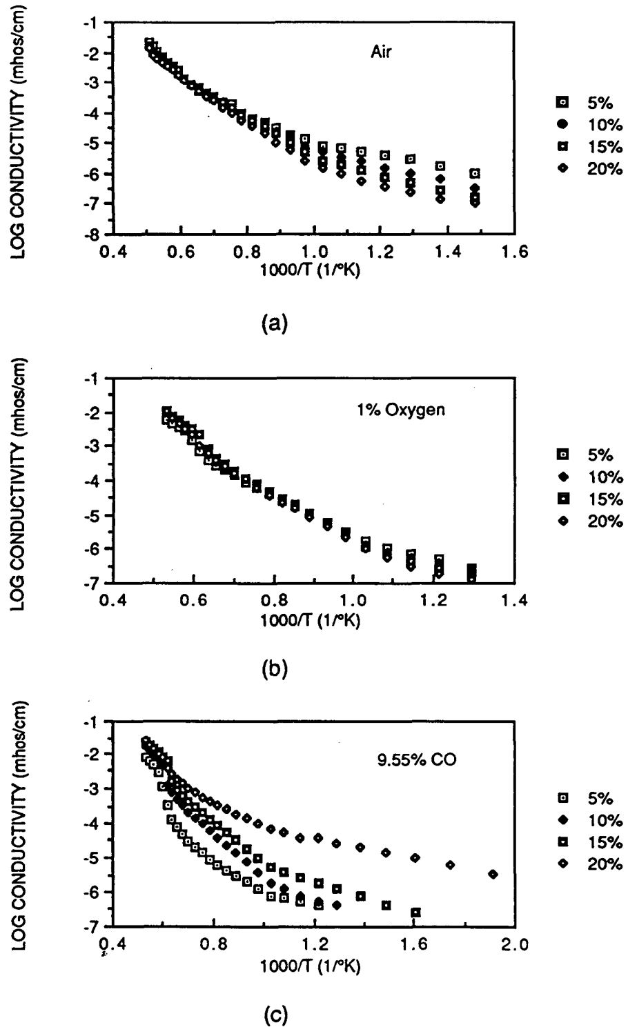
Figure 53. The electrical conductivity of four compositions in the HZT system measured as a function of temperature in (a) air, (b) 1% \text{O}_2 in Ar, and (c) 9.55% CO in \text{CO}_2 . The amount of \text{TiO}_2 in mol% is indicated on the right.
