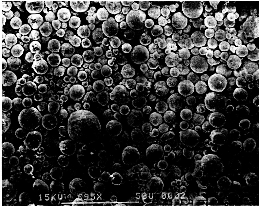
Figure 43. Scanning electron micrograph of plasma-sprayed powder having 20 mol% \text{TiO}_2 ( 20\text{T}_3 ).
