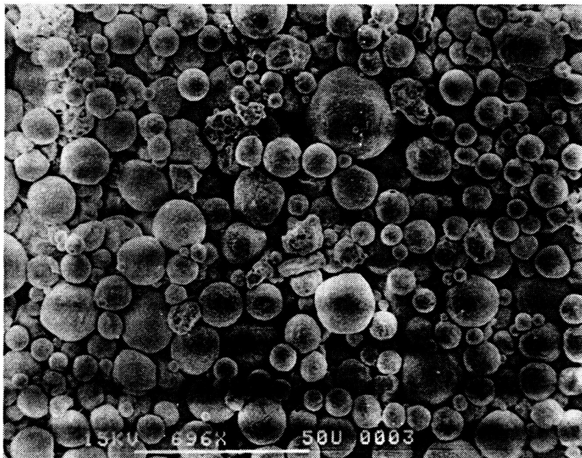
Figure 42. Scanning electron micrograph of plasma-sprayed powder having 15 mol% \text{TiO}_2 ( 15\text{T}_3 ).
