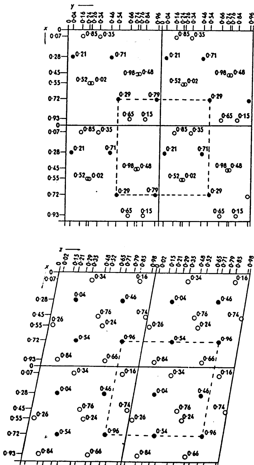
Figure 2. Lattice positions of the monoclinic cell of ZrO_2 . Solid circles: Zr^{4+} . Open circles: O^{2-} . Broken lines become tetragonal cell after transformation (Ref. 10).
