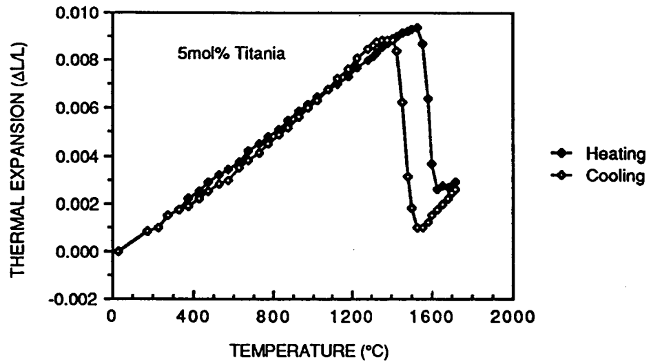
Figure 58. Linear thermal expansion of the 5 mol% \text{TiO}_2 composition in the HZT system.
