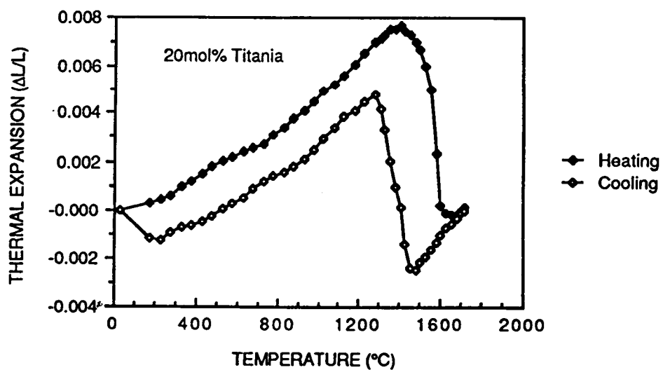
Figure 61. Linear thermal expansion of the 20 mol% TiO_2 composition in the HZT system.
