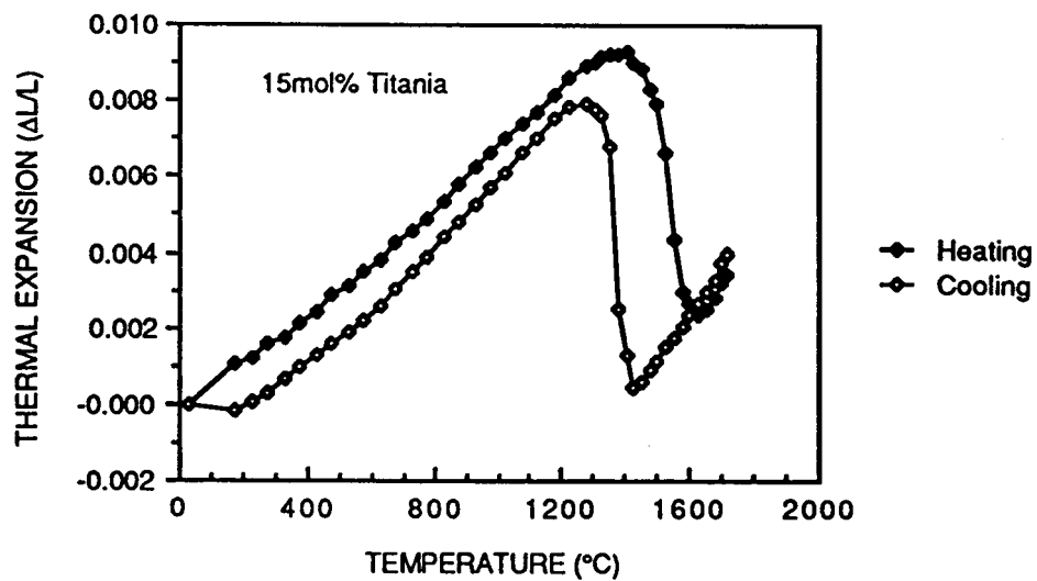
Figure 60. Linear thermal expansion of the 15 mol% TiO_2 composition in the HZT system.
