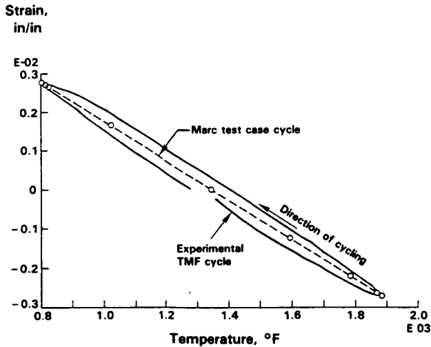
Strain and temperature vary sinusoidally with time
