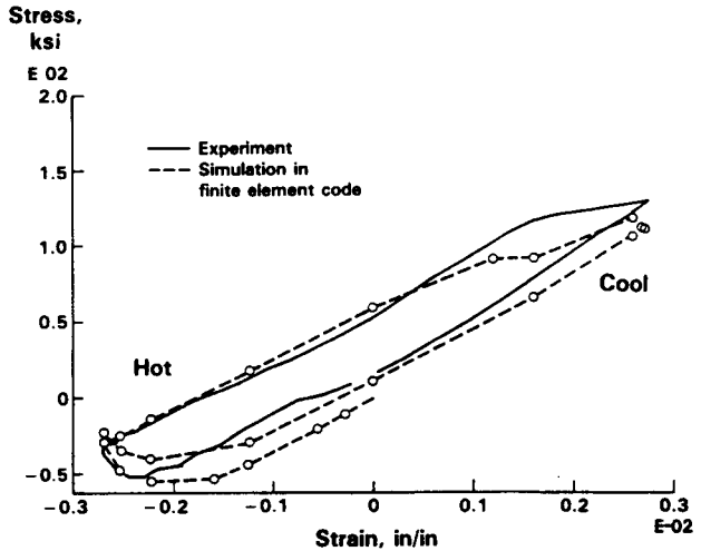
Stress vs. mechanical strain in thermomechanical fatigue test
