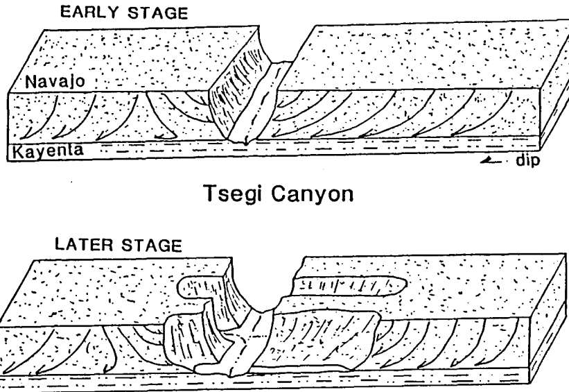
Figure 47. Schematic of groundwater recharge and asymmetrical valley development for Tsegi channels seen in Figure 46.
