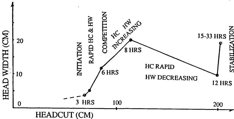
Figure 9. (top) Idealized channel evolution phases observed in the flume. (bottom) Example of sequence from Run 3.
