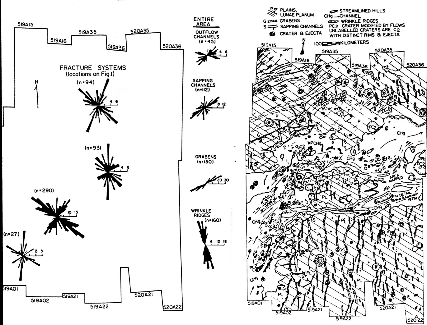
Figure 24. Sapping modified margins of western Kasei Vallis, outflow channel on Mars. Sapping has extended channel widths considerably by following structural trends. Note correspondence of structural features with channels (from Kochel and Burgess, 1983).
