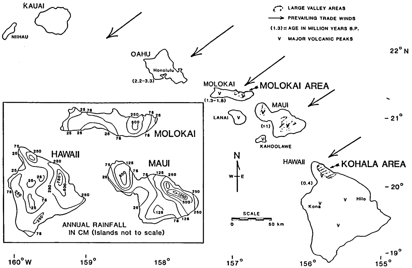
Figure 32. Index map and climate data for Hawaiian analog study sites.
