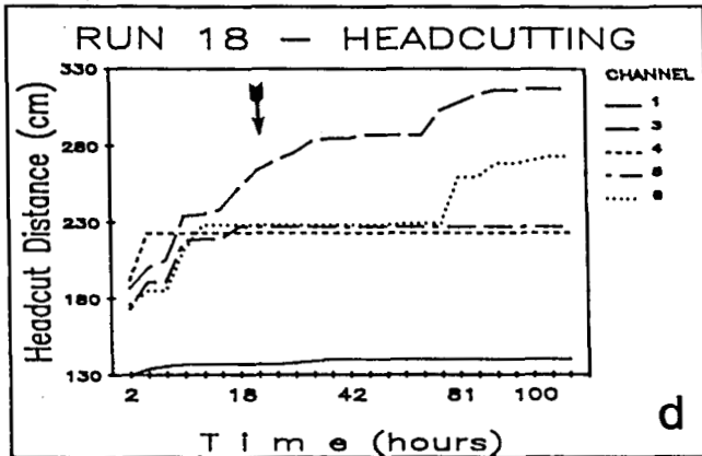
Figure 29. Channel morphodynamics for Run 18. Note rapid growth of channels once the diked aquifer is tapped at 18 hrs (from Kochel and Piper, 1986).
