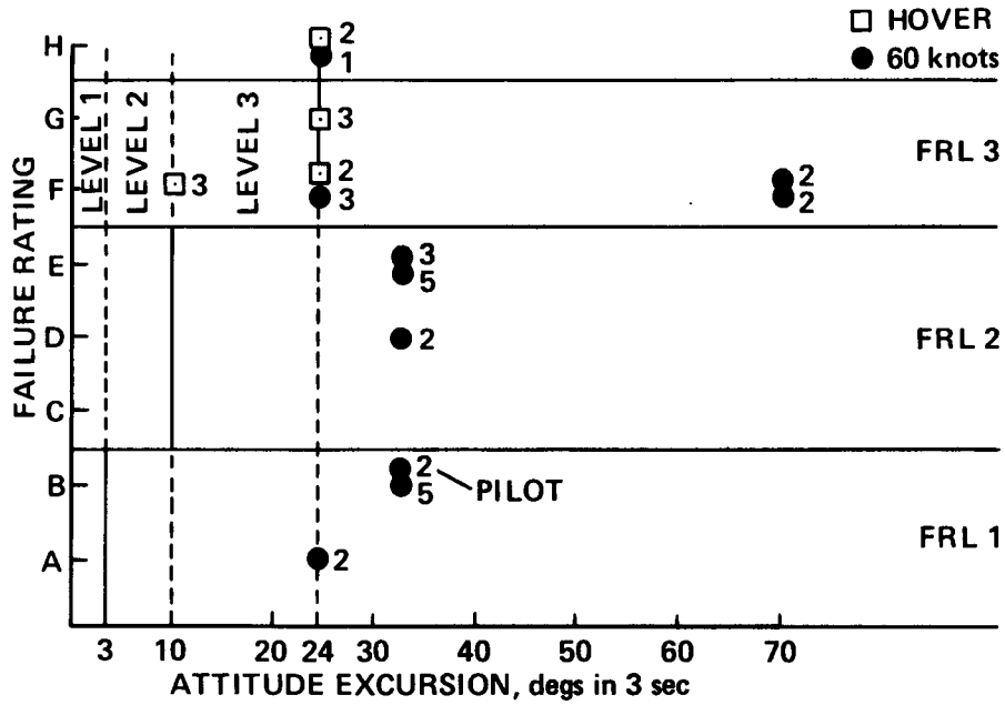
Figure 20. — Lateral axis failures.
