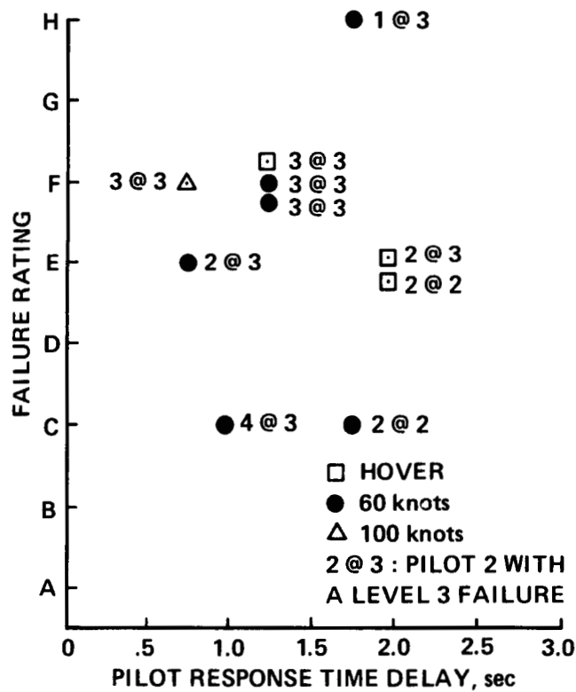
Figure 19. — Reaction time delays for longitudinal axis failures.
