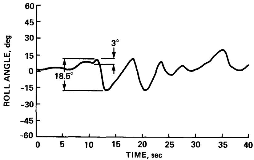
Figure 23. — Time history for new level 2 roll-axis failure.
