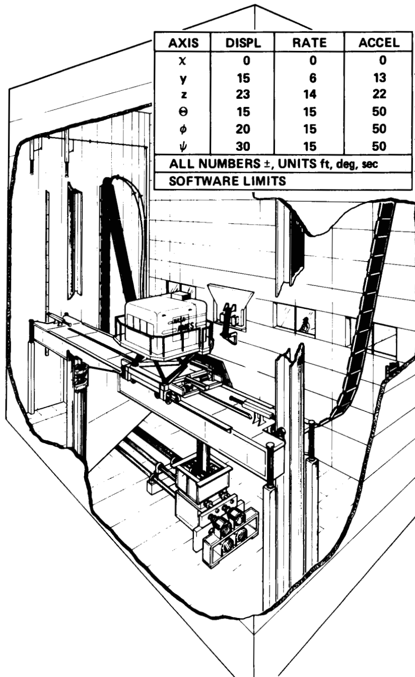
Figure 12. — Vertical motion simulator.
