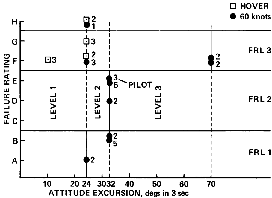
Figure 21. — Suggested revision for lateral axis failures.
