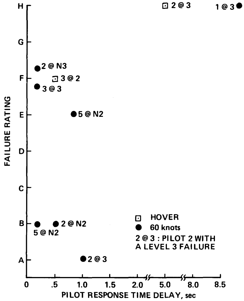
Figure 22. — Reaction time delays for lateral axis failures.
