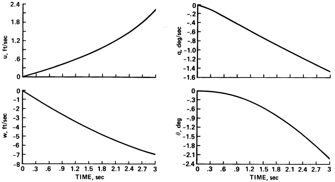
Figure 6. — Response to an equivalent 1-in. collective input.
