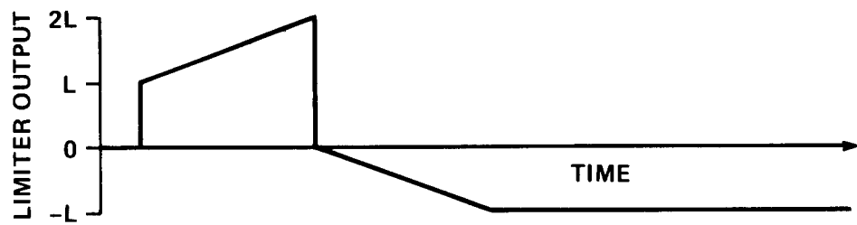
Figure 3. — AFCS-PFCS interface limiter.
