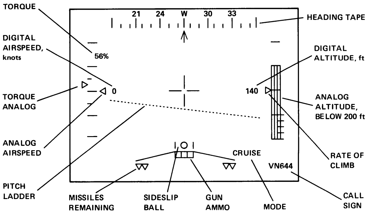
Figure 16. — Cruise head-up display.
