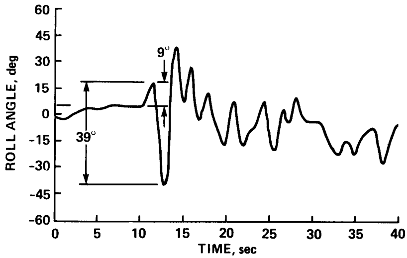
Figure 24. — Time history for new level 2 roll-axis failure.
