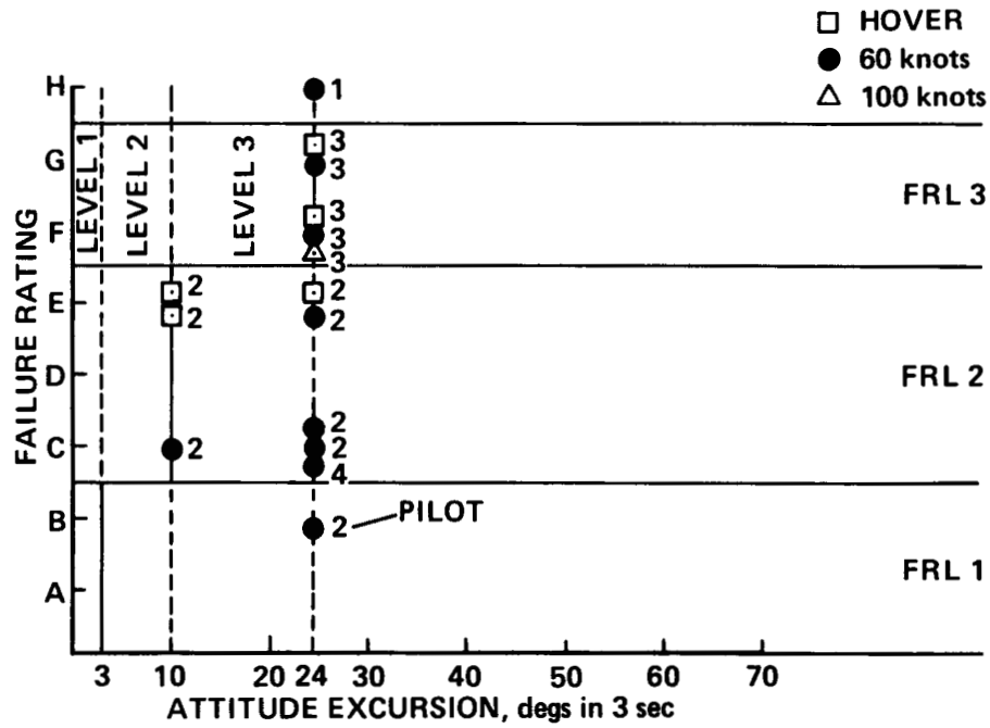
Figure 18. — Longitudinal axis failures.
