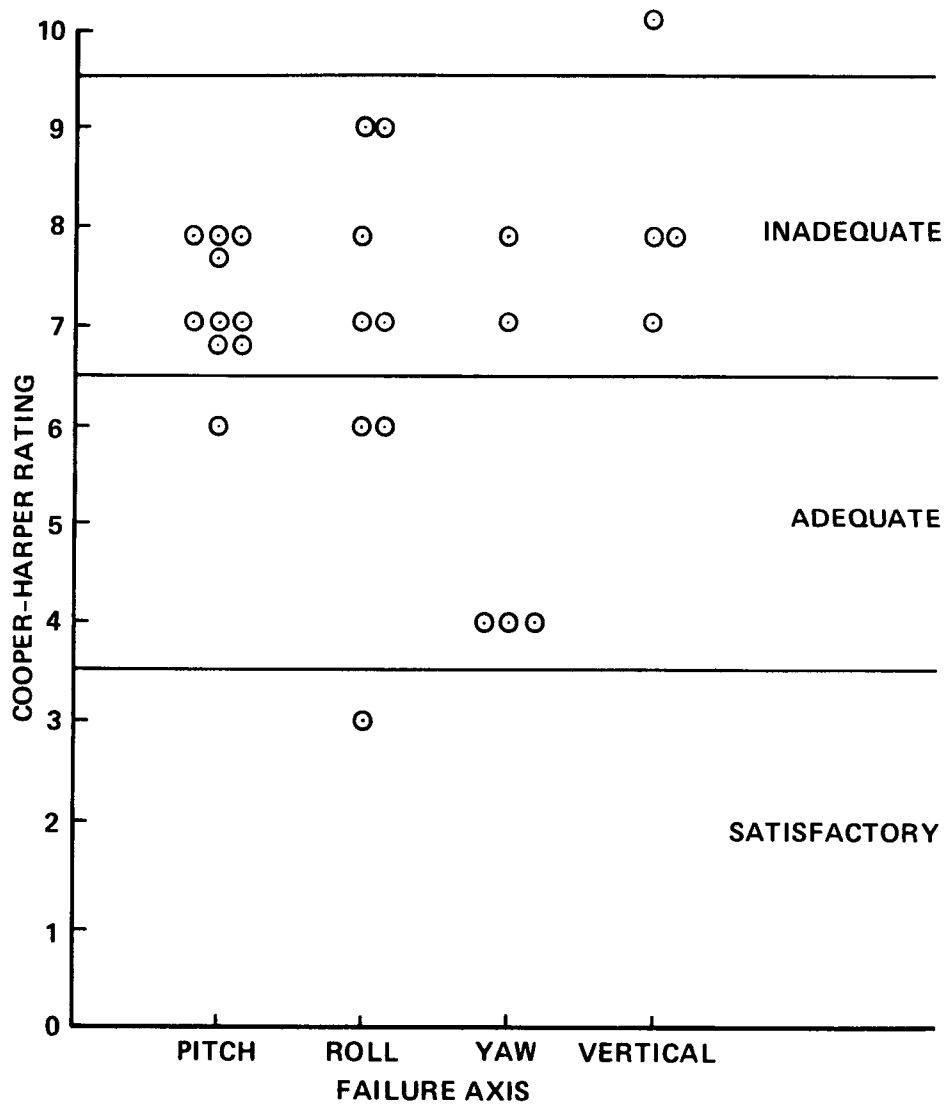
Figure 17. — Cooper-Harper ratings for the post-failed aircraft.
