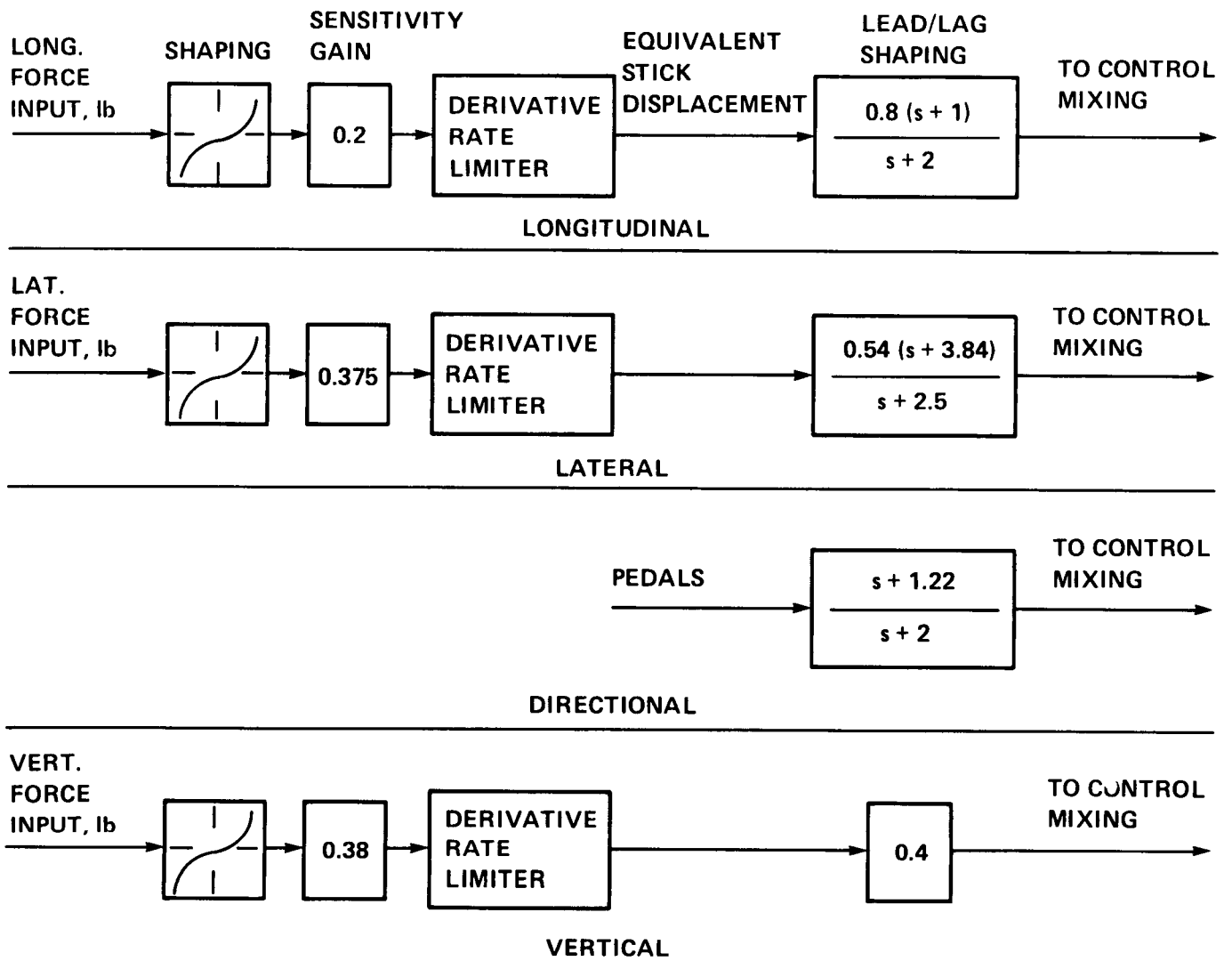
Figure 4. — PFCS block diagram.
