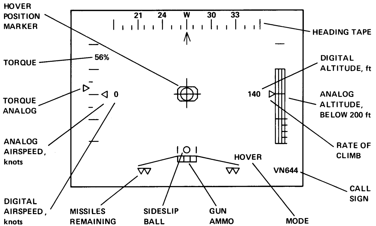
Figure 15. — Hover head-up display.
