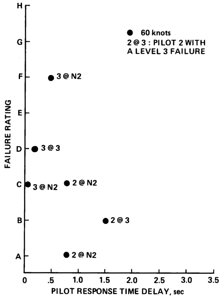
Figure 26. — Reaction time delays for directional axis failures.
