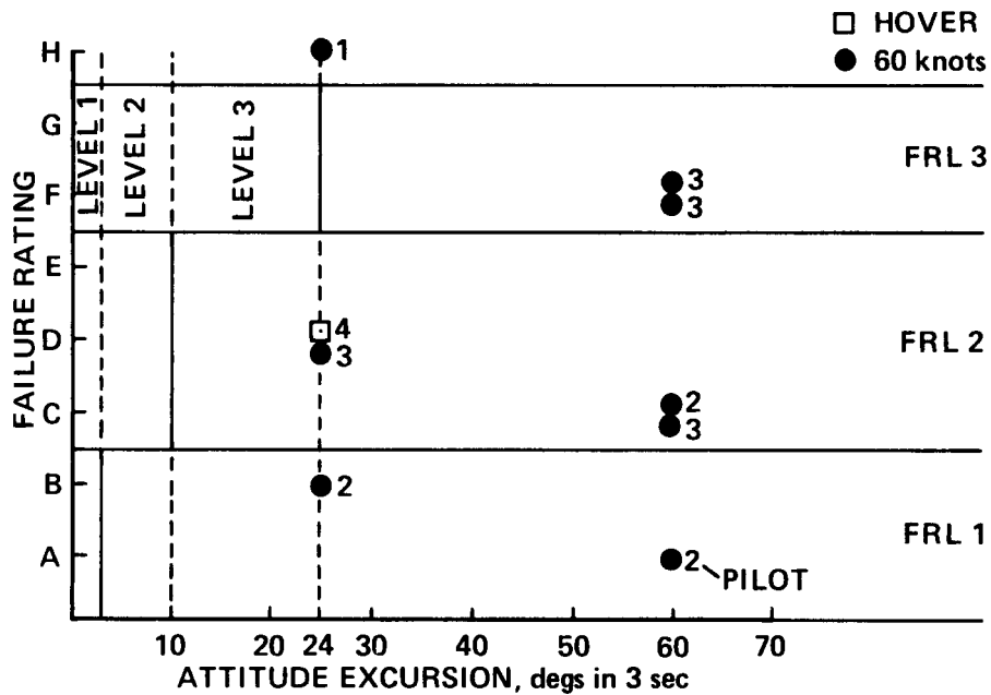
Figure 25. — Direction axis failures.
