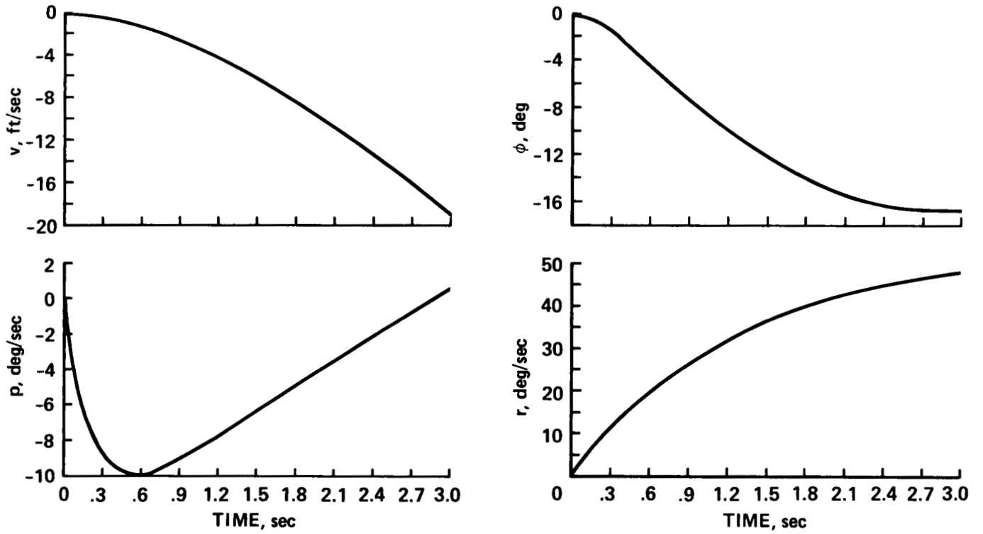
Figure 8. — Response to an equivalent 1-in. pedal input.
