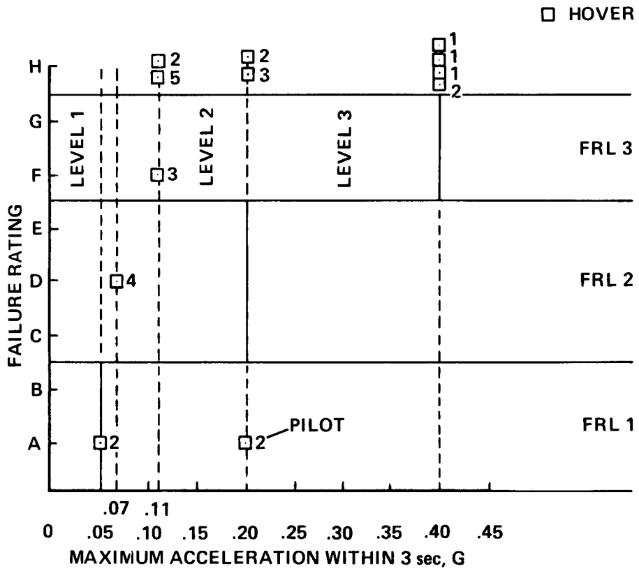
Figure 27. — Vertical axis failures.
