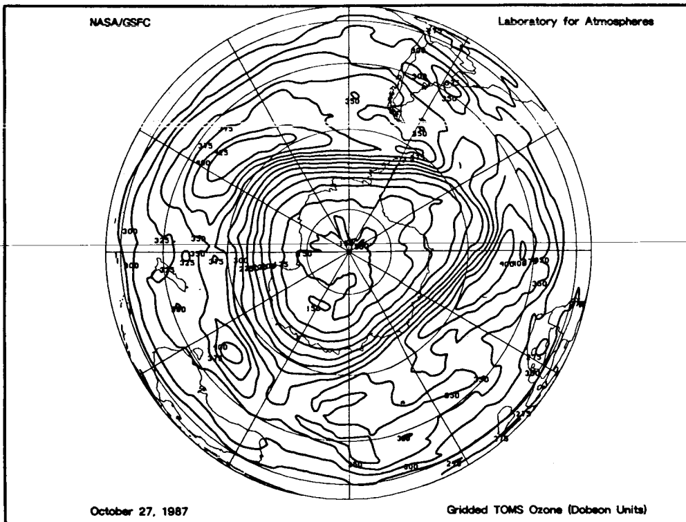
Figure 32a-b. TMS ozone distribution for the southern hemisphere on October 22 and 27, 1987.
