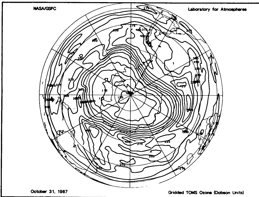
Figure 32c-d. TMS ozone distribution for the southern hemisphere on October 28 and 31, 1987.
