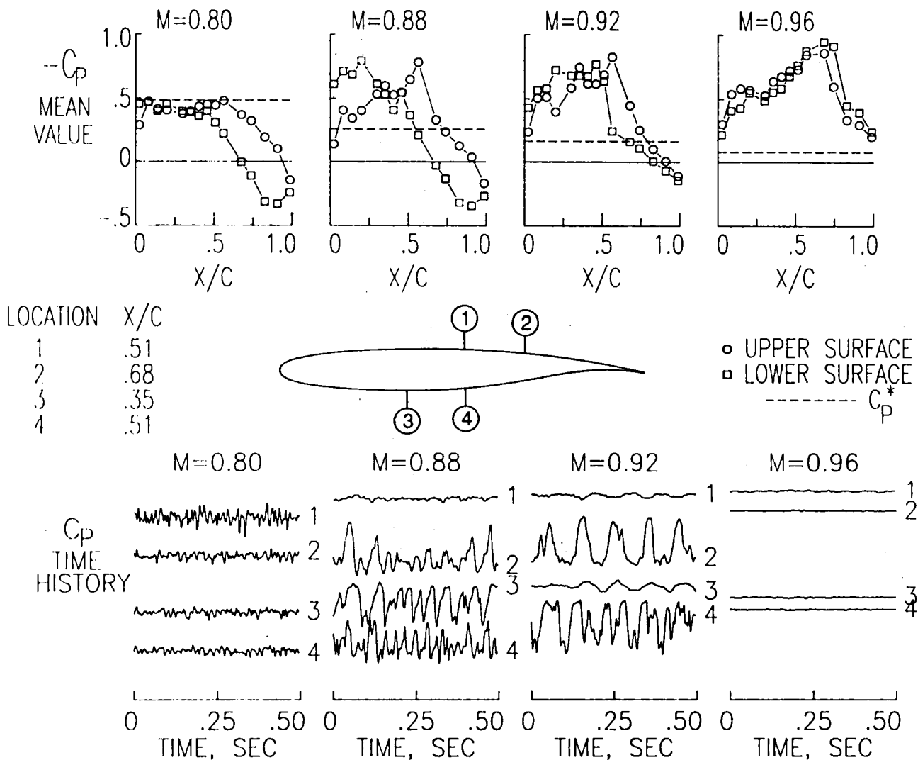
Figure 7.- Mean value chordwise pressure distributions and sample pressure measurement time histories (high q test condition, \eta=.87 ).
