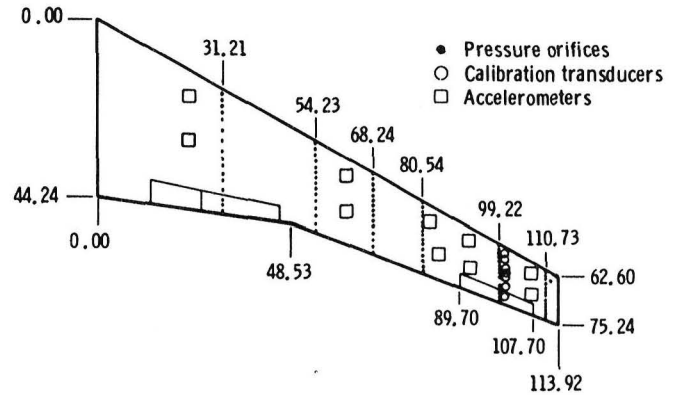
Figure 2.- Wing planform and instrumentation locations (in inches).
