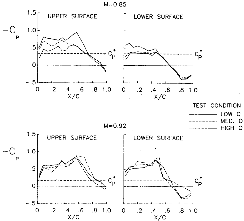
Figure 12.- Pressure distribution variations with test dynamic pressure ( \eta=0.87 ).
