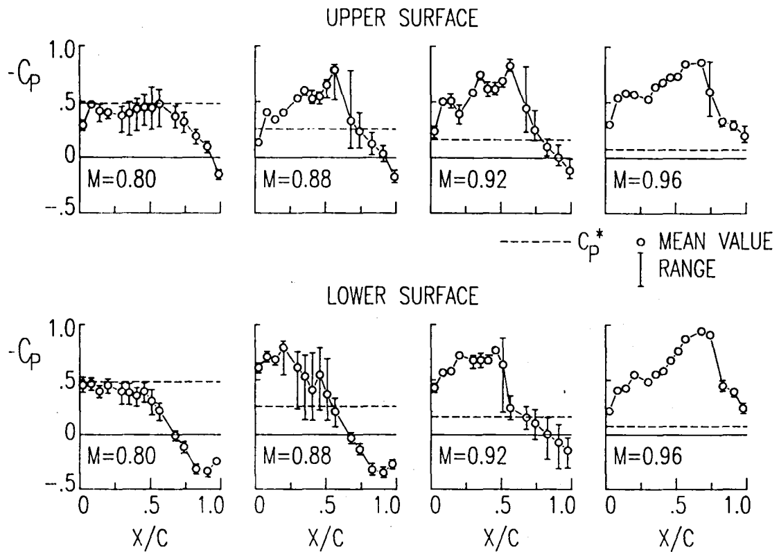
Figure 8.- Chordwise pressure distribution mean values and measurement ranges for representative Mach numbers (high q test condition, \eta=0.87 ).
