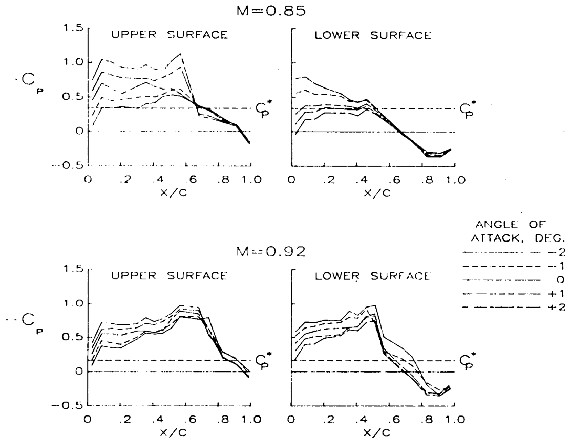
Figure 13.- Pressure distribution variations with angle of attack (medium q test condition, \eta=0.87 ).
