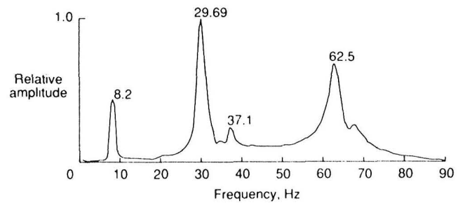
Figure 3.- Wing frequency response characteristics measured in still air.
