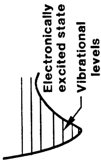
Rayleigh (elastic)
