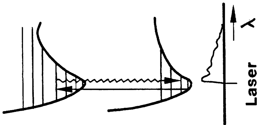
Fluorescence
