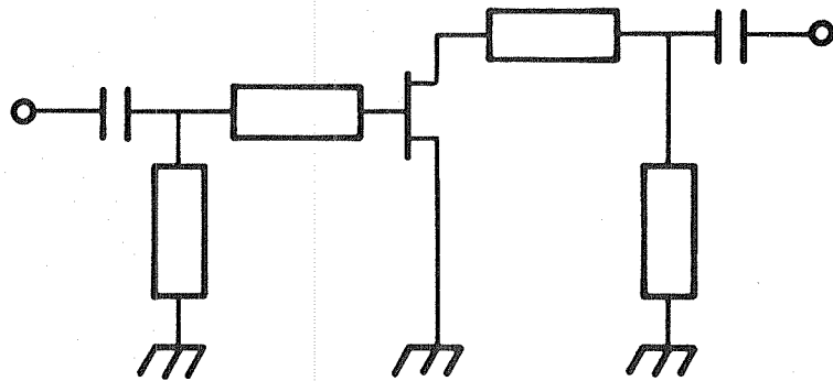
Fig. 5 Schematic of a single-stage buffer amplifier.
