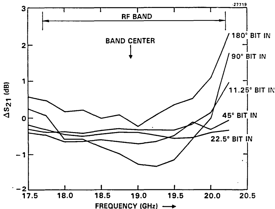
Fig. 39 Differential insertion loss for five different phase shifter states.
