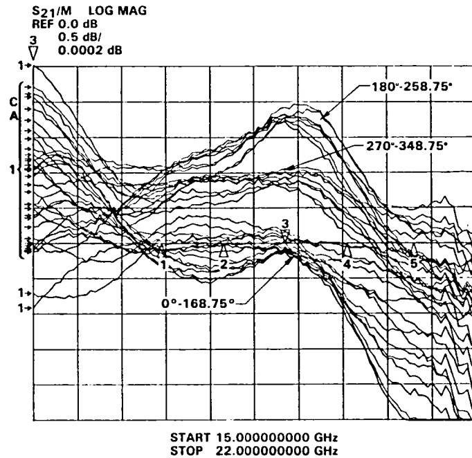
Fig. 44 Survey of the insertion loss delta for all 32 phase-setting combinations, chip 104271-1-6.
