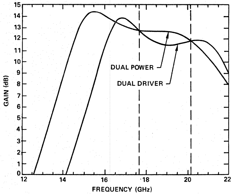
Fig. 26 Predicted gain of the two-stage driver combinations of Fig. 25.
