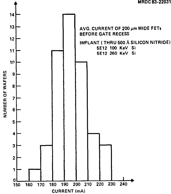
Fig. 50 A histogram of I_{dss} values in 200 μm wide FETs on an implanted layer. These values were measured prior to gate recess etch.
