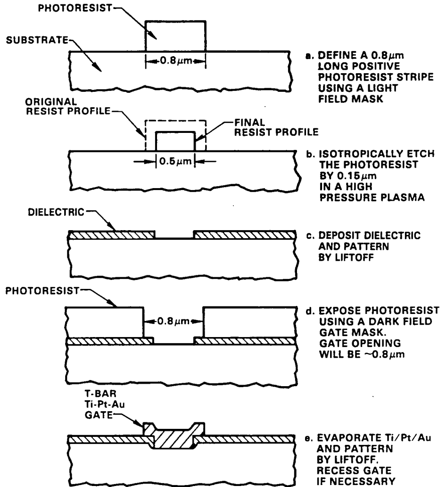
Fig. 55 An optical lithography technology for the realization of sub 0.5 μm gate length FETs.
