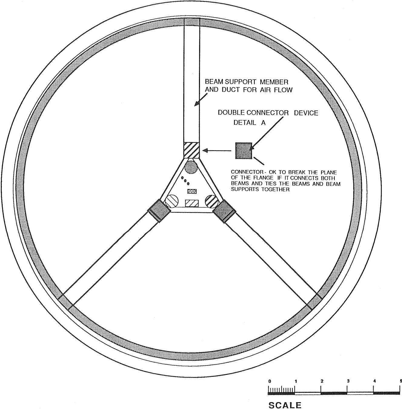
Figure 64 Triangular Beam Model Details
