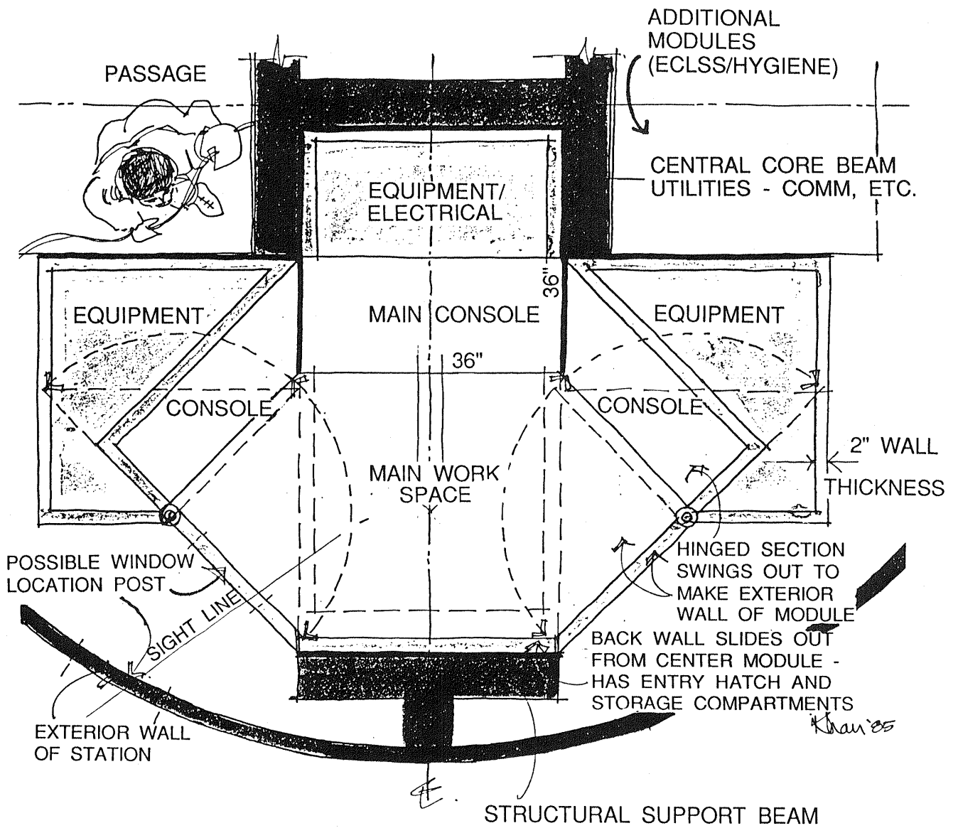
TYPICAL WORK STATION CONCEPT - MODULAR SYSTEM FROM 3 MODULES - (3' X 3' X 7')
