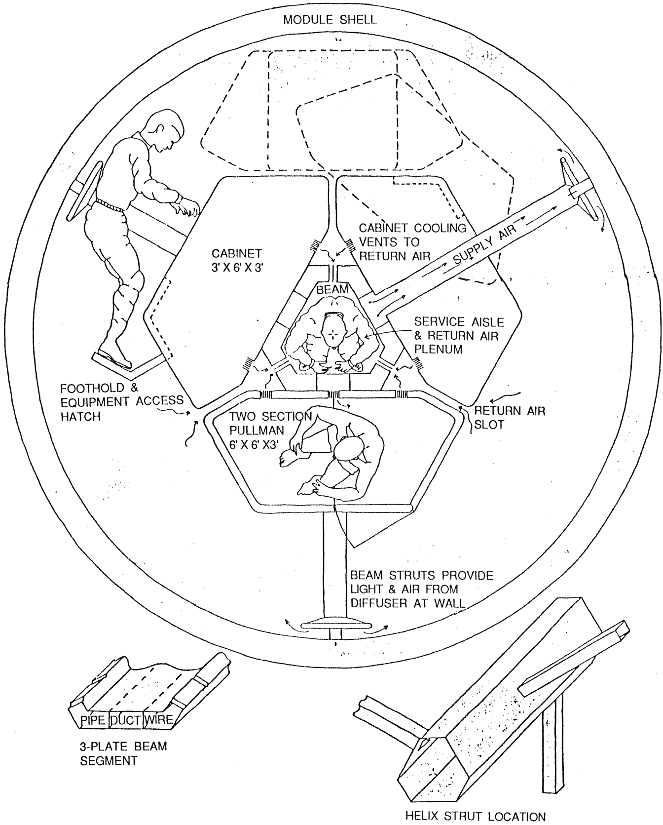
Figure 56 Dense Pack Triangular
