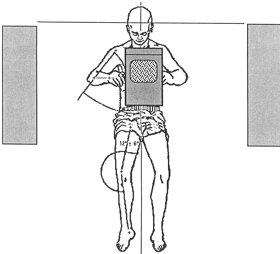
Figure 19 Top View - Engineering Workstation
