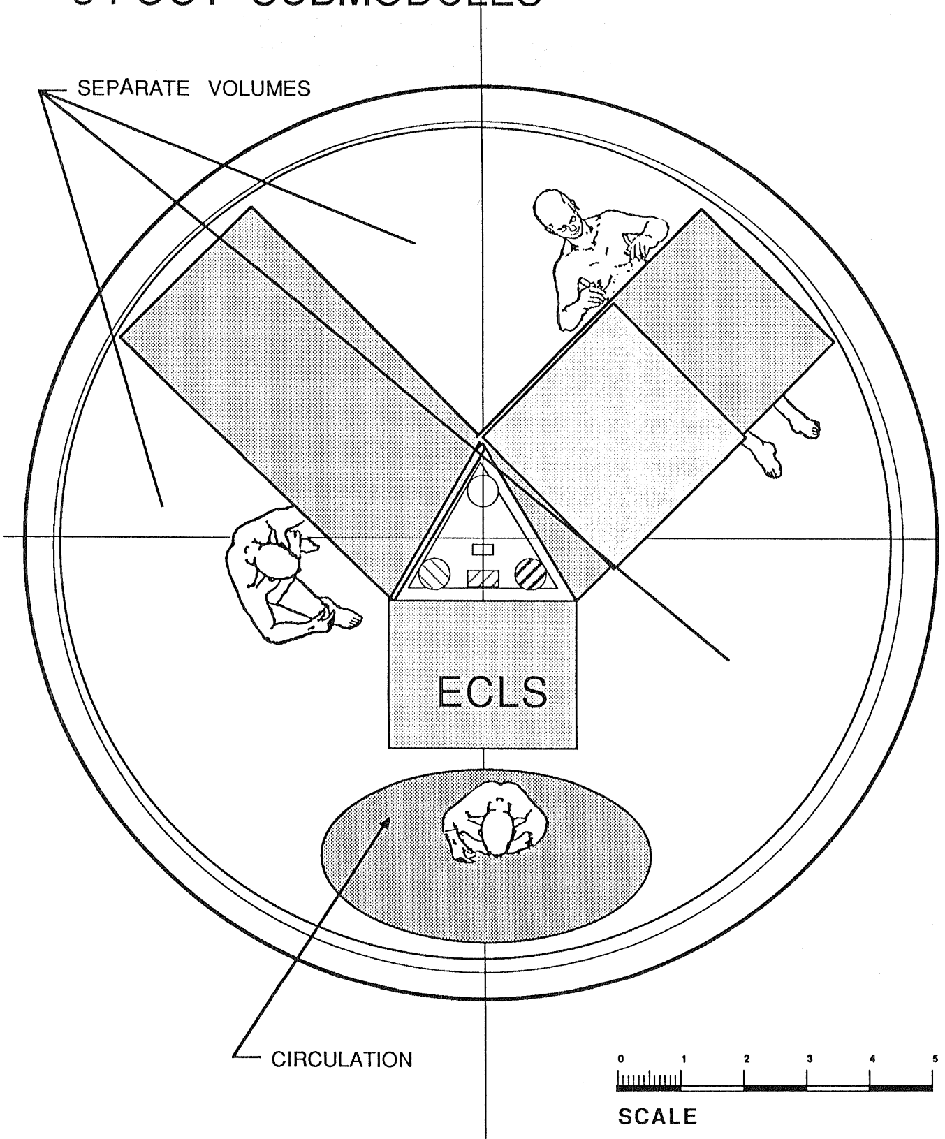
Figure 33 Equilateral Triangular Beam - On Center
