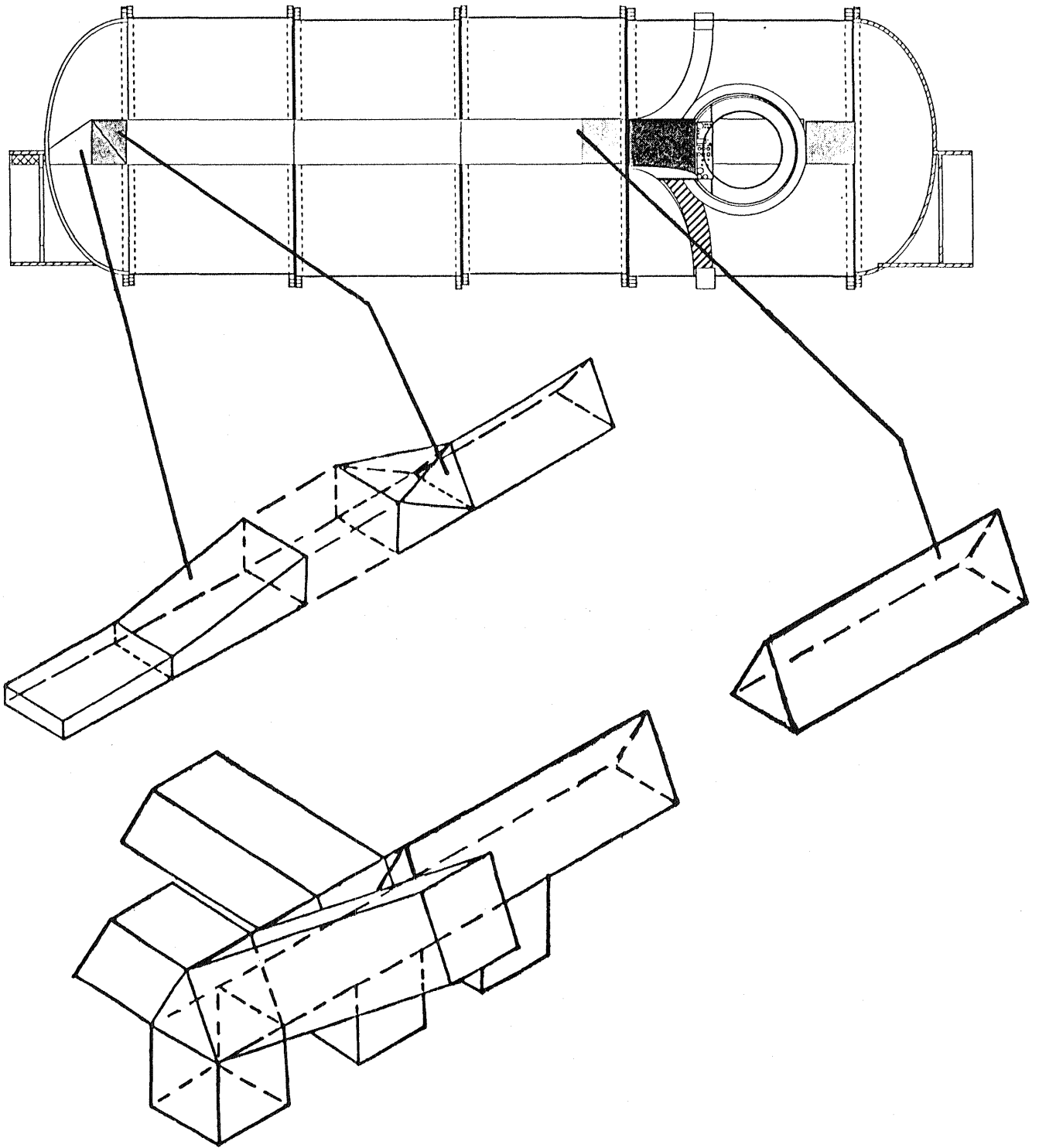
Figure 59 Transition Details
