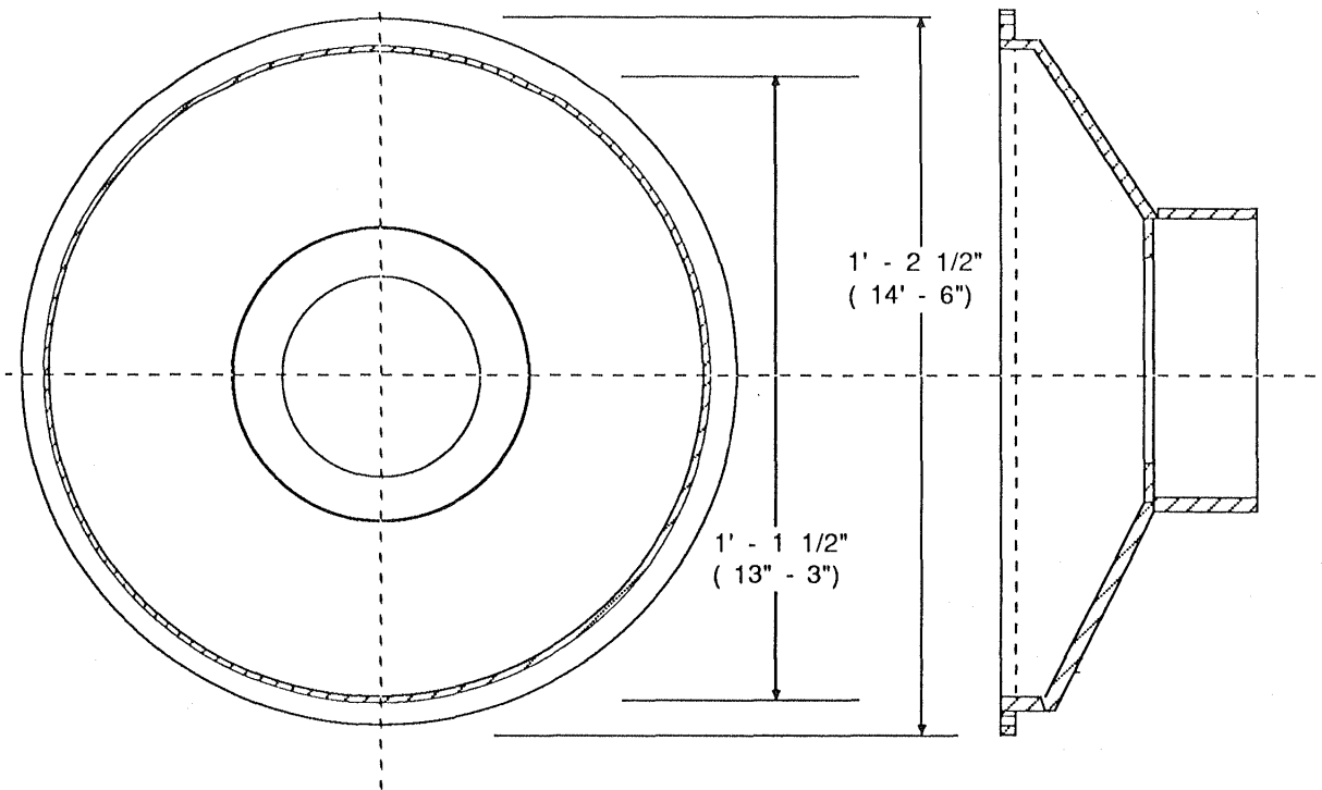
Figure 68 Volume and Packing Details
