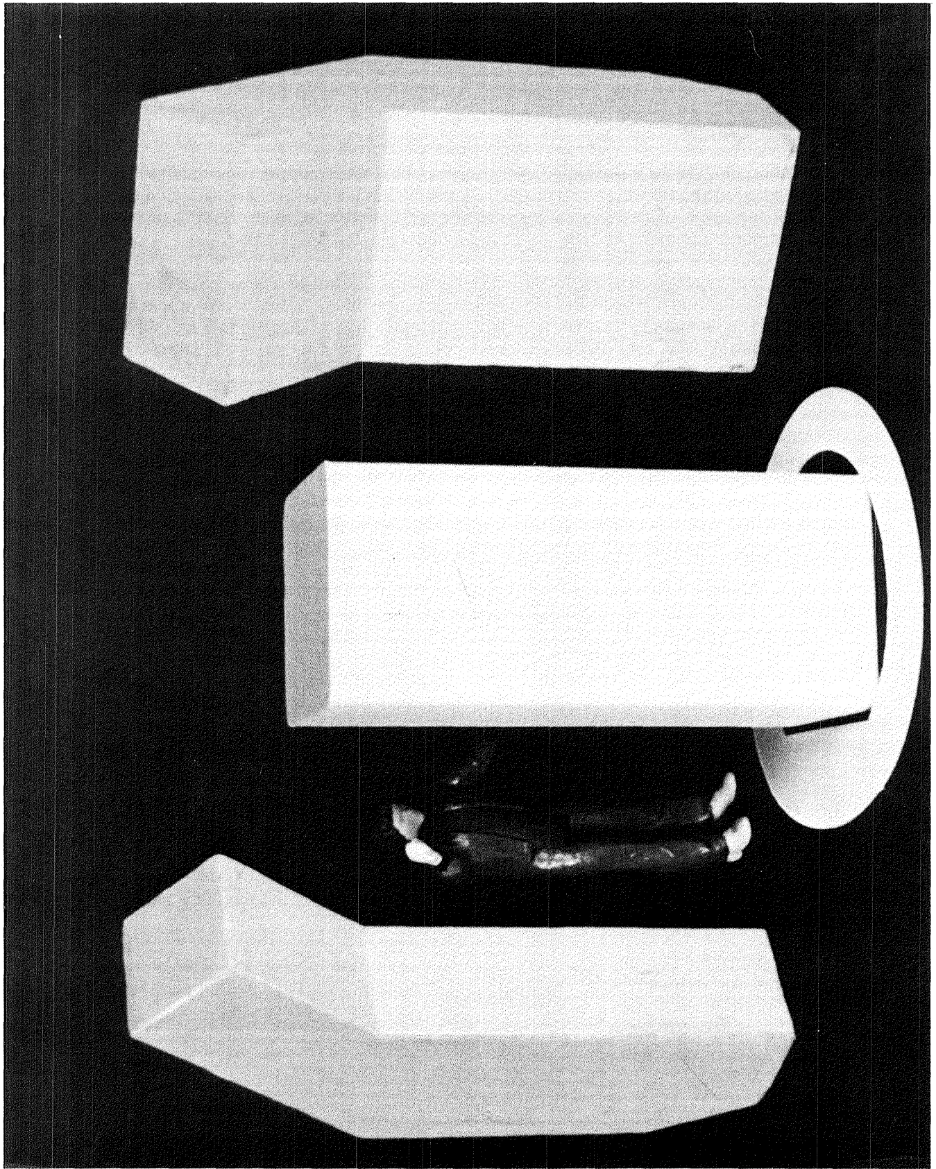
Photograph-3 Hatch with Sub Module, Spacelab Racks and Scaled Human
