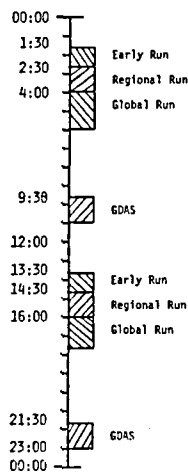
Figure 2. Structure of Current NMC Operational Prediction Models.
