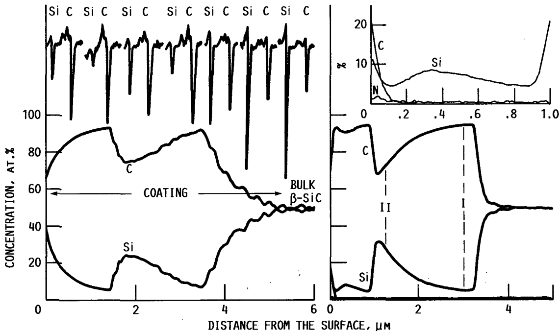
(a) "AS-RECEIVED" FIBER WITH CHARACTERISTIC Si AND C AUGER dN(E)/dE PEAK SHAPES CORRESPONDING TO CONCENTRATION. (b) FIBER AFTER ANNEAL (1 ATM N_2 AT 1200 °C FOR 40 HR) WITH INSET SHOWING NEAR SURFACE DETAIL.
