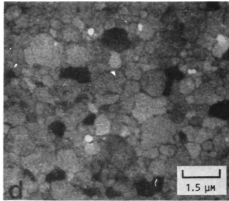
(D) HEAT-TREATED AT 400 °C AGED FOR 9 MONTHS.
