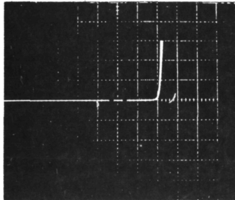
(C) 396 °C FOR 20 SEC WITH TiN AGED FOR 8 MONTHS.
