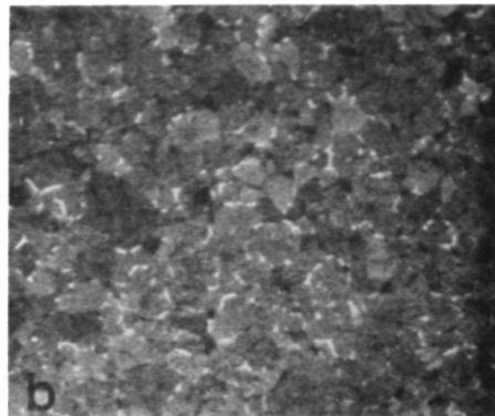
(B) AS-DEPOSITED AGED FOR 11 MONTHS.
