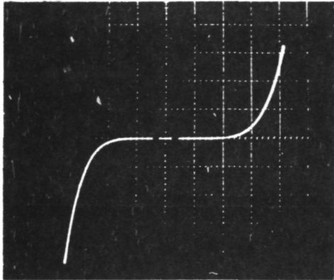
(A) NEW CONTACTS ARE RECTIFYING (1.0V, 1mA/DIV.).
