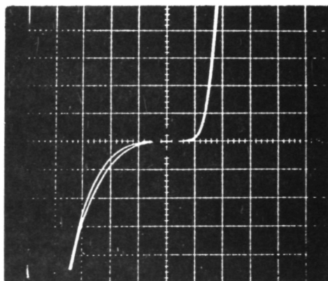
(D) MOST TYPICAL WITH AS-DEPOSITED AGED CONTACTS (0.5V, 1mA/DIV.).
