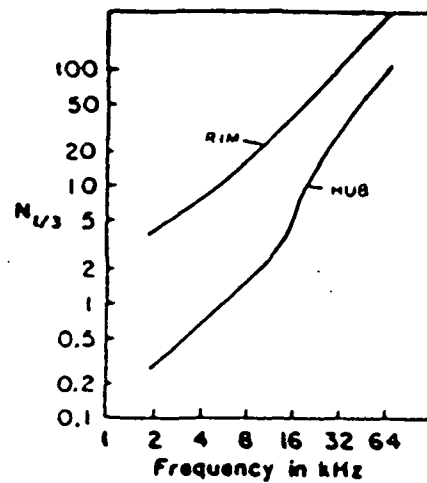
Figure 20. Mode counts in third-octave bands for rim and hub of a gear [7]
