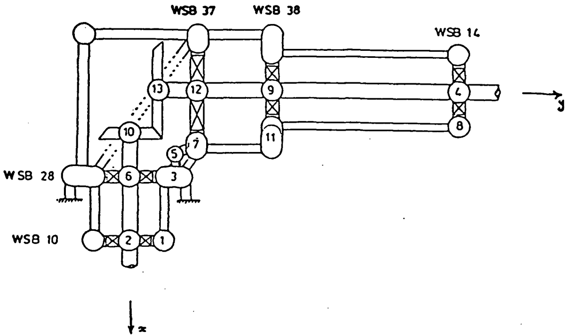
Figure 7. Wessex Tail Rotor Gearbox model idealization and the location of lumped-masses and inertias [24]
