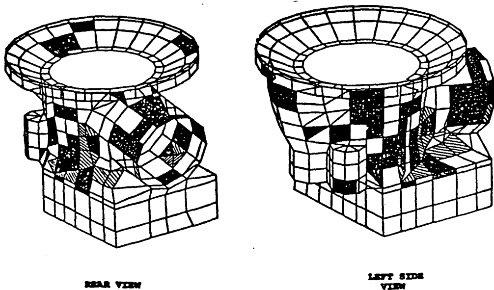
Figure 33. Areas of high strain energy density for modes 3 and 4 [8]
