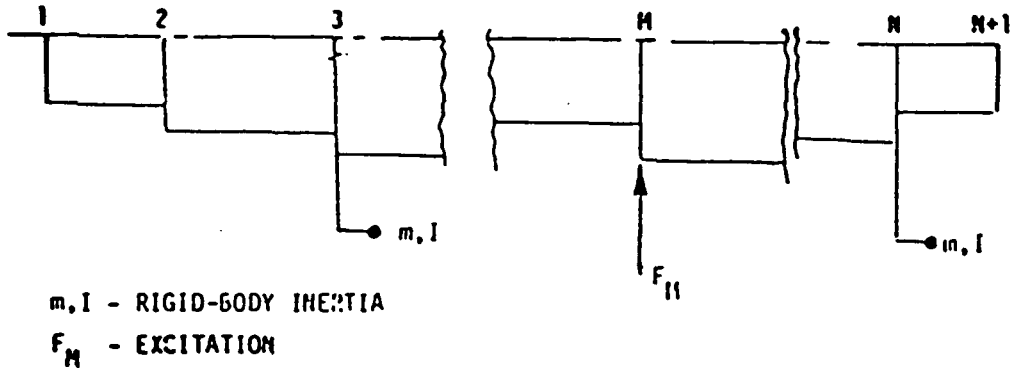
Figure 4. Geared system representation [19]
