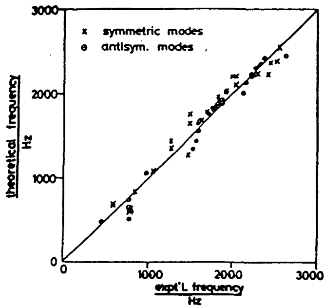
Figure 31. Correlation of theoretical and experimental natural frequencies [47]
