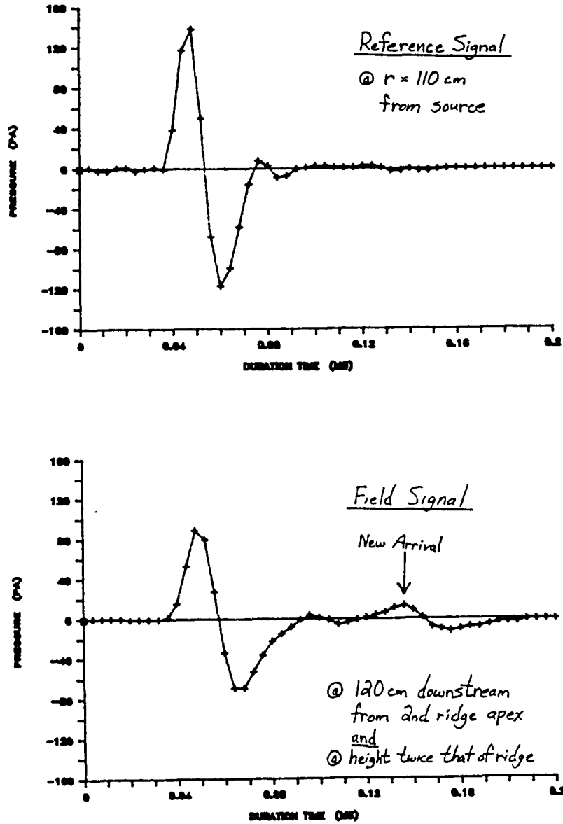
Figure 8. Arrival pulses at the reference microphone (top) and at the field microphone (bottom). The reference microphone is located 110cm from the source and such that no reflections are captured. In this figure, the field microphone is located 120 cm downstream from the second ridge and at a height twice that of the ridge. Correction for spherical spreading losses has been made. Notice the trailing pulse arrival in the bottom figure. Due to its position and magnitude, this arrival is believed to have been diffracted by the first ridge and then reflected by the forward surface of the second ridge.
