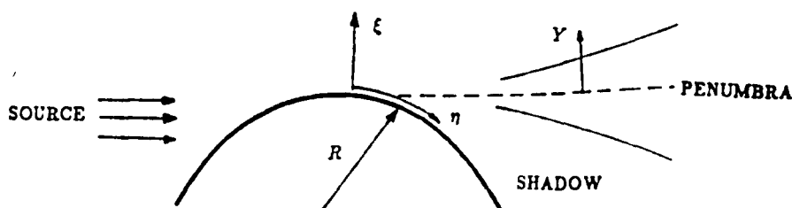
Figure 1: Geometry of the diffraction problem
