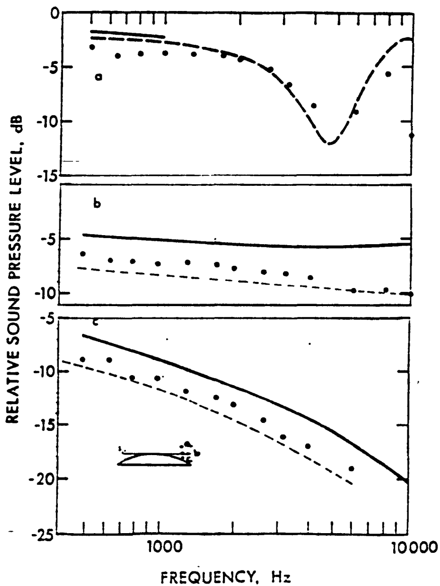
Figure 3 : Relative Sound Pressure Level in the penumbra
