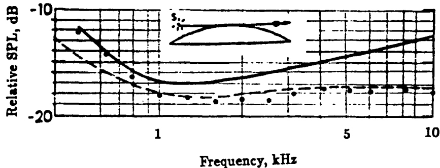
Figure 3 : Relative Sound Pressure Level in the penumbra • • • : Data from Berry and Daigle [11] ——— : Prediction from the creeping wave series [11] - - - - : Prediction from MAE theory [Eq. (3)]
