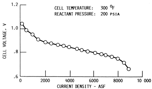
FIGURE 4. - PERFORMANCE CALIBRATION.
