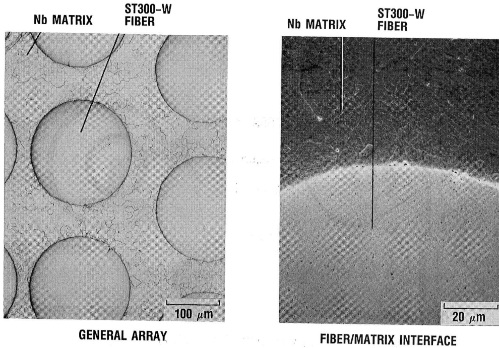
FIGURE 14. - TUNGSTEN FIBER REINFORCED NIOBIUM MATRIX COMPOSITES AS-FABRICATED MICROSTRUCTURE.
