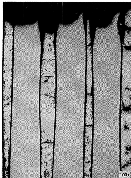
FIGURE 21. - FRACTURE SECTION OF ST300/Nb + 1Zr CREEP RUPTURE SPECIMEN.
