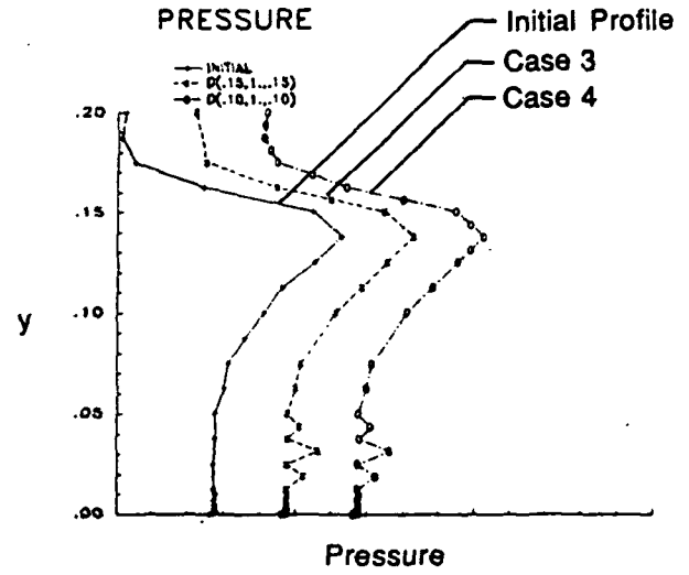
Fig. 39 Pressure profiles on ramp showing effects of varying threshold values.
