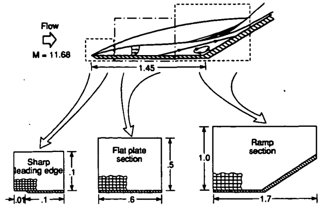
Fig. 5 Subdivision of hypersonic flow domain.
