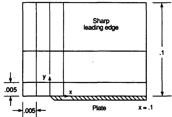
Fig. 6 Skeleton mesh for sharp leading edge.
