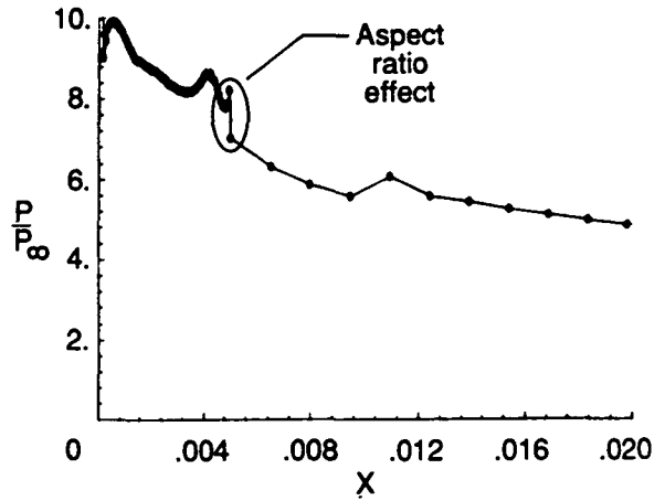
Fig. 9 Pressure distribution in the vicinity of the leading edge.
