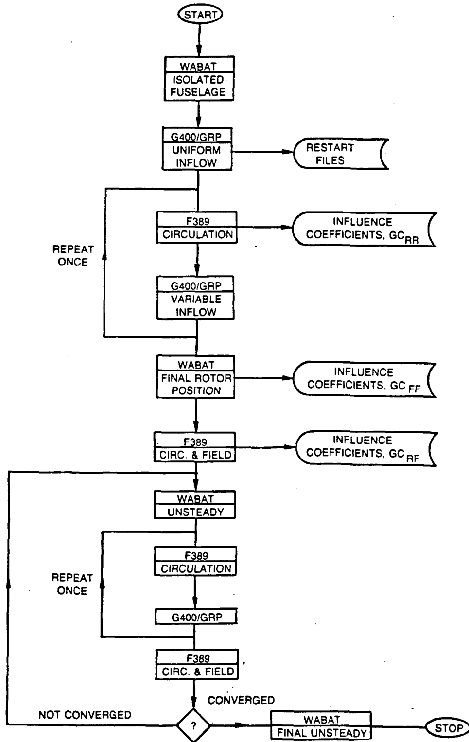
Figure 1. Program calling sequence (concluded).
