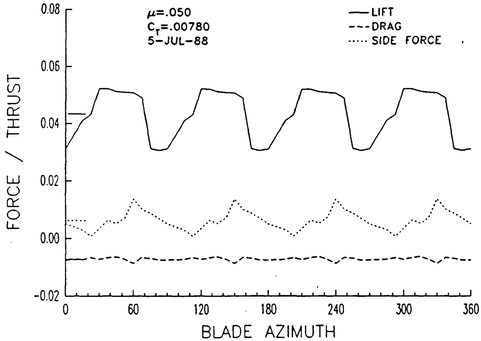
a) Aerodynamic forces on the fuselage.
