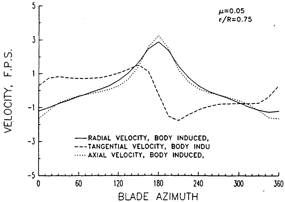
b) Fuselage-induced velocities at the rotor.
