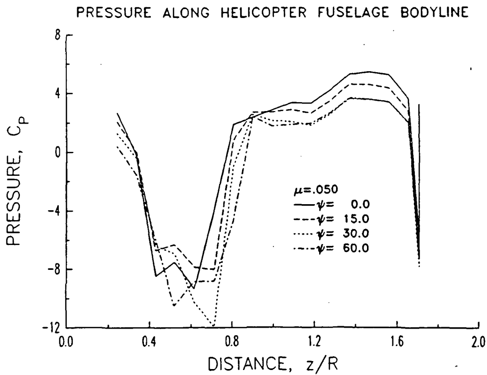
b) Pressure along a fuselage bodyline.
