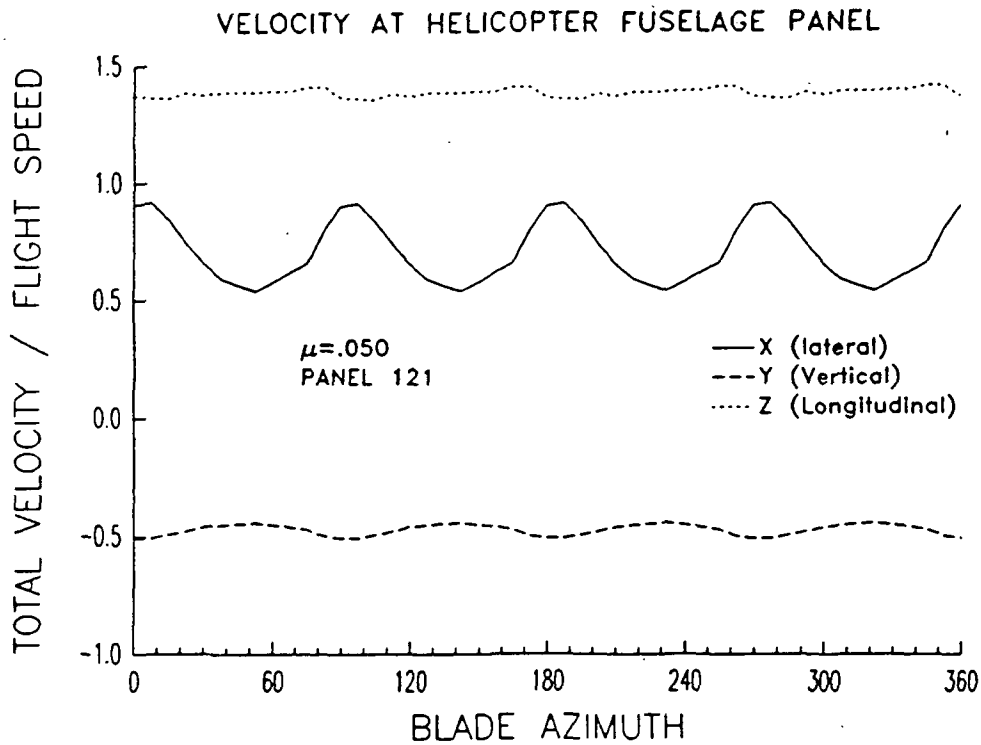
a) Time history of the velocity at a fuselage panel.
