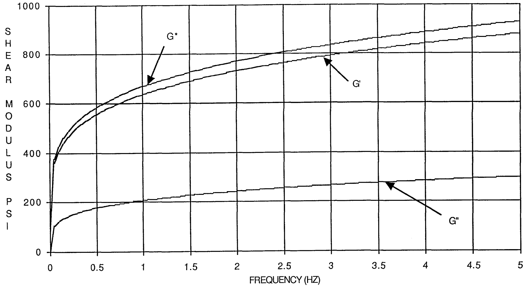
Figure 21. Dynamic shear modulus of TP-H1148 SRM propellant based on power equation fit of stress relaxation data.
