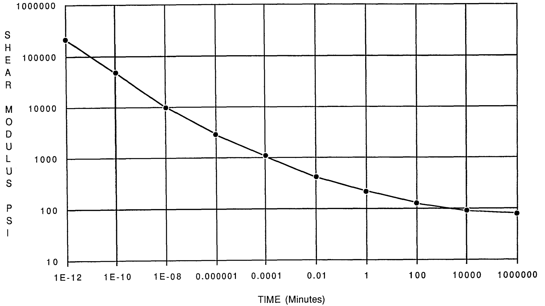
Figure 9. Log shear modulus G(t) versus log time.
