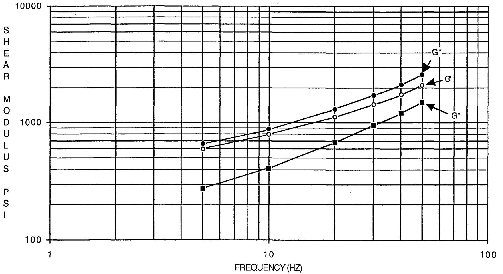
Figure 17. Dynamic shear modulus of TP-H1148 SRM propellant, mix 9910060 at 70°F, sample 36 from TWR-11779.
