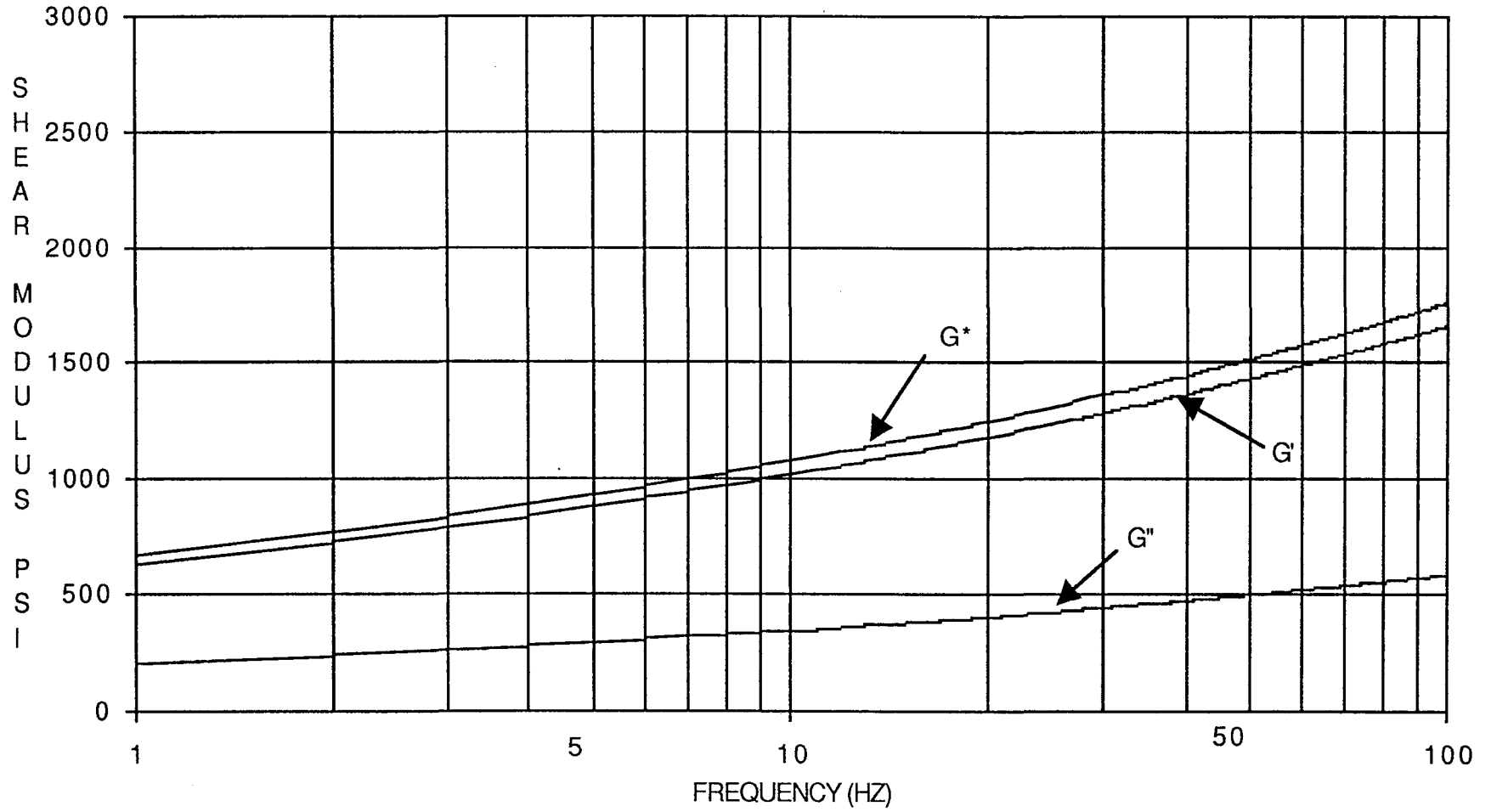
Figure 22. Dynamic shear modulus of TP-H1148 SRM propellant based on power equation fit of stress relaxation data.
