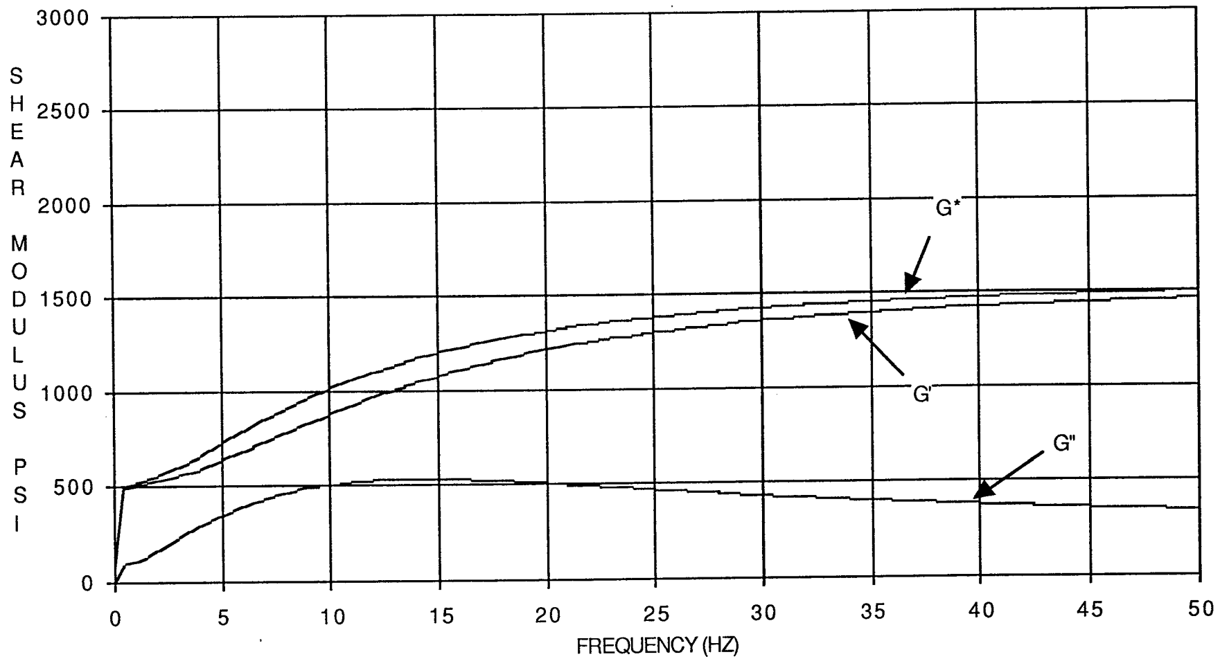
Figure 8. Dynamic shear modulus of TP-H1148 SRM propellant based on Prony Series fit of stress relaxation data.
