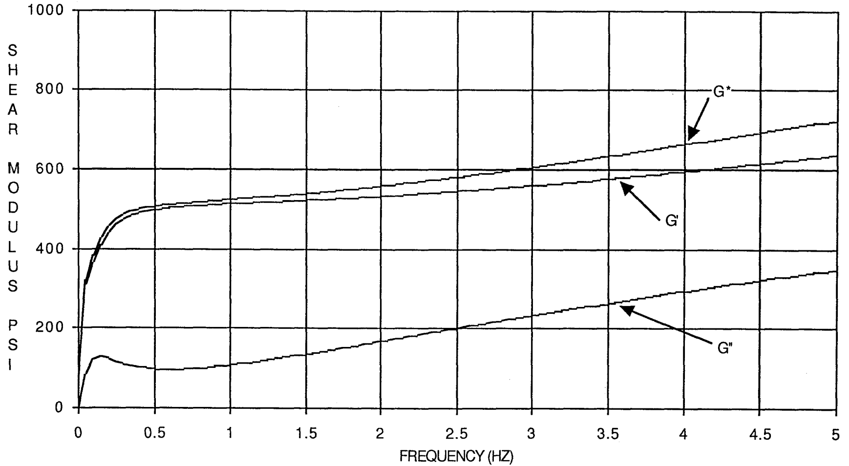
Figure 18. Dynamic shear modulus of TP-H1148 SRM propellant, based on Prony Series fit of stress relaxation data.
