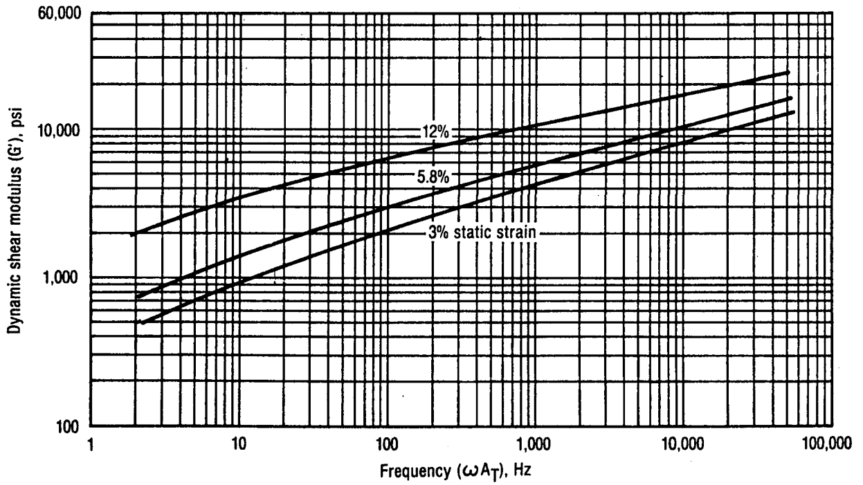
Figure 4. Comparison of static strain levels for batch No. TP-H1148-9.
