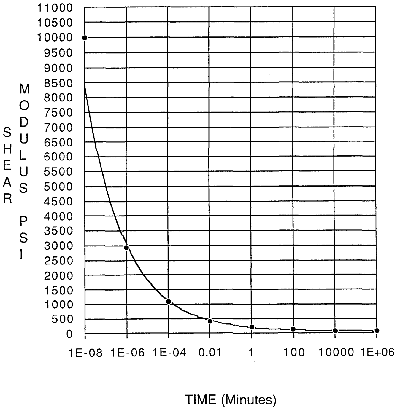
Figure 11. Shear modulus G(t) versus log time, power equation fit.
