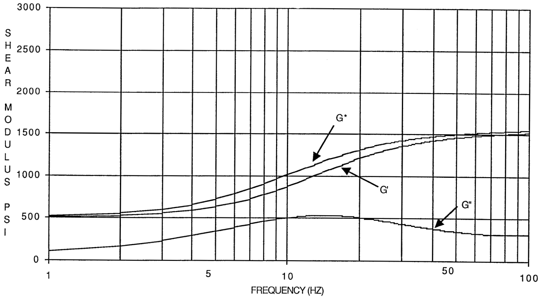
Figure 19. Dynamic shear modulus of TP-H1148 SRM propellant, based on Prony Series fit of stress relaxation data.
