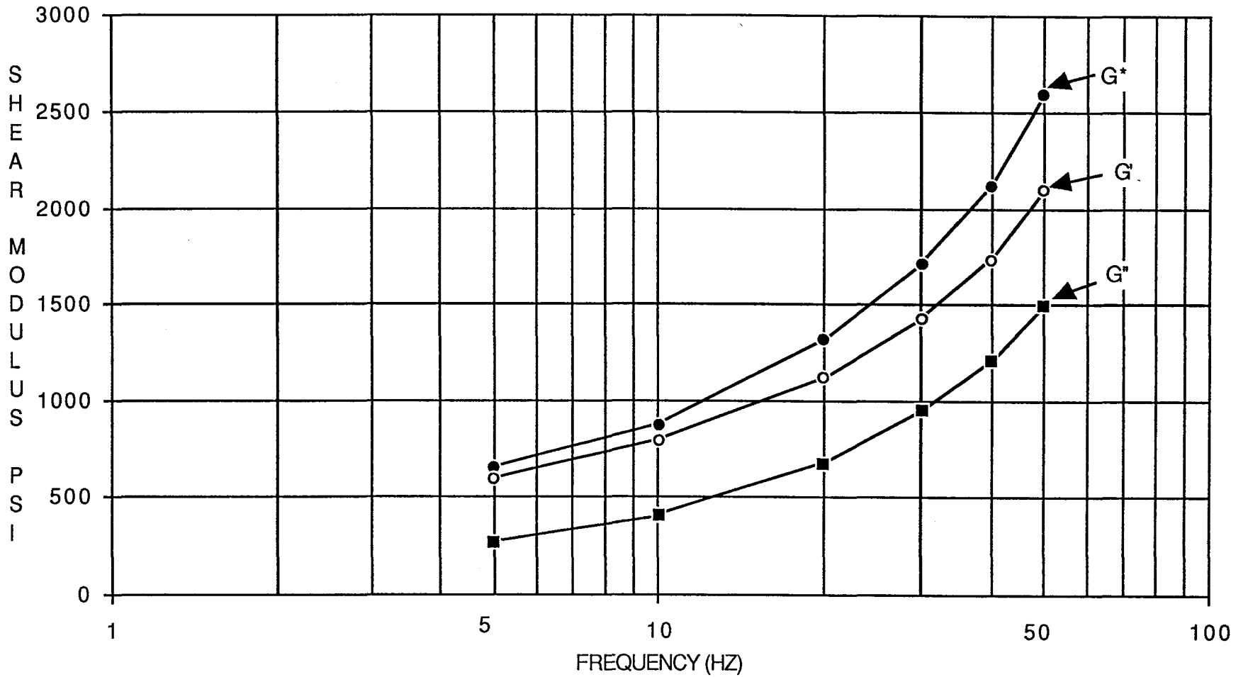
Figure 16. Dynamic shear modulus of TP-H1148 SRM propellant, mix 9910060 at 70°F, sample 36 from TWR-11779.
