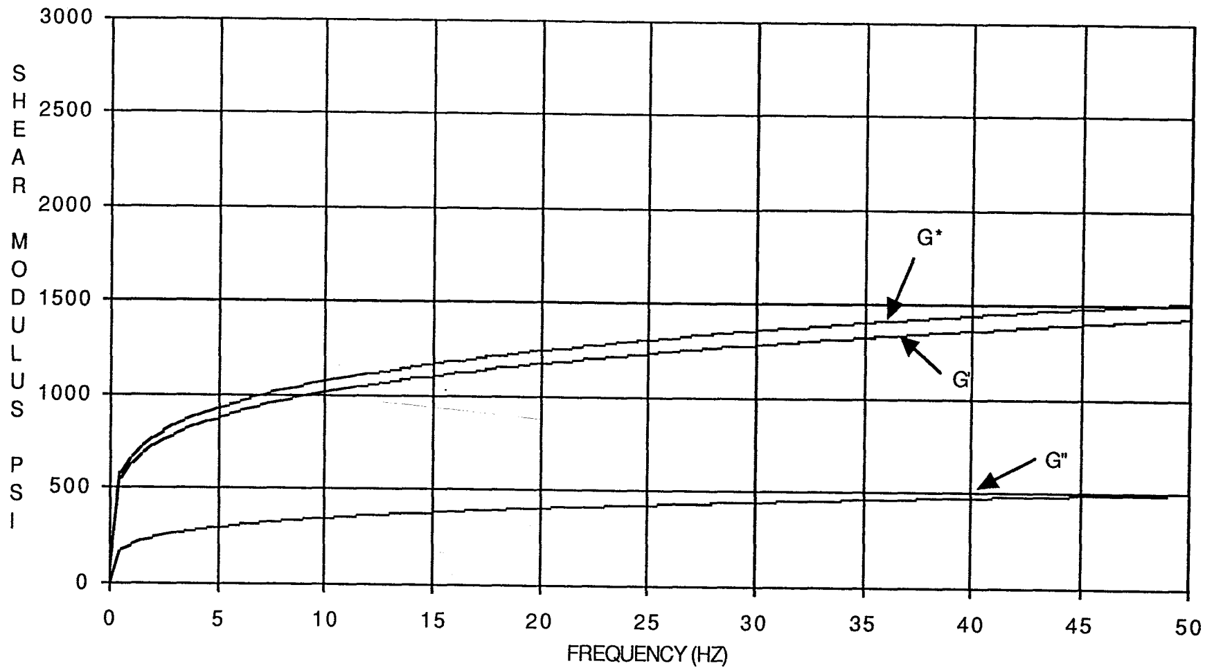
Figure 12. Dynamic shear modulus of TP-H1148 SRM propellant based on power equation fit of stress relaxation data.
