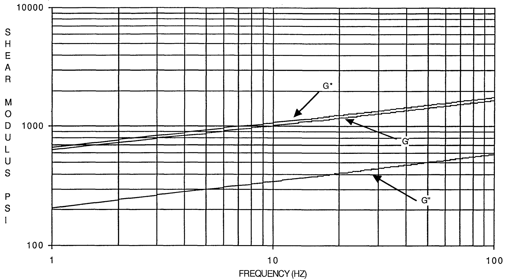
Figure 23. Dynamic shear modulus of TP-H1148 SRM propellant based on power equation fit of stress relaxation data.
