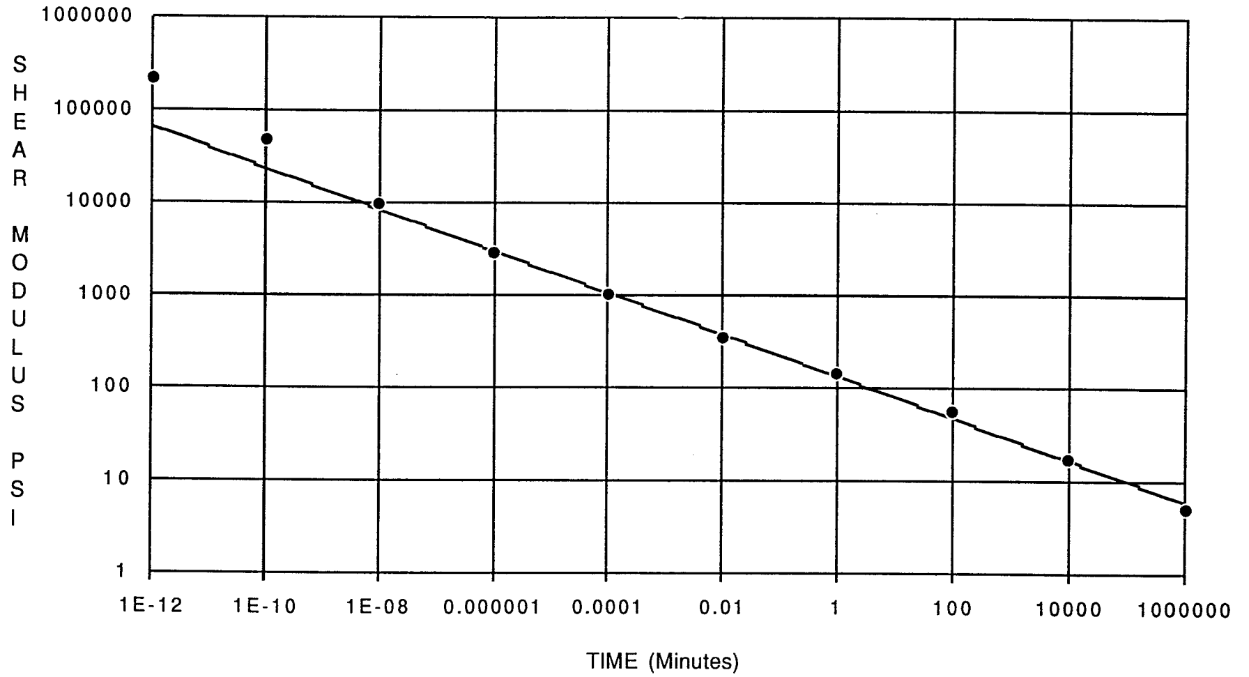
Figure 10. Log shear modulus ( G(t)-75 ) versus log time, power equation fit.
