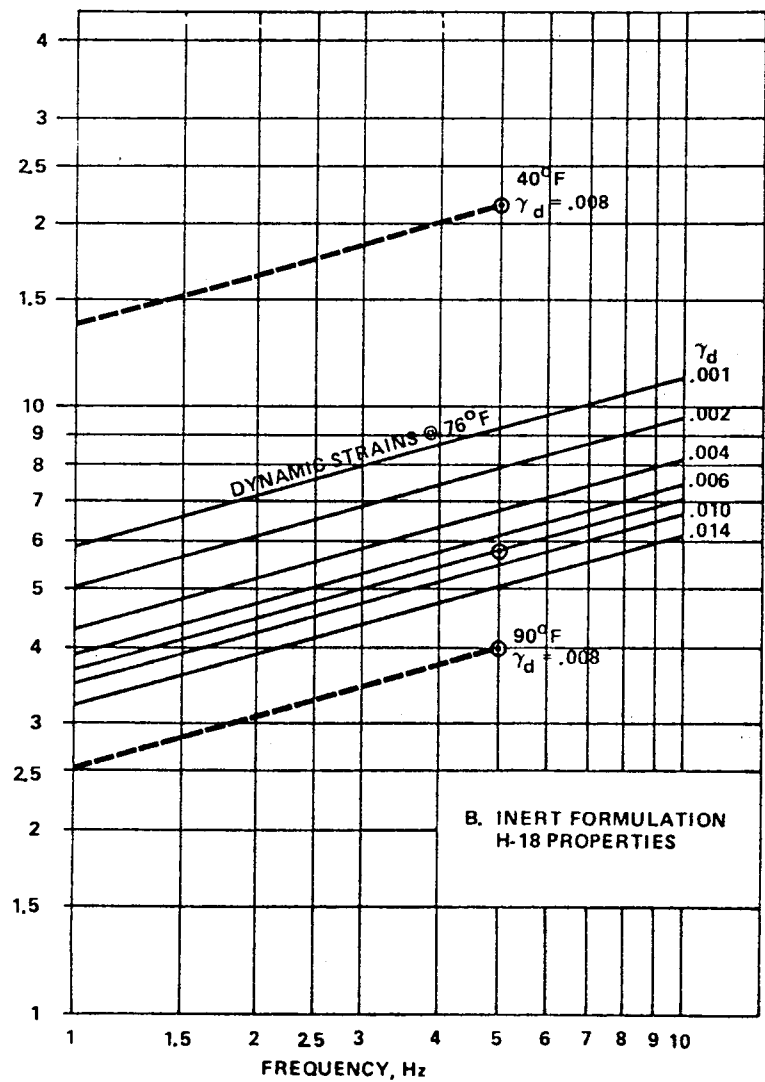
Figure 3. SRB propellant real modulus versus frequency and dynamic strains.
