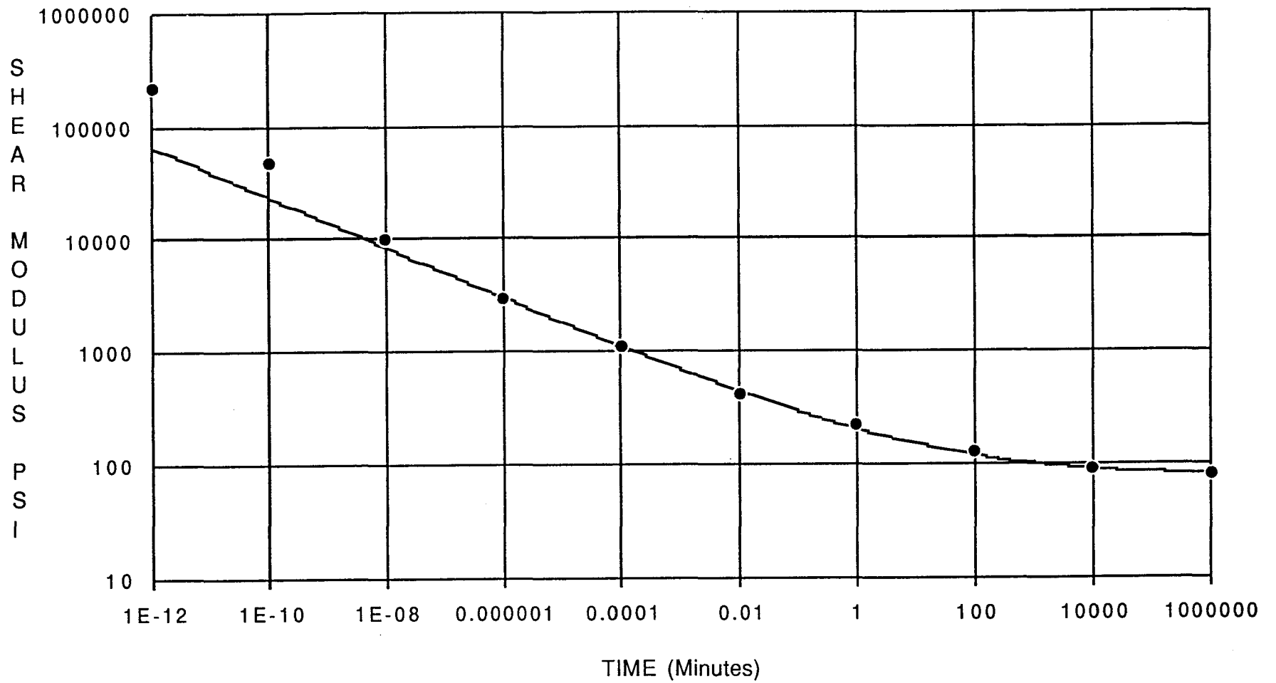
Figure 15. Log shear modulus G(t) versus log time, power equation fit.
