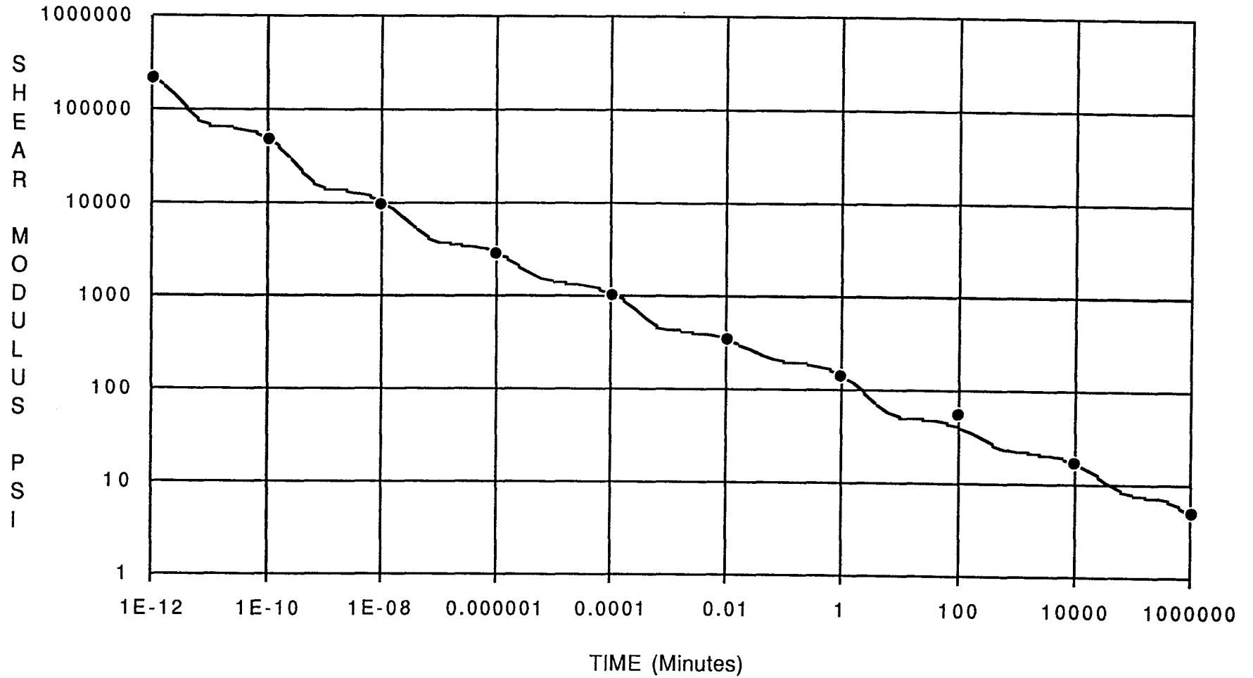
Figure 14. Log shear modulus ( G(t)-75 ) versus log time, Prony Series fit.
