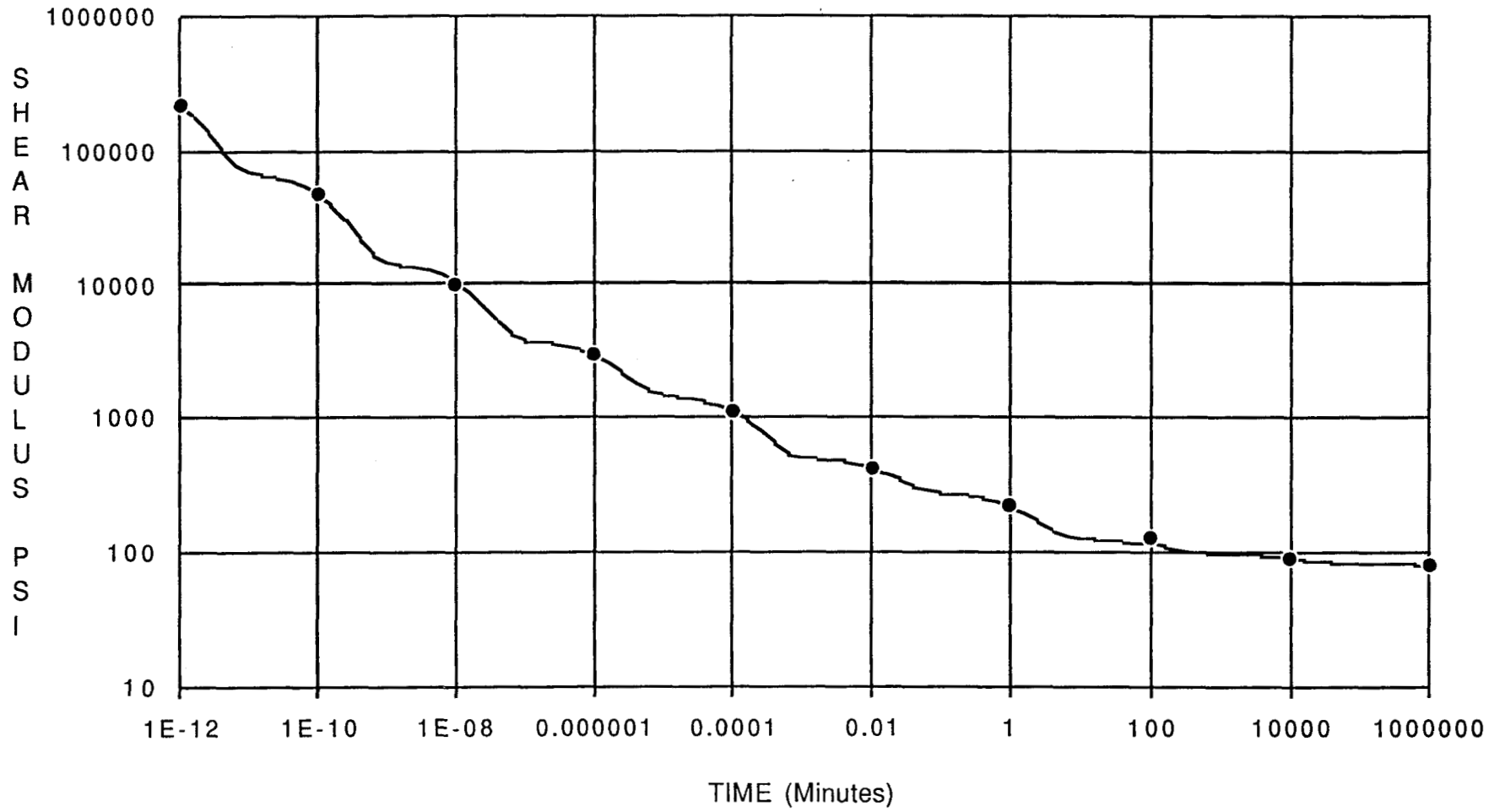
Figure 13. Log shear modulus G(t) versus log time, Prony Series fit.
