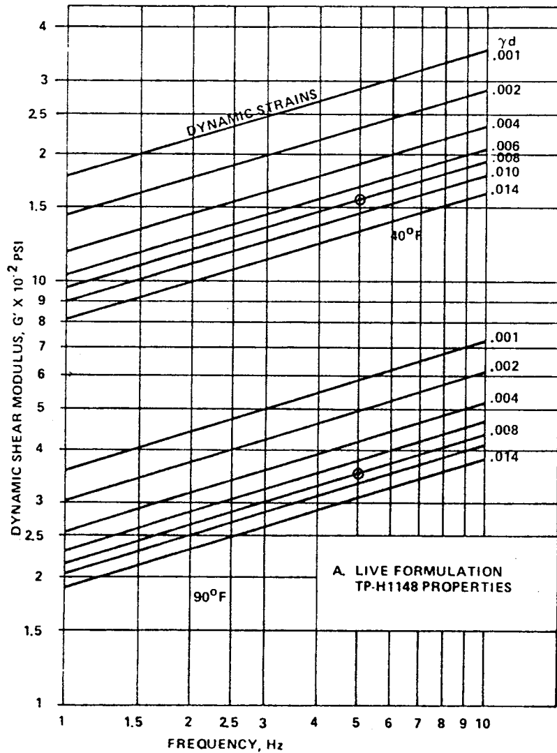
Figure 3. SRB propellant real modulus versus frequency and dynamic strains.
