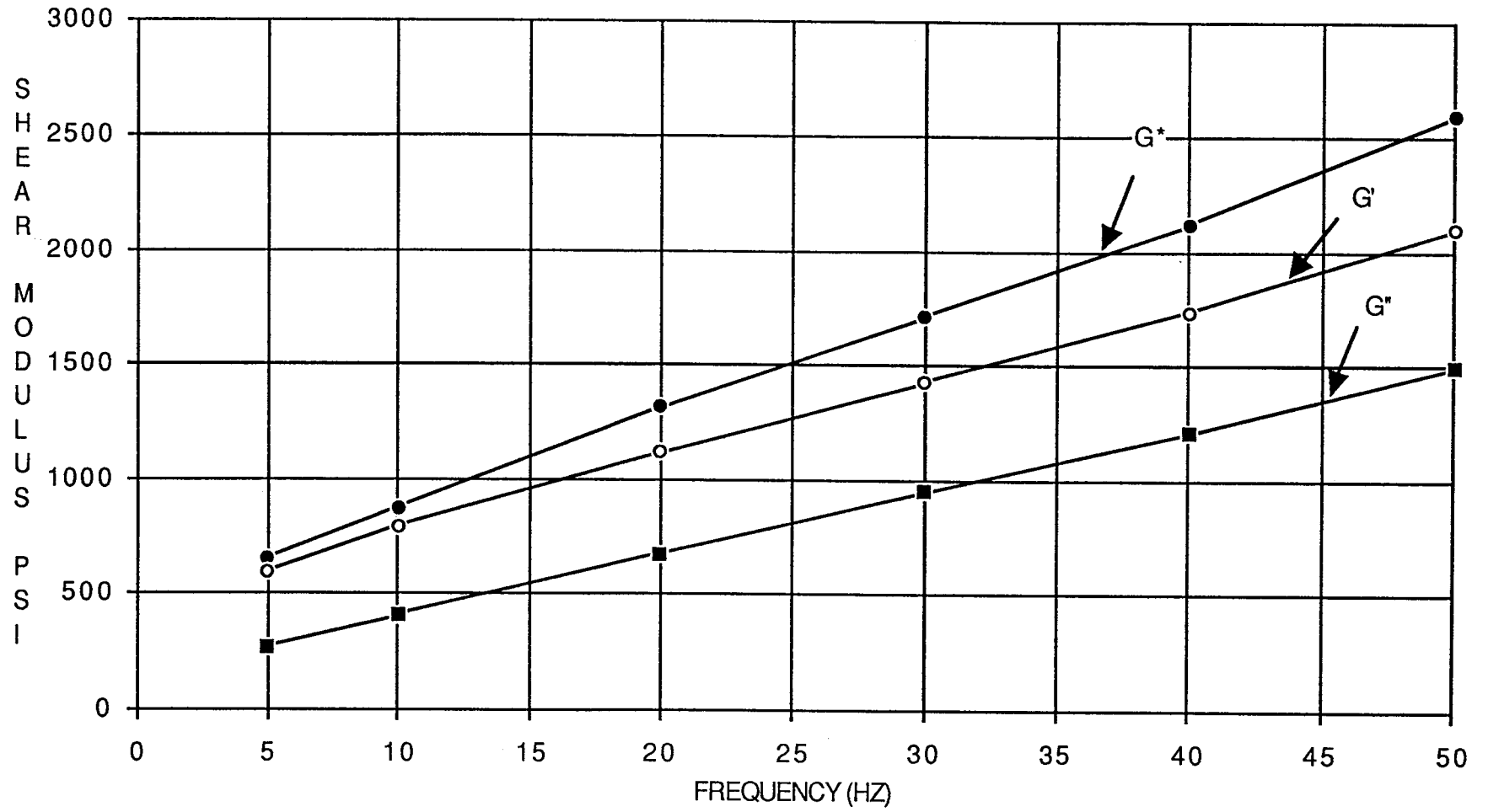
Figure 7. Dynamic shear modulus of TP-H1148 SRM propellant, Mix 9910060 at 70°F, Sample 36 from TWR-11779.
