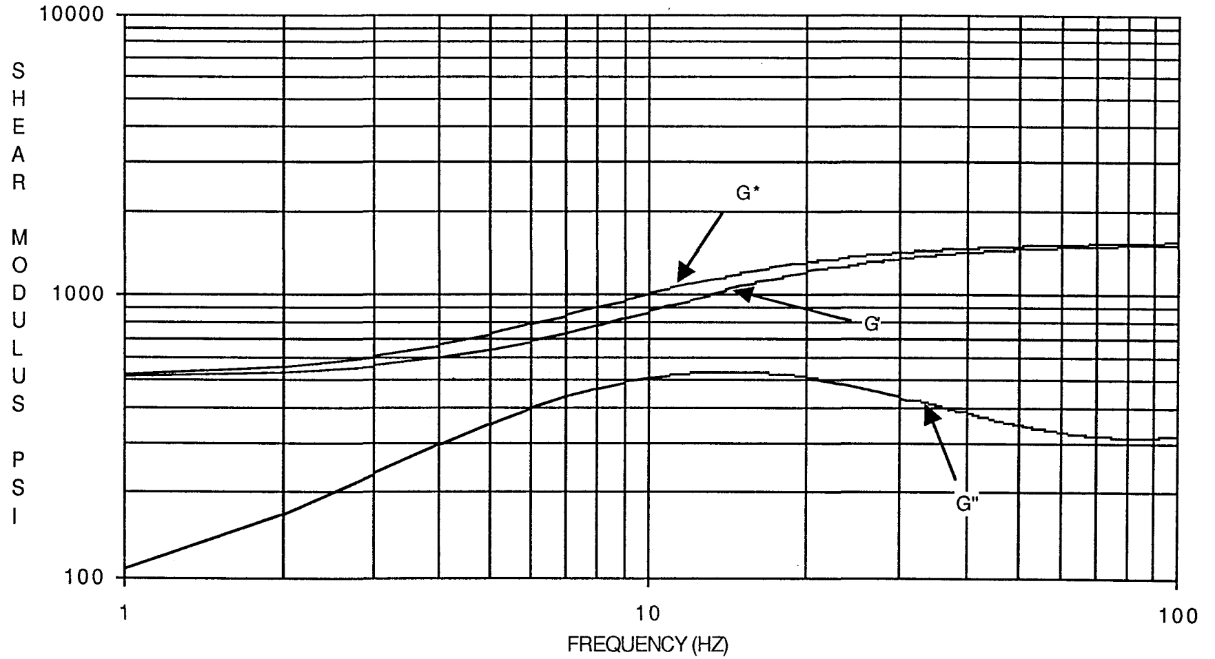
Figure 20. Dynamic shear modulus of TP-H1148 SRM propellant, based on Prony Series fit of stress relaxation data.
