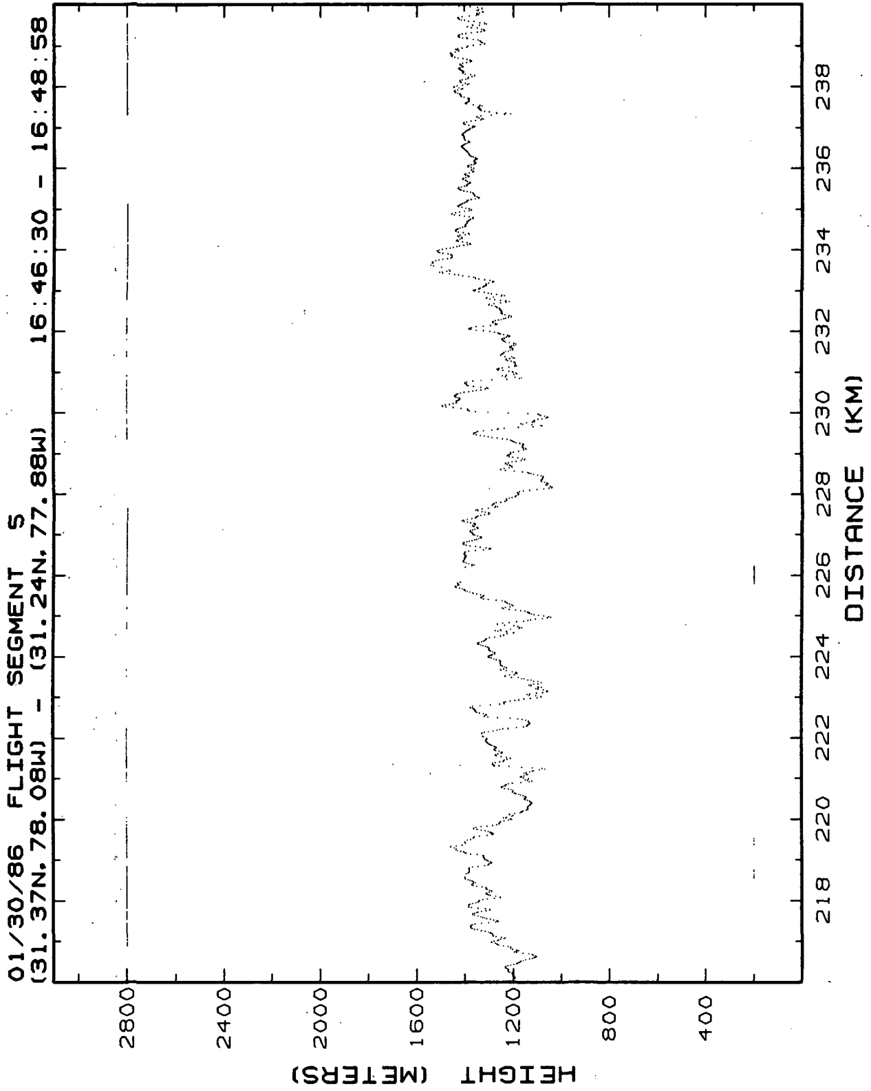
Figure 10.5j. Lidar retrieved MABL heights for Flight 2, 30-Jan-86, flight segment 5, 216-240 km.
