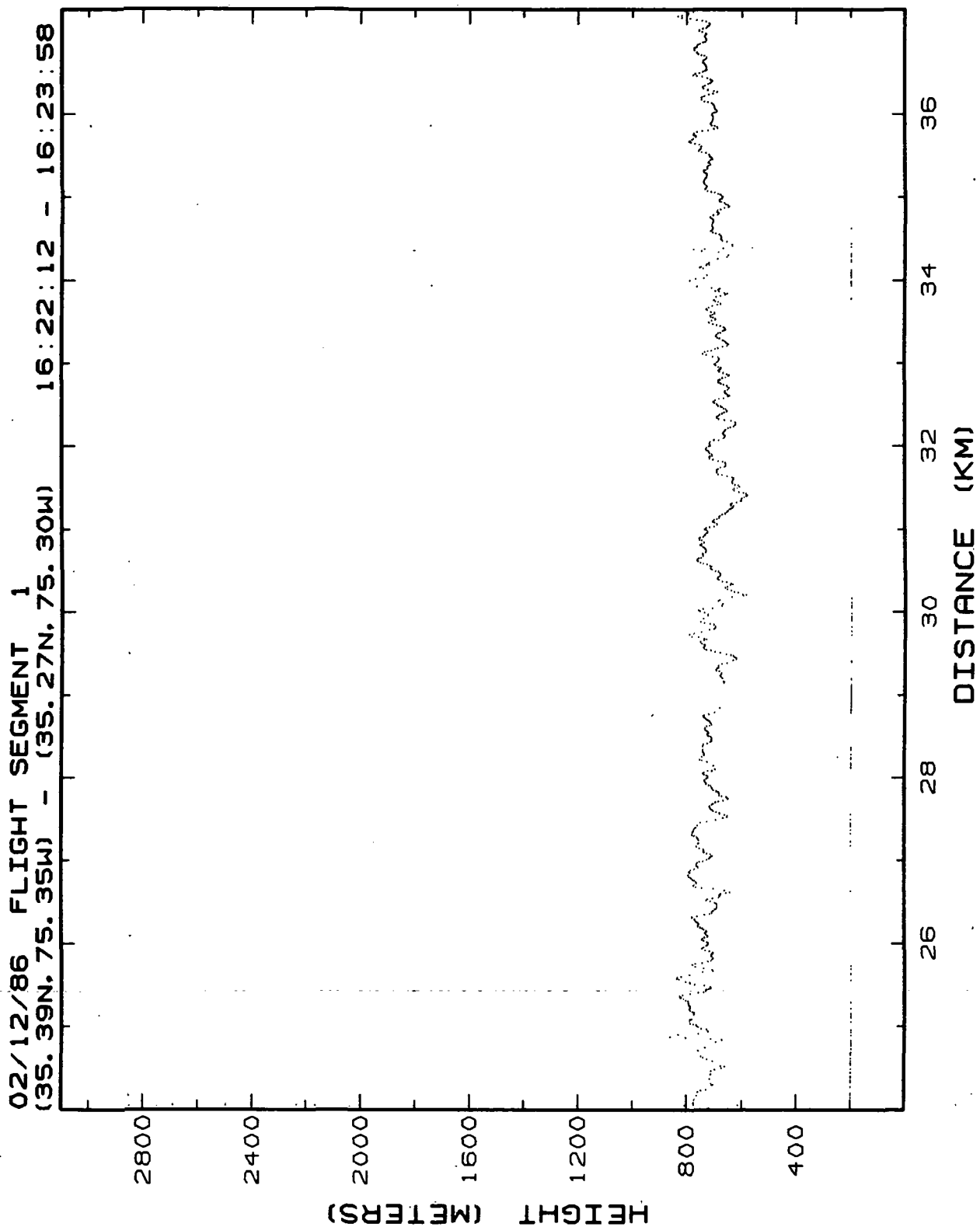
Figure 11.1b: Lidar retrieved MABL heights for Flight 3, 12-Feb-86, flight segment 1, 24-37 km.
