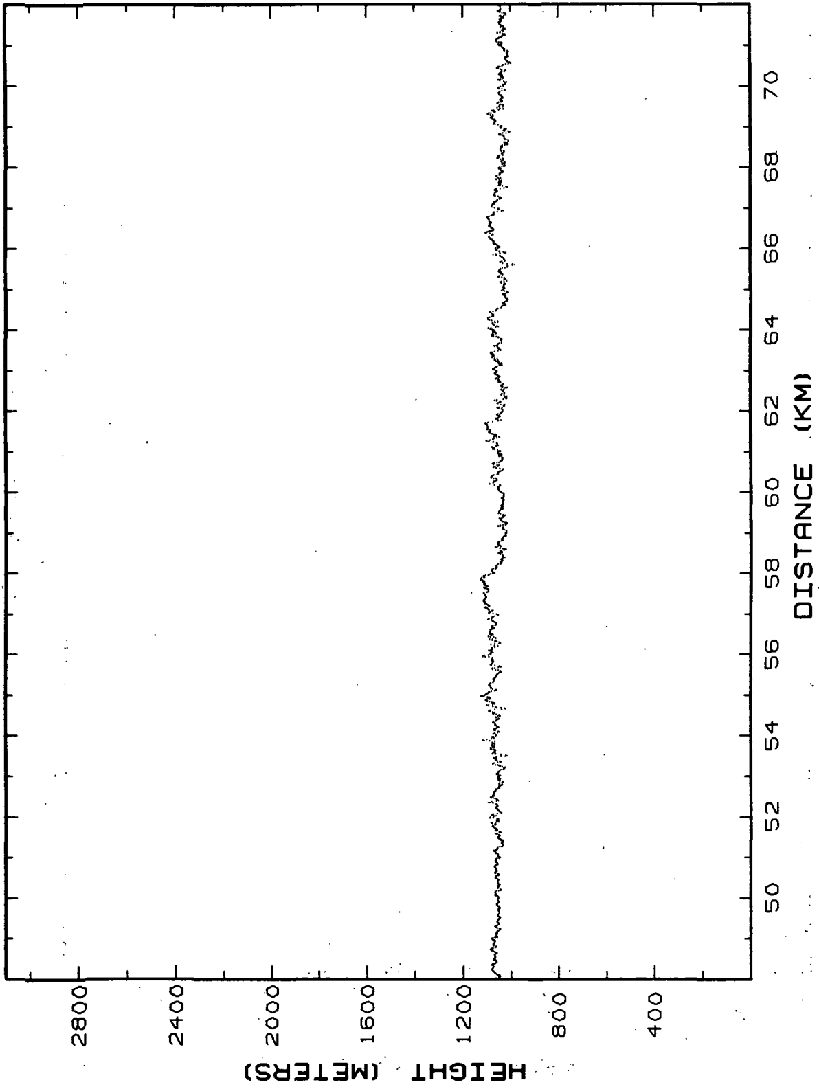
Figure 10.3c. Lidar retrieved MABL heights for Flight 2, 30-Jan-86, flight segment 3, 48-72 km.
