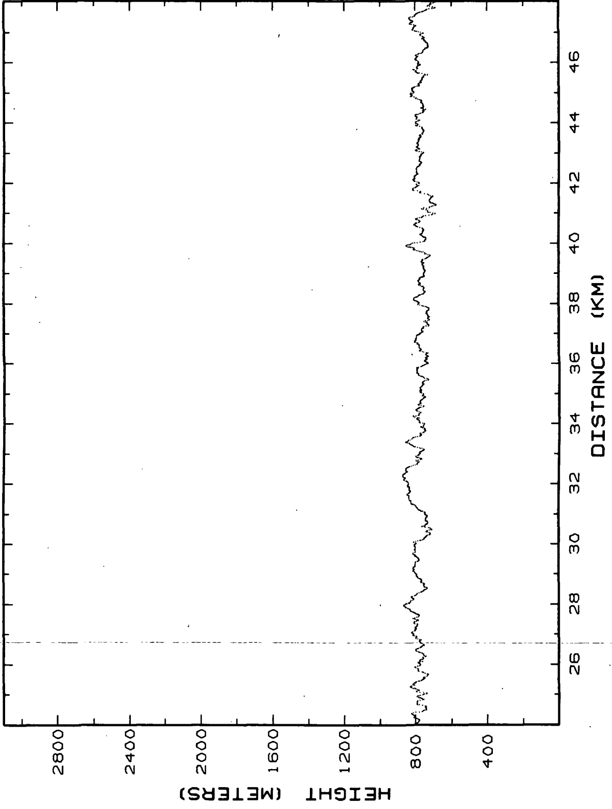
Figure 10.12b. Lidar retrieved MABL heights for Flight 2, 30-Jan-86, flight segment 12, 24-48 km.
