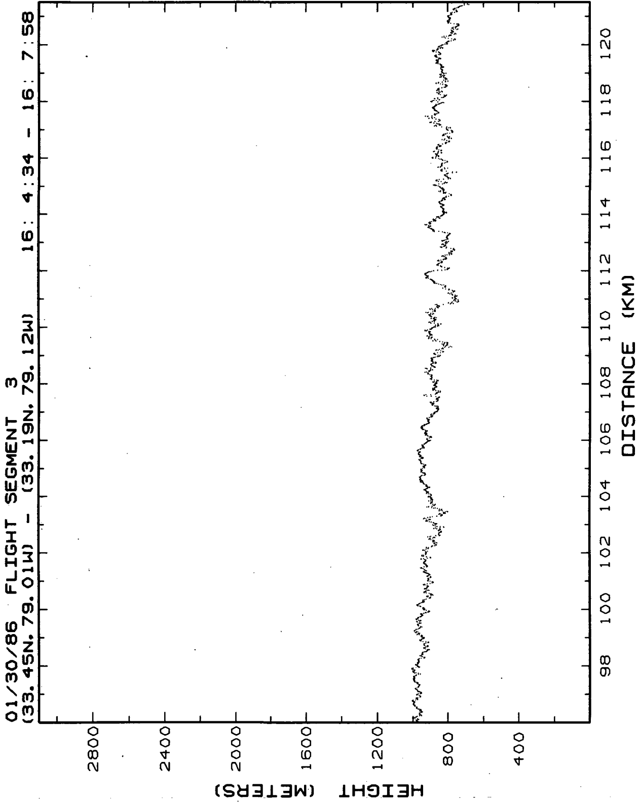
Figure 10.3c. Lidar retrieved MABL heights for Flight 2, 30-Jan-86, flight segment 3, 96-120 km.
