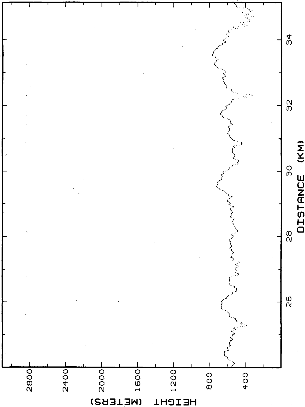
Figure 12.10b. Lidar retrieved MABL heights for Flight 4, 02-Mar-86, flight segment 11, 24-35 km.
