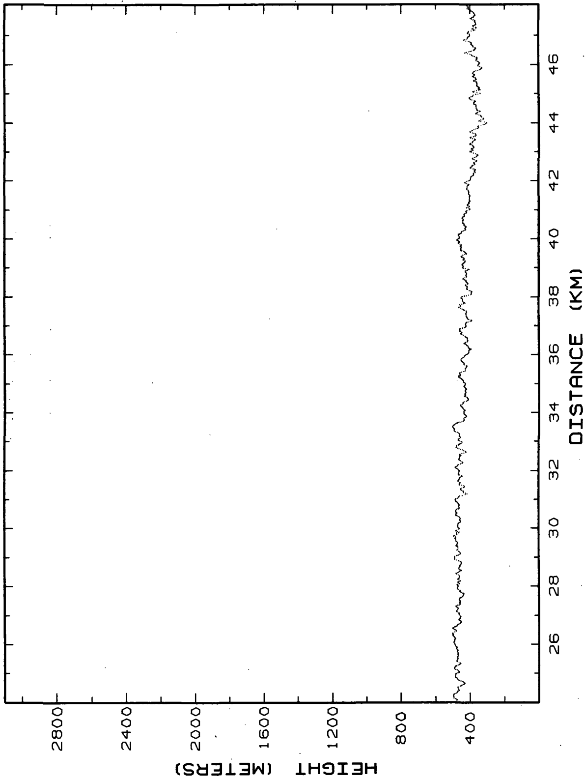
Figure 12.2b. Lidar retrieved MABL heights for Flight 4, 02-Mar-86, flight segment 2, 24-48 km.
