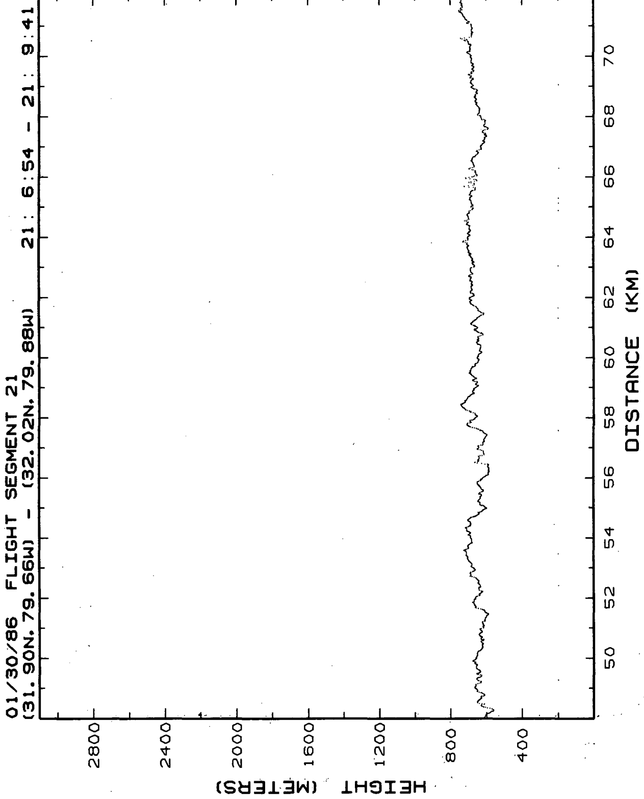
Figure 10.21c. Lidar retrieved MABL heights for Flight 2, 30-Jan-86, flight segment 21, 48-72 km.
