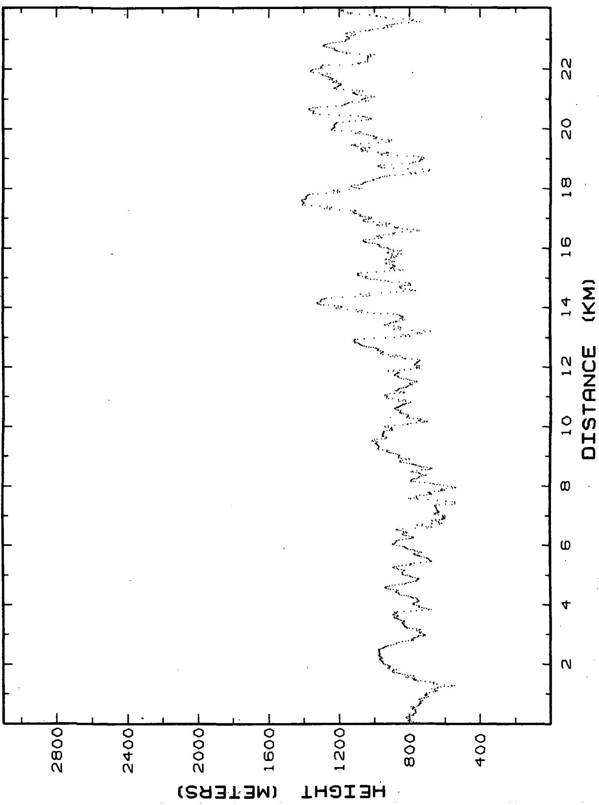
Figure 12.5a. Lidar retrieved MABL heights for Flight 4, 02-Mar-86, flight segment 5, 0-24 km.
