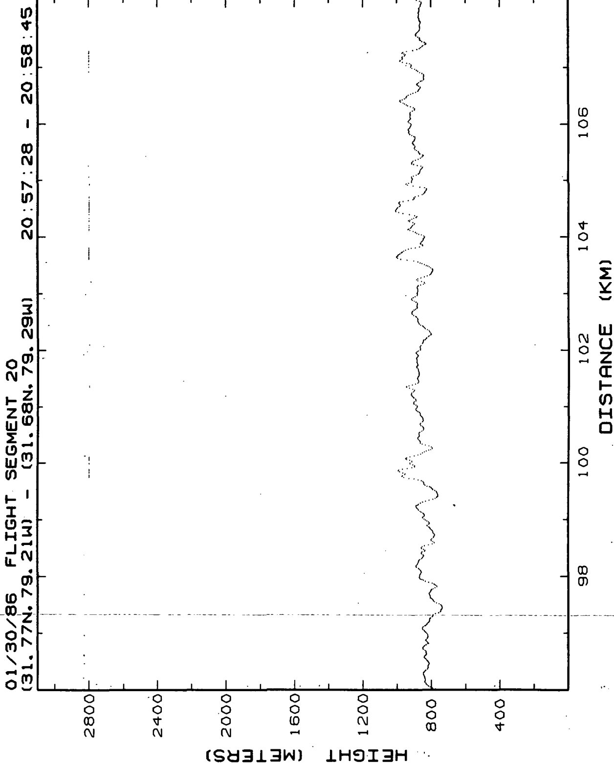
Figure 10.20e. Lidar retrieved MABL heights for Flight 2, 30-Jan-86, flight segment 20, 96-108 km.
