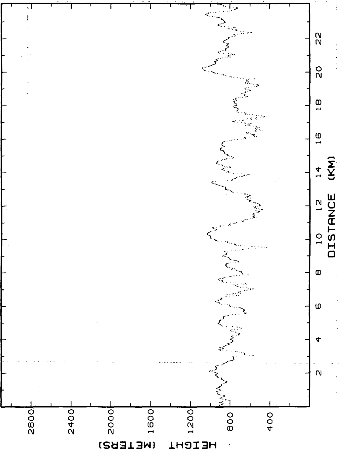
Figure 12.14a. Lidar retrieved MABL heights for Flight 4, 02-Mar-86, flight segment 16, 0-24 km.
