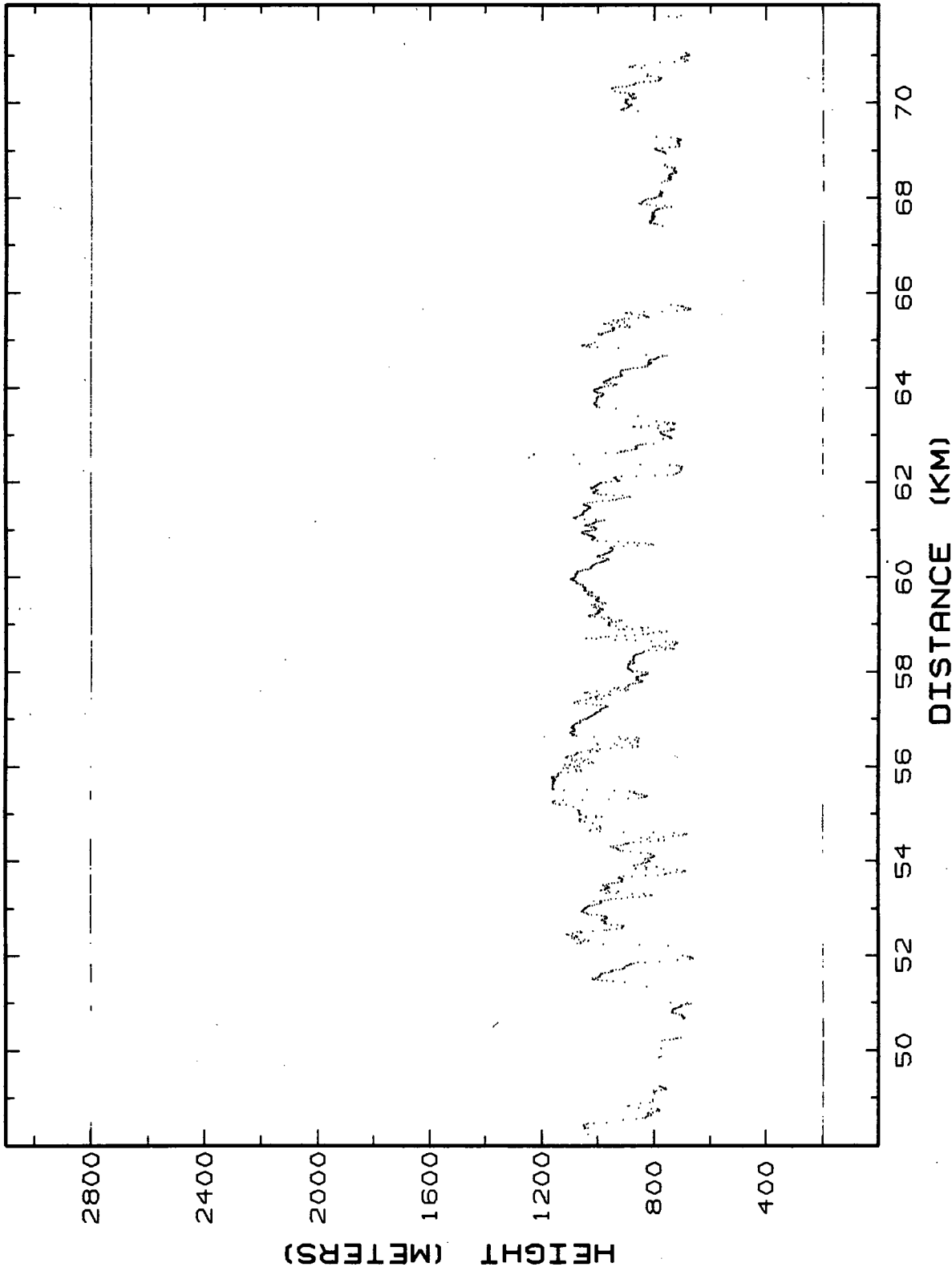
Figure 11.2c. Lidar retrieved MABL heights for Flight 3, 12-Feb-86, flight segment 2, 48-72 km.
