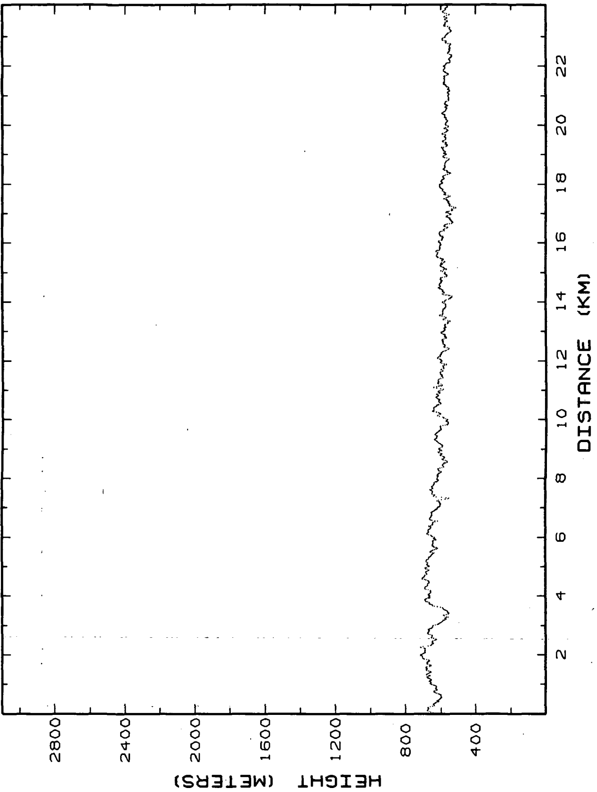
Figure 12.1a. Lidar retrieved MABL heights for Flight 4, 02-Mar-86, flight segment 1, 0-24 km.
