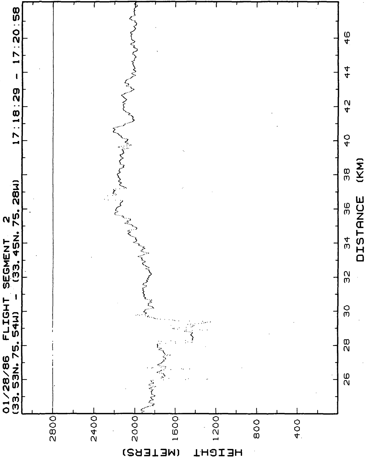
Figure 9.2b. Lidar retrieved MABL heights for Flight 1, 28-Jan-86, flight segment 2, 24-48 km.
