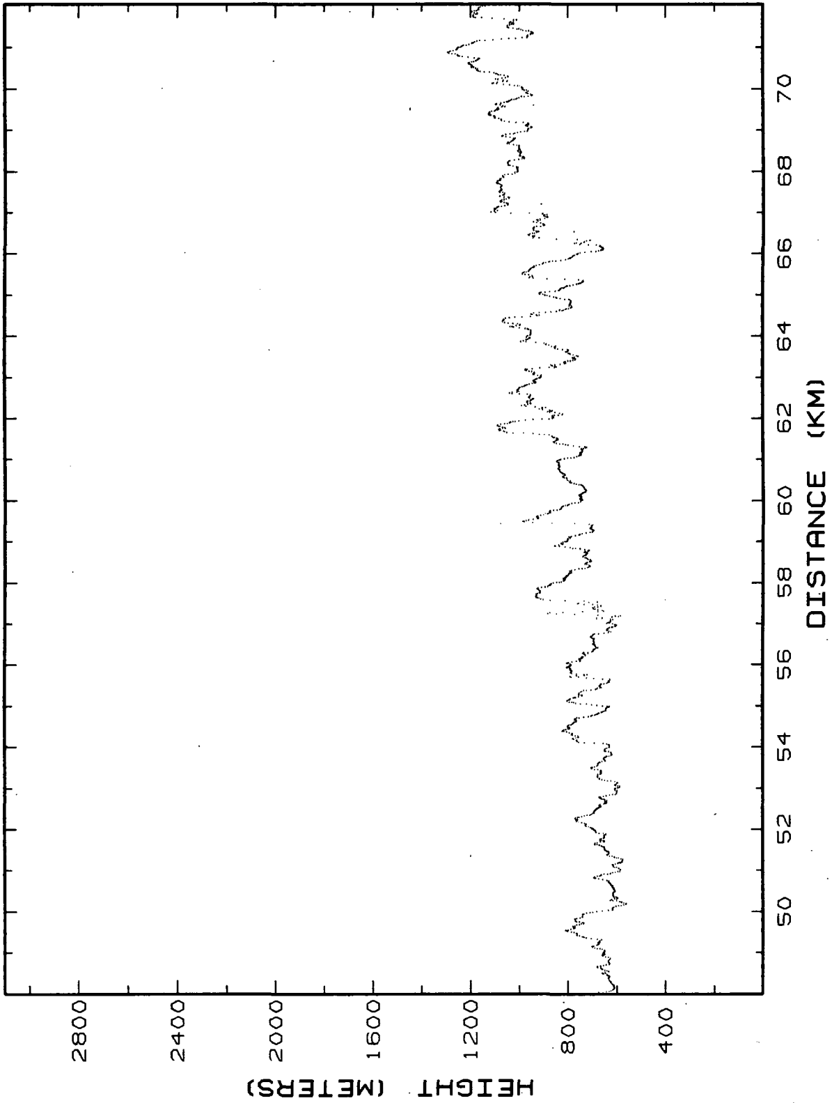
Figure 12.4c. Lidar retrieved MABL heights for Flight 4, 02-Mar-86, flight segment 4, 48-72 km.
