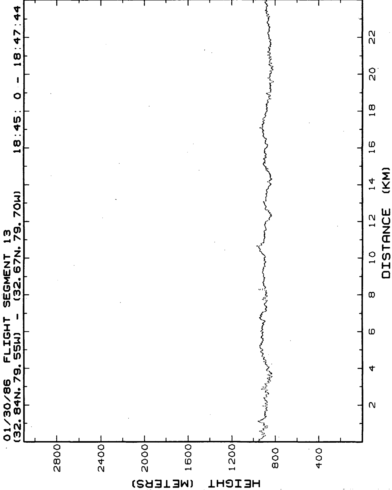
Figure 10.13a. Lidar retrieved MABL heights for Flight 2, 30-Jan-86, flight segment 13, 0-24 km.
