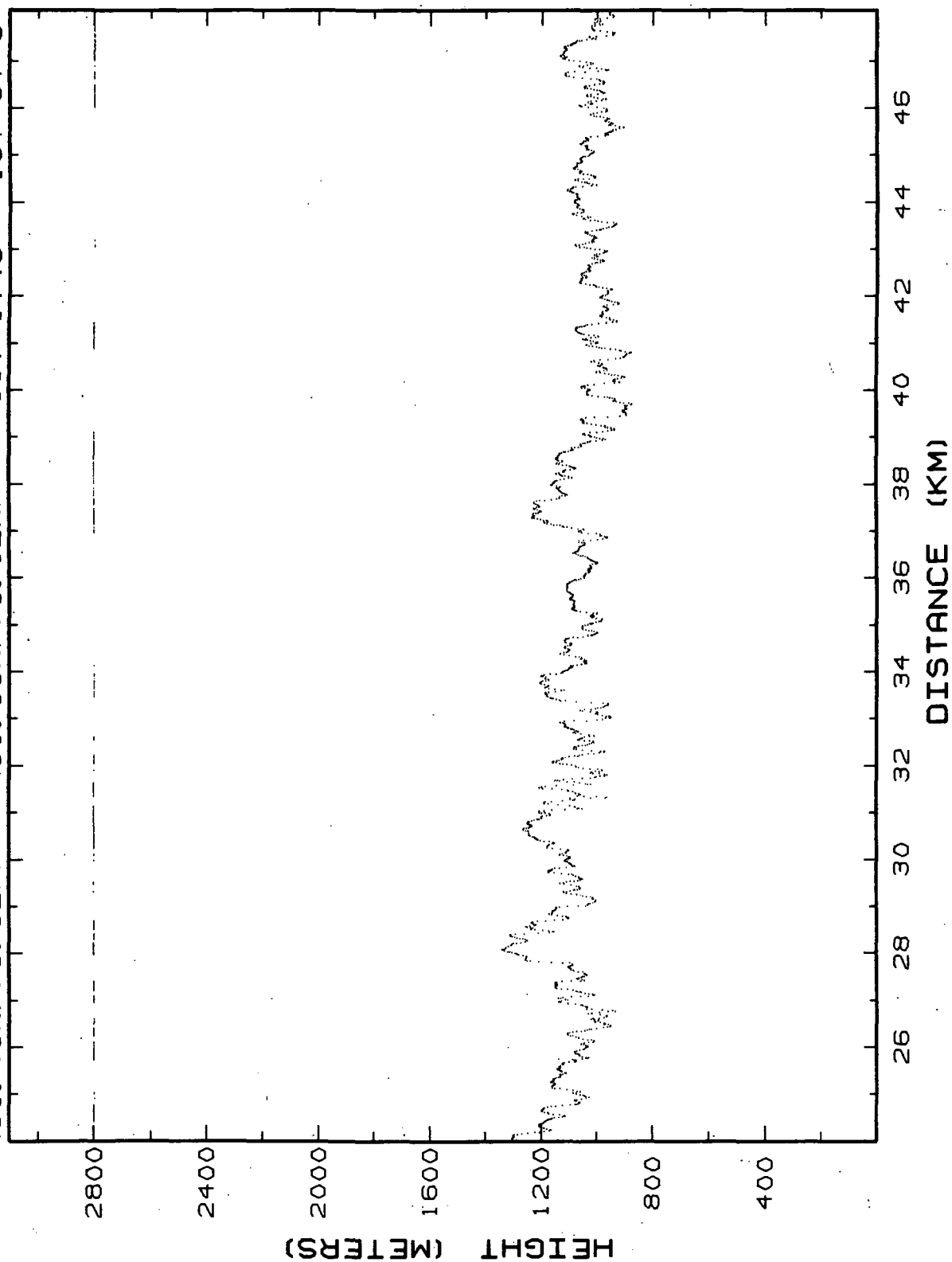
Figure 10.10b. Lidar retrieved MABL heights for Flight 2, 30-Jan-86, flight segment 10, 24-48 km.
