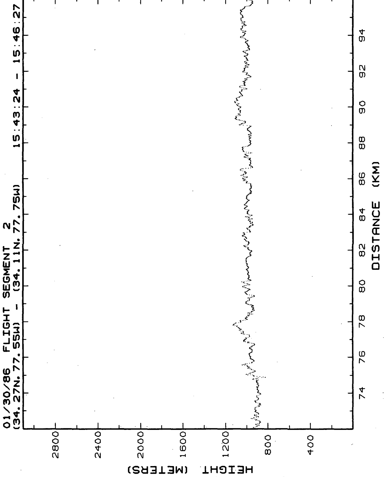
Figure 10.2d. Lidar retrieved MABL heights for Flight 2, 30-Jan-86, flight segment 2, 72-96 km.
