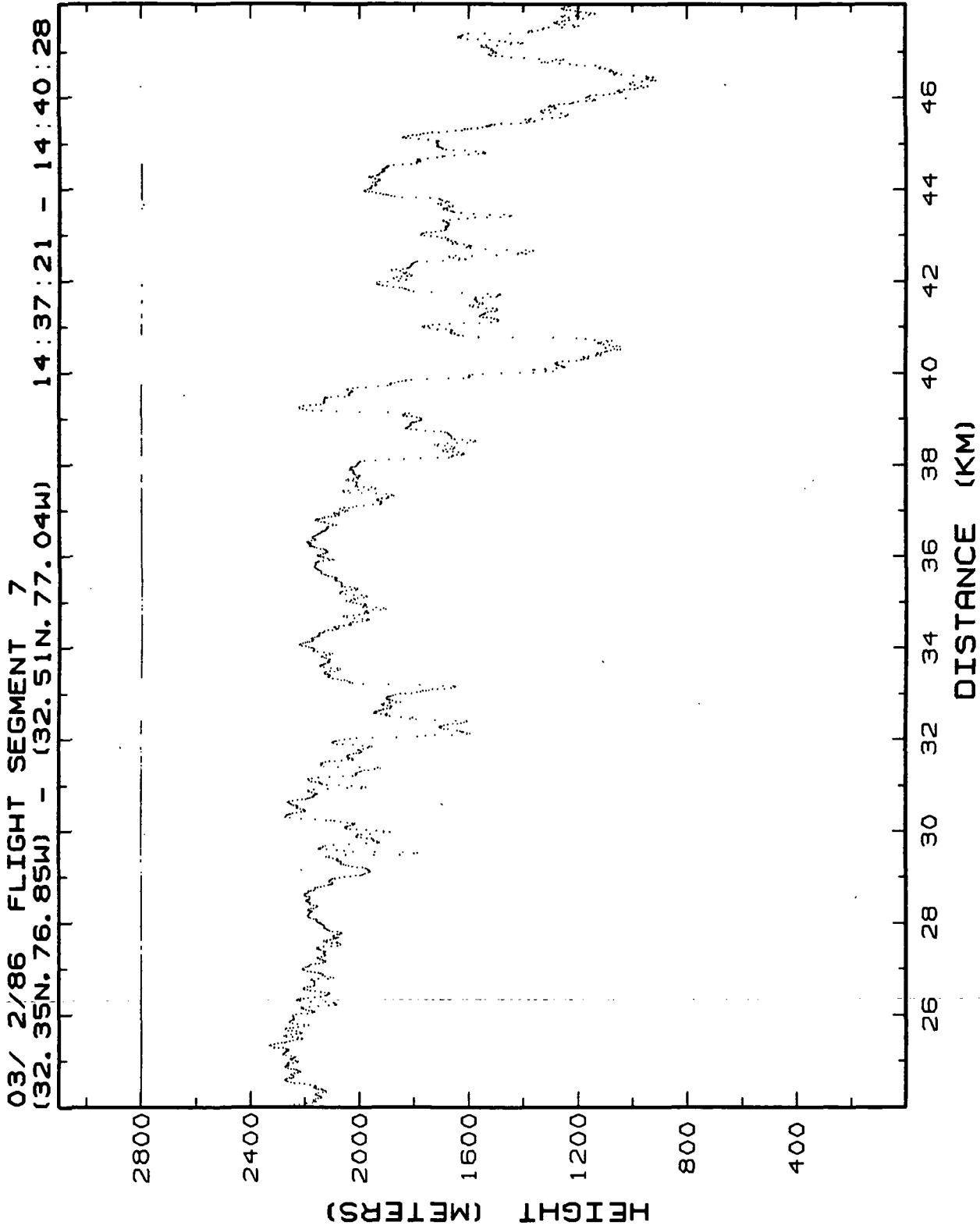
Figure 12.7b. Lidar retrieved MABL heights for Flight 4, 02-Mar-86, flight segment 7, 24-43 km.
