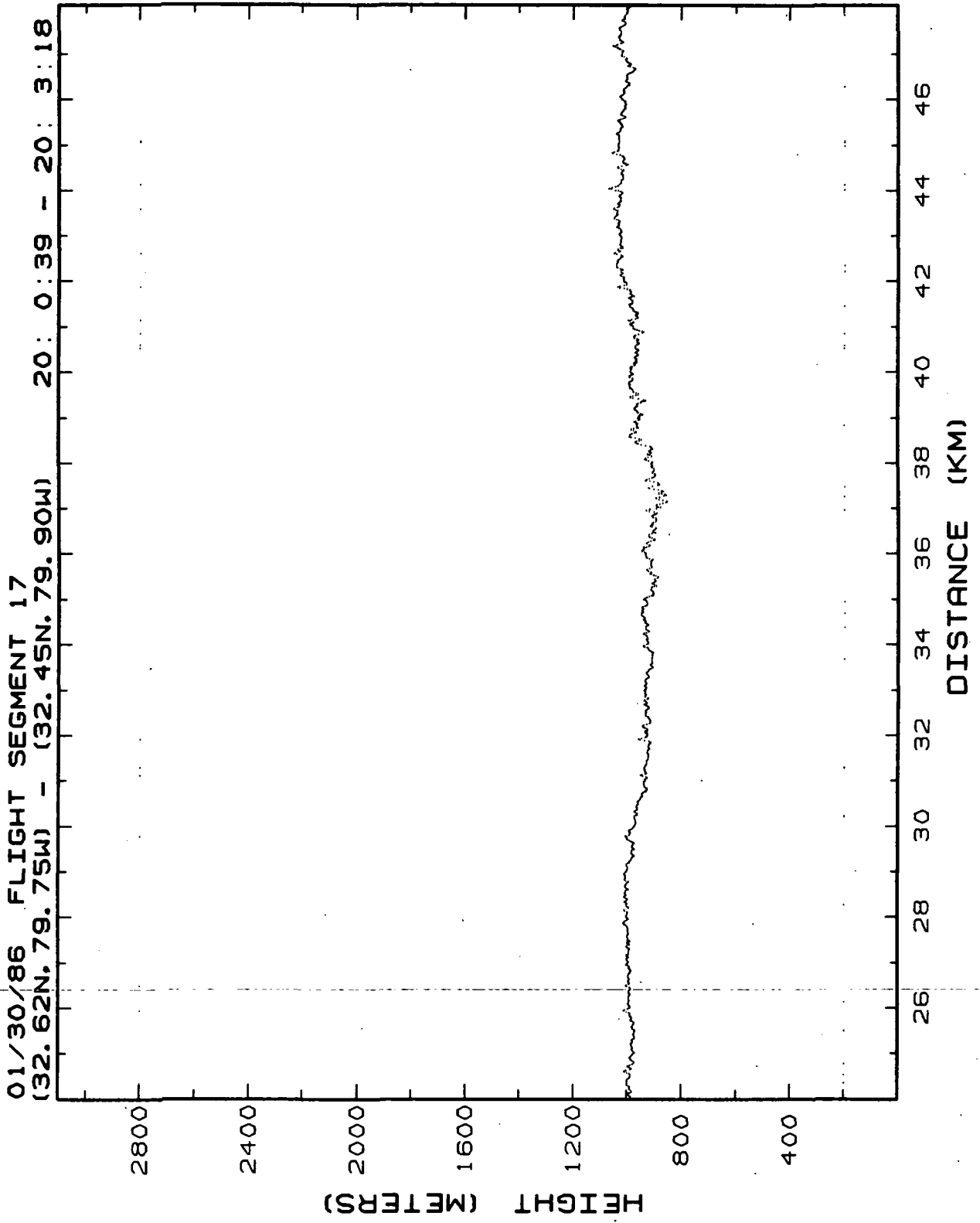
Figure 10.17b. Lidar retrieved MABL heights for Flight 2, 30-Jan-86, flight segment 17, 24-48 km.
