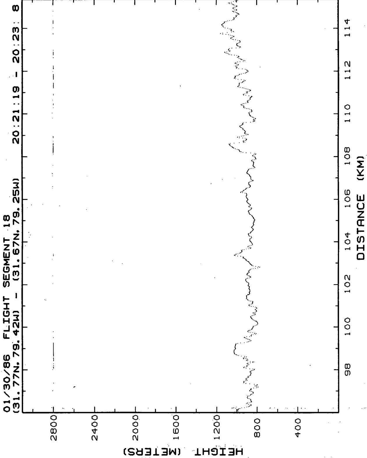
Figure 10.18e. Lidar retrieved MABL heights for Flight 2, 30-Jan-86, flight segment 18, 96-115 km.
