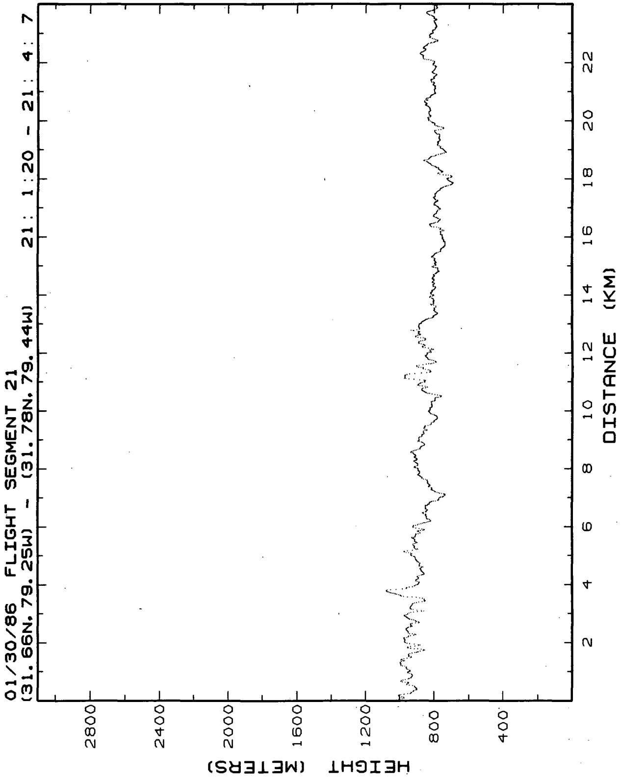
Figure 10.21a. Lidar retrieved MABL heights for Flight 2, 30-Jan-86, flight segment 21, 0-24 km.
