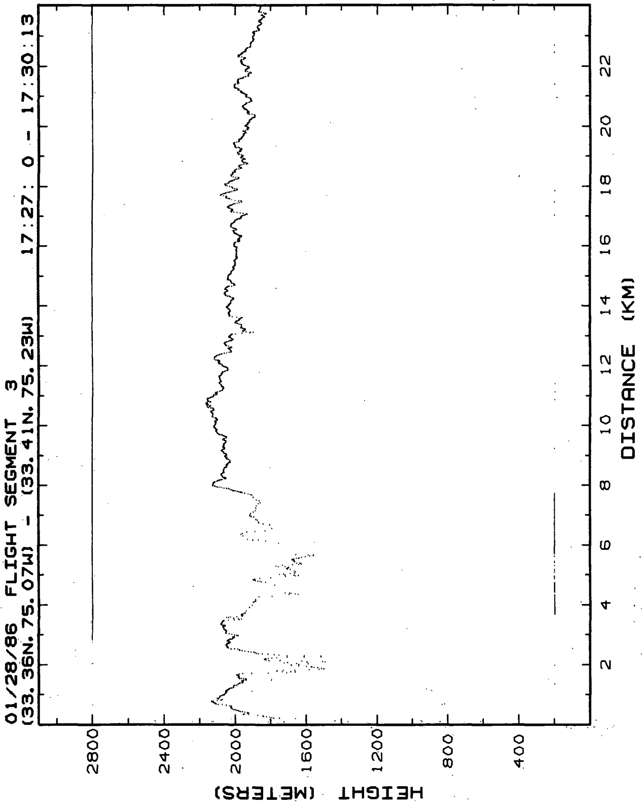
Figure 9.3. Lidar retrieved MABL heights for Flight 1, 28-Jan-86, flight segment 3, 0-24 km.
