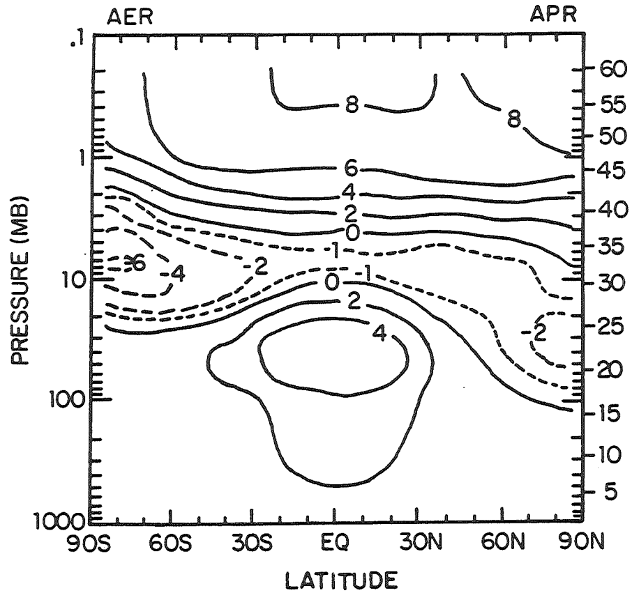
D-1a. Ozone profile changes (%) from JPL-85 to JPL-87 chemical models with the AER model for the months of January and April.
