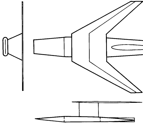
(b) FLAT BODY WITH SWEPT PARASOL WING
